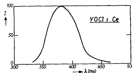
FIG. 8. Spectral energy distribution of the fluorescence of Y 0.99 Ce 0.01 OCl under 254-m \mu excitation.
