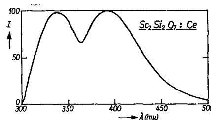
FIG. 7. Spectral energy distribution of the fluorescence of Sc 1.98 Ce 0.02 Si 2 O 7 under 254-m \mu excitation.
