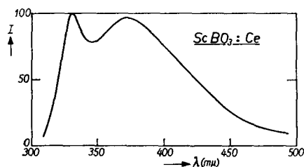
FIG. 6. Spectral energy distribution of the fluorescence of Sc 0.99 Ce 0.01 BO 3 under 254-m \mu excitation.
