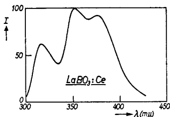
Fig. 4. Spectral energy distribution of the fluorescence of La 0.99 Ce 0.01 BO 3 under 254-m \mu excitation. In Figs. 5-12 the radiant power per constant wavelength interval in arbitrary units ( I ) is plotted along the ordinate.
