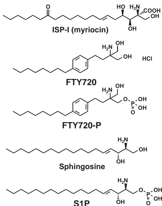
Fig. 1. The chemical structures of ISP-I, FTY720, FTY720-P, sphingosine,
