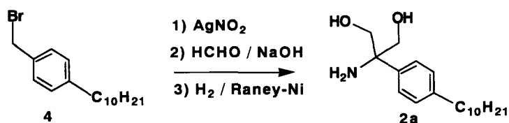
Scheme 2. Synthesis of 2a.
