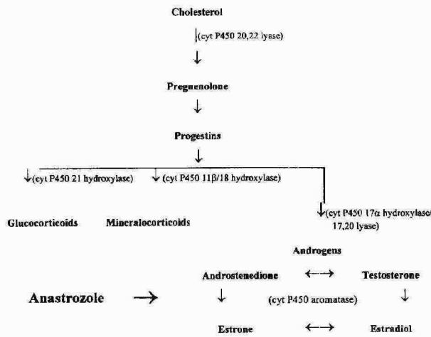
Figure 1. Estrogen synthesis (16).
