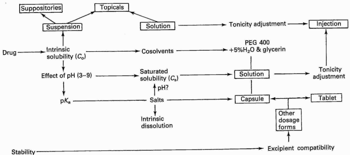
Fig. 13.8 A generic development pathway: the relationship between preformulation and formulation in dosage form development. The formulation stages are shown in boxes and the performance stages are unboxed
