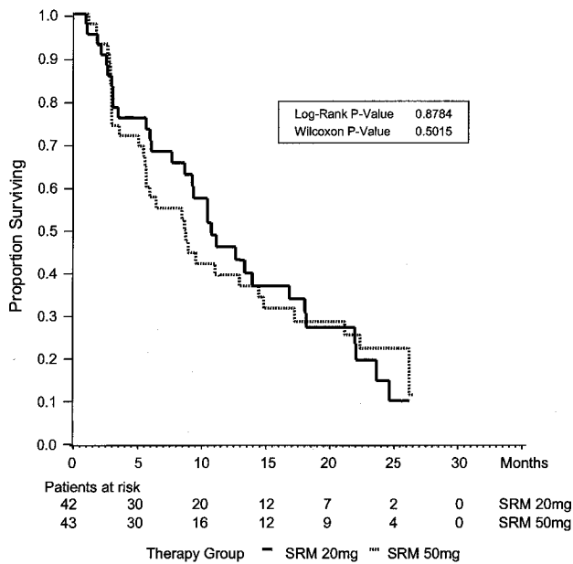
Figure 2. Time to progression.
