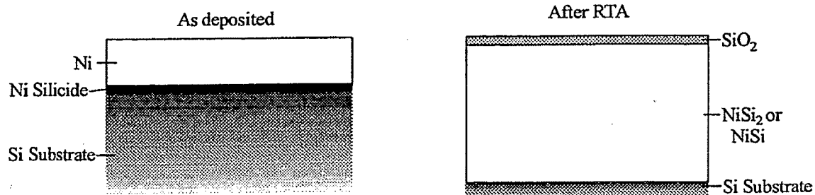
Figure 5.11. Schematic of the structure of the studied Ni-Si films.
