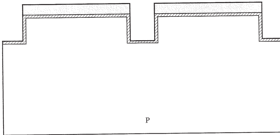
Figure 2-7 A thin “liner” oxide is thermally grown in the trenches. The nitride prevents any additional oxidation on the top surface of the wafer.
