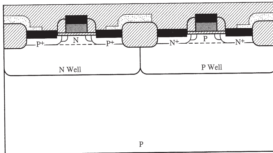
Figure 2-39 Chemical-Mechanical Polishing (CMP) or resist etchback is used to polish or etchback the deposited SiO 2 layer. This planarizes the wafer surface.
