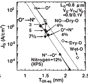
Fig. 7 Gate leakage current vs. T_{OX-eq} of SiON and SiO 2 using radical processes and using conventional thermal processes (Dry-O, Wet-O and NO→Dry-O).
