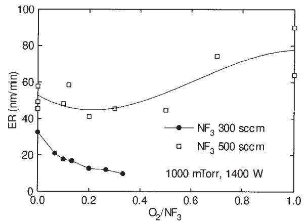
FIG. 4. The etch rate of silicon dioxide as a function of the flow ratio \text{O}_2/\text{NF}_3 . The etch rate decreases as oxygen is added to a flow of 300 sccm of \text{NF}_3 . If a higher \text{NF}_3 flow is used (500 sccm), the etch rate remains on a constant level up to a ratio of 0.4, and then increases slightly upon further increase of the flow ratio.
