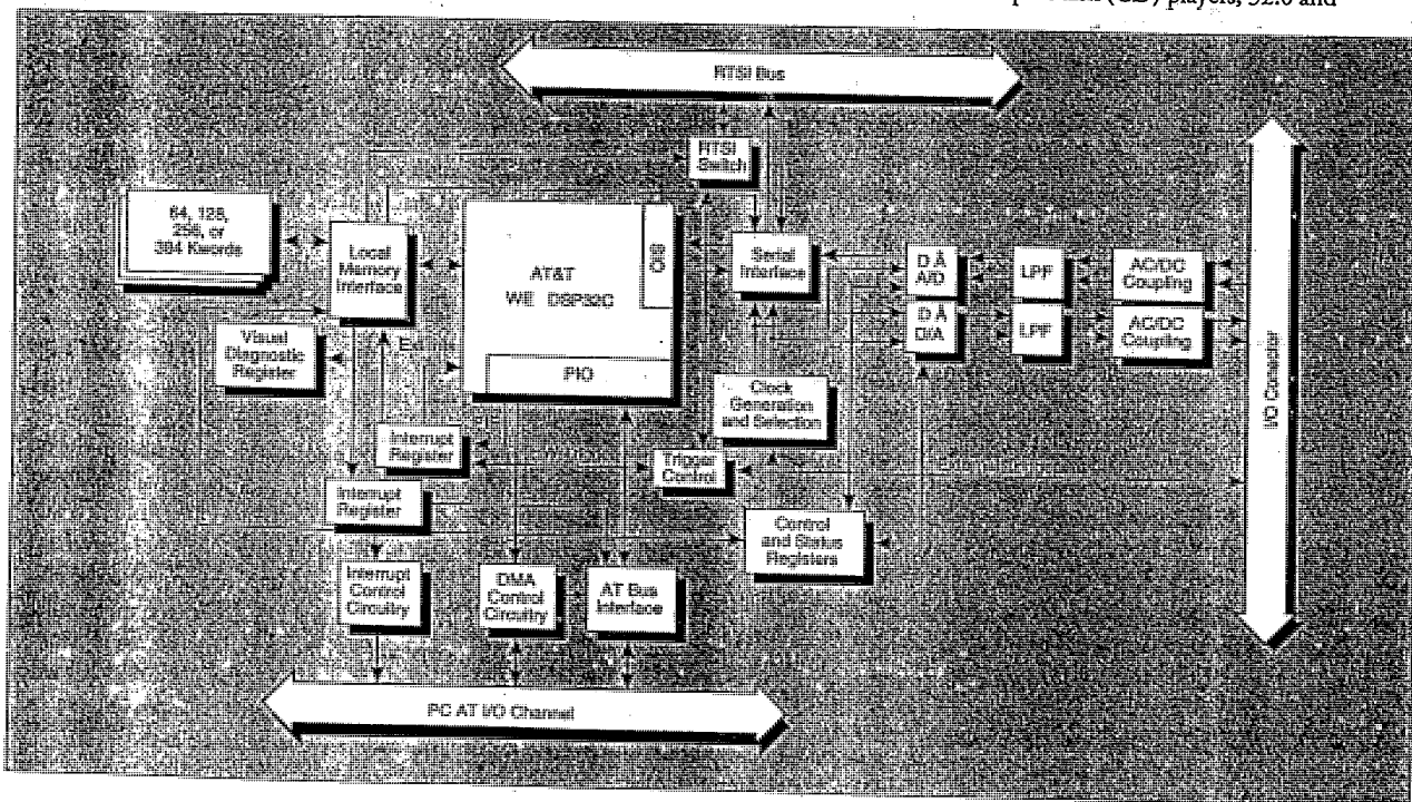
Figure 1. AT-DSP2200 Block Diagram
