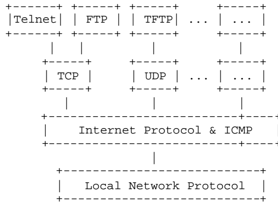
Protocol Relationships
