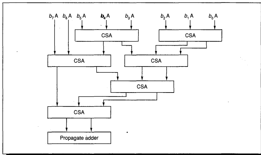
FIGURE A.25 Wallace-tree multiplier.
