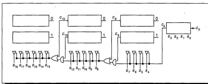
FIGURE A.17 Carry-select adder. As soon as the carry out of the rightmost block is known, it is used to select the other sum bits.
