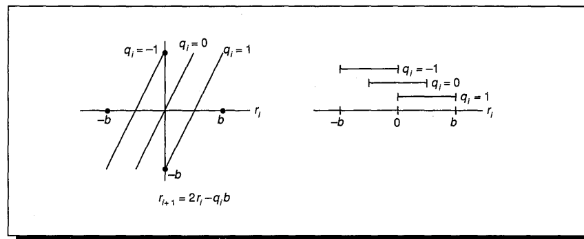
FIGURE A.28 Quotient selection for radix-2 division. The x axis represents the i th remainder, which is the quantity in the ( P,A ) register pair. The y axis shows the value of the remainder after one additional divide step. Each bar on the right-hand graph gives the range of r_i values for which it is permissible to select the associated value of q_i .
