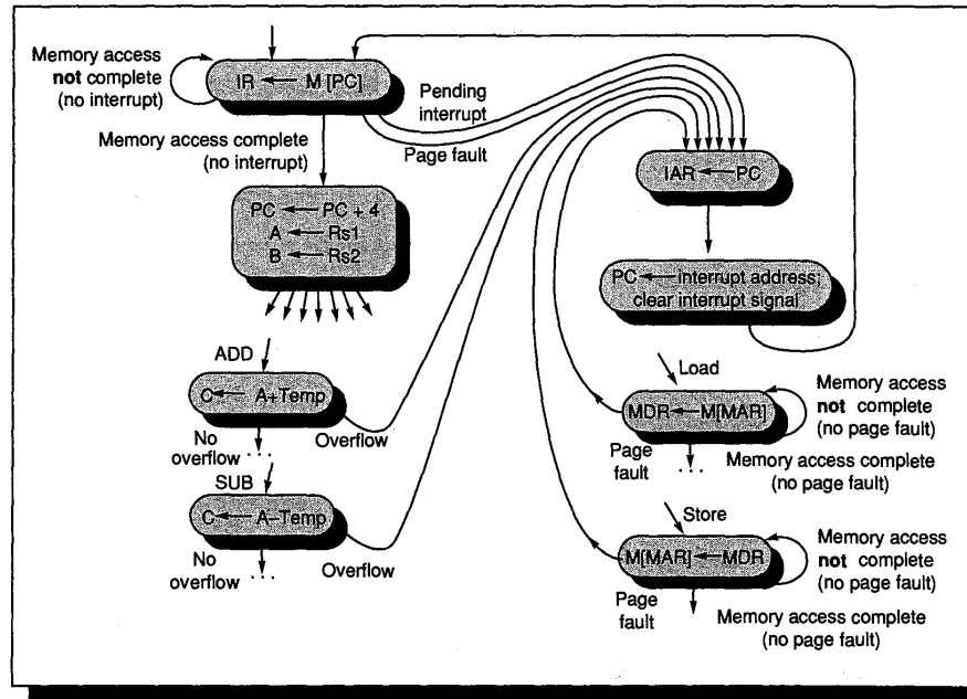
FIGURE 5.12 The top-level view of the DLX finite-state diagram (Figure 5.4 on page 207) modified to check for interrupts. Either a between-instruction or an instruction page fault invokes the control that saves the PC and then loads it with the address of the appropriate interrupt routine. The lower portion of the figure shows interrupts resulting in page faults of data accesses or arithmetic overflow.
