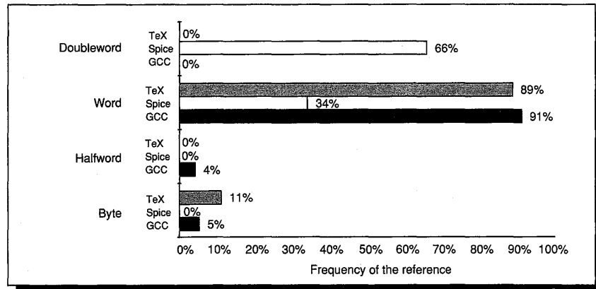
FIGURE 3.23 Distribution of data accesses by size for the benchmark programs. Access to the major data type (word or doubleword) clearly dominates. Reads outnumbered writes of data items by a factor of 1.6 for TeX to a factor of 2.5 for Spice. The doubleword data type is used solely for double-precision floating point in Spice. Spice makes only small use of single-precision floating point; most word references in Spice are to integers. These measurements were taken on the memory traffic generated on a load/store architecture.
