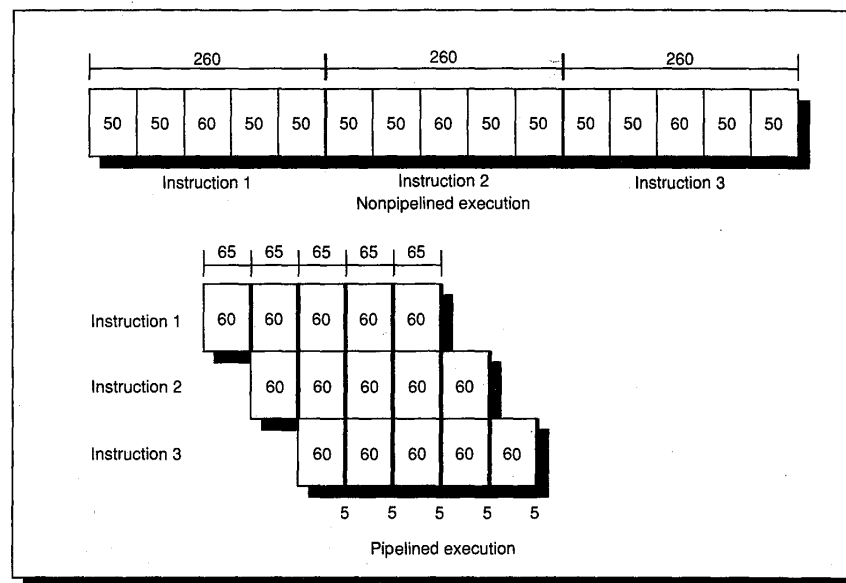
FIGURE 6.2 The execution pattern for three instructions shown for both the nonpipelined and pipelined versions. In the nonpipelined version, the three instructions are executed sequentially. In the pipelined version, the shaded areas represent the overhead of 5 ns per pipestage. The length of the pipestages must all be the same: 60 ns plus the 5-ns overhead. The latency of an instruction increases from 260 ns in the nonpipelined machine to 325 ns in the pipelined machine.
