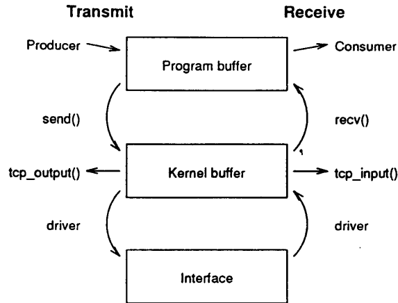
Figure 1: Data movements in a typical TCP/IP implementation
