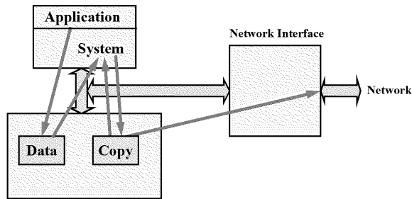
Figure 2: Data flow in traditional network interface
