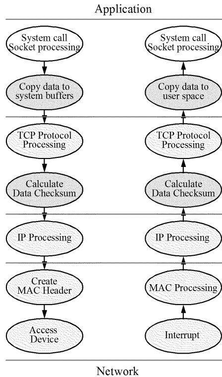
Figure 1: Network data processing overheads
