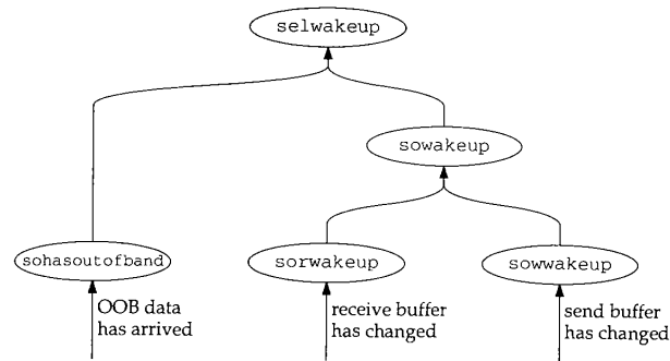
Figure 16.59 selwakeup processing.
