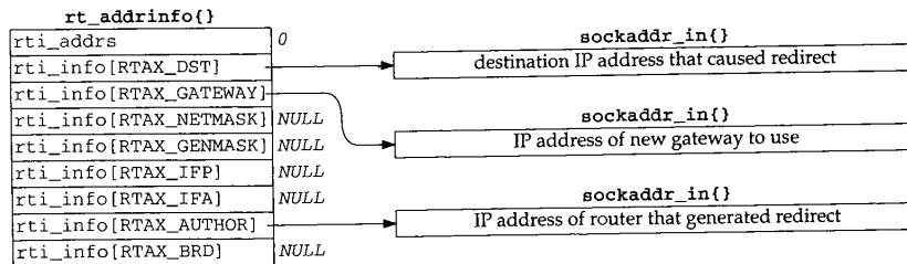
Figure 19.22 rt_addrinfo structure passed by rtredirect to rt_missmsg .
