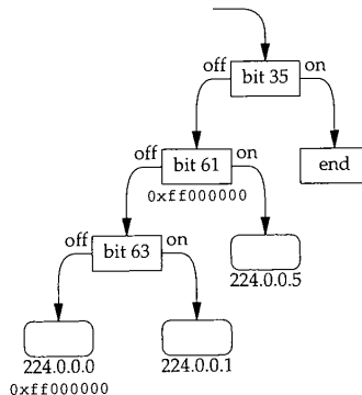
Figure 18.7 Modification of Figure 18.4 after inserting entry for 224.0.0.5 .
