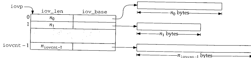
Figure 16.11 iovec arguments to writev .
