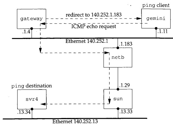
Figure 22.35 Example of ICMP redirect.
