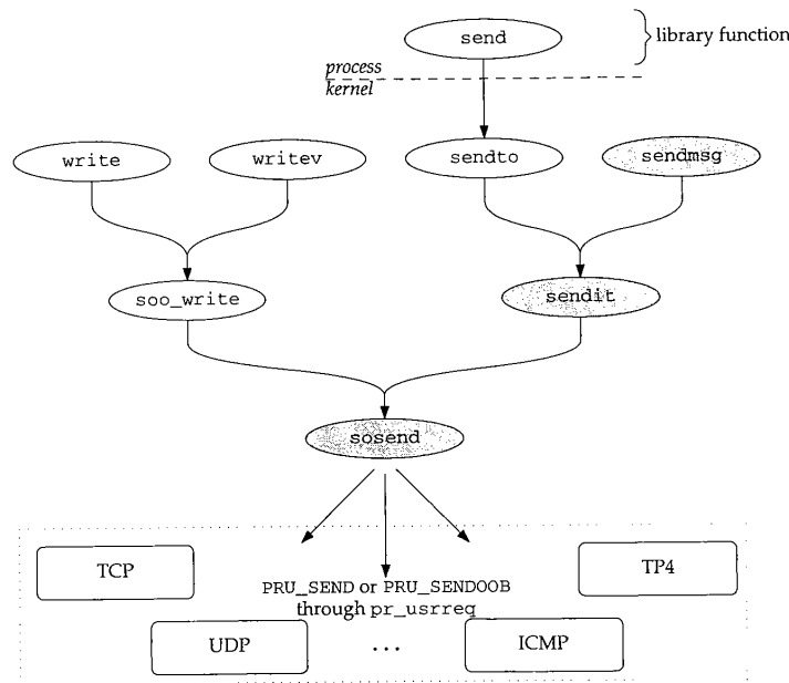
Figure 16.8 All socket output is handled by sosend .
