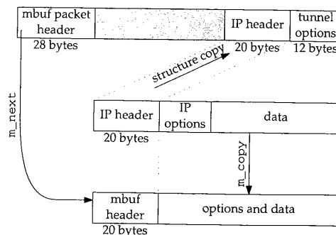
Figure 14.42 Inserting tunnel options.
