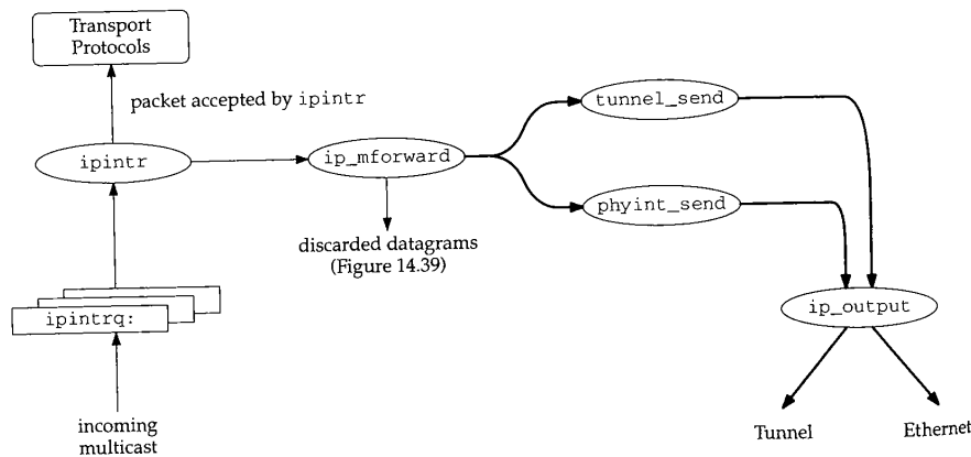
Figure 14.35 Multicast datagram arriving on physical interface.
