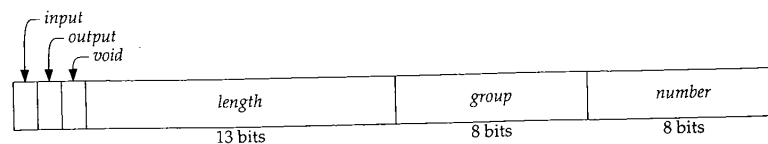
Figure 17.19 The structure of an ioctl command.
