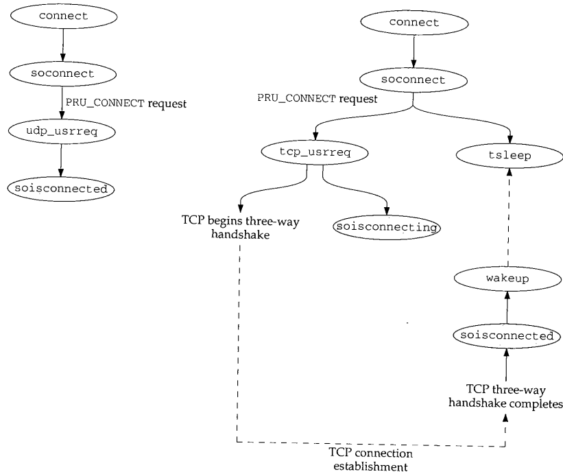
Figure 15.31 connect processing.
