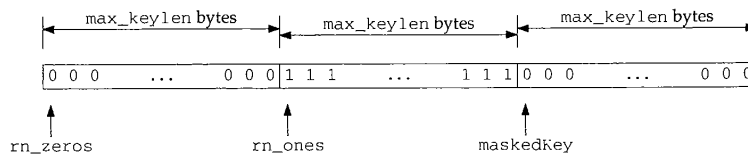
Figure 18.33 rn_zeros, rn_ones, and maskedKey arrays.
