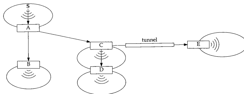
Figure 14.25 Spanning tree for network A.
