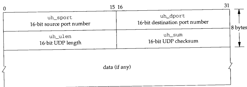
Figure 23.10 UDP header and optional data.
