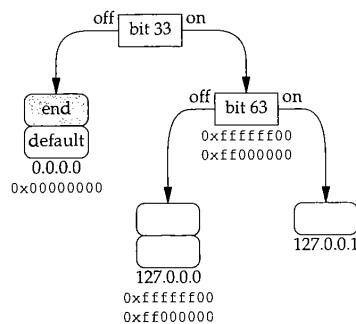
Figure 18.36 Routing tree showing duplicate keys for 127.0.0.0.
