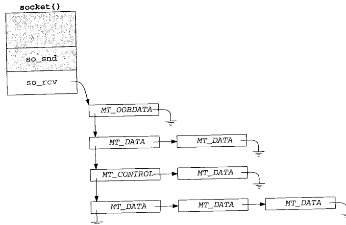
Figure 16.37 so_rcv buffer with control and OOB data.
