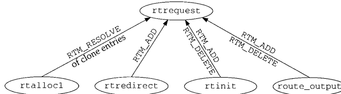
Figure 19.6 Summary of functions that call rtrequest .
