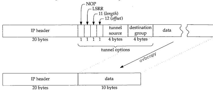
Figure 14.38 Multicast tunnel options.
