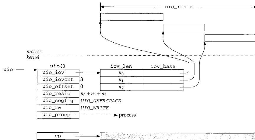
Figure 16.19 uiomove: before.
