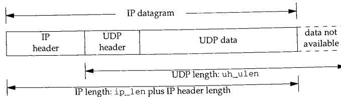
Figure 23.23 UDP length too big.
