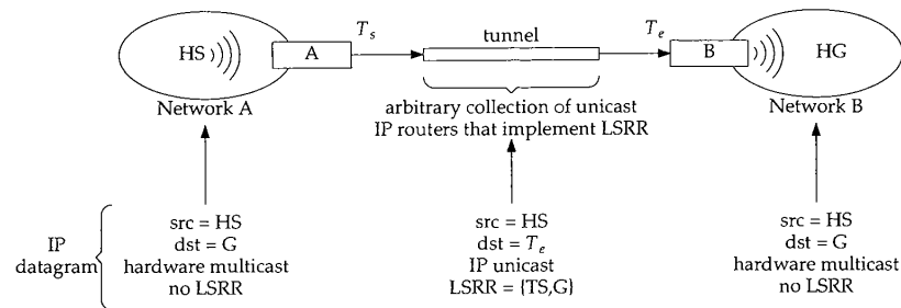
Figure 14.12 A multicast tunnel.
