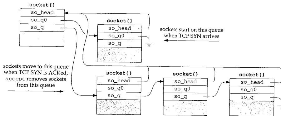
Figure 15.8 Socket connection queues.
