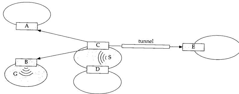
Figure 14.26 TRPB routing for network C.
