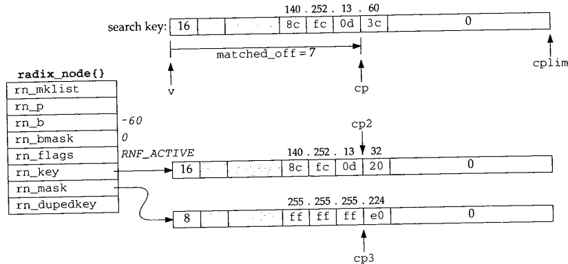
Figure 18.41 Example for network mask comparison.
