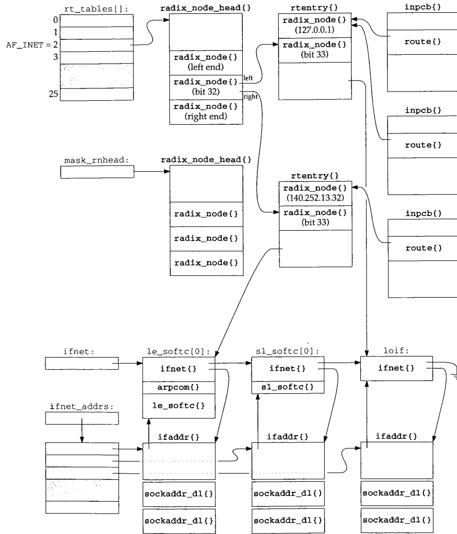
Figure 18.8 Data structures involved with routing tables.
