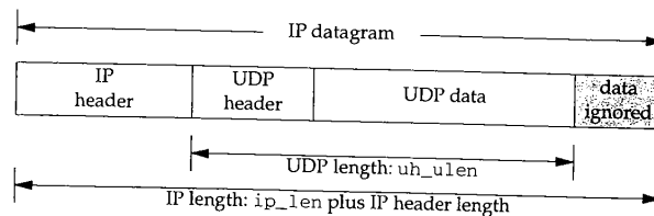
Figure 23.22 UDP length too small.
