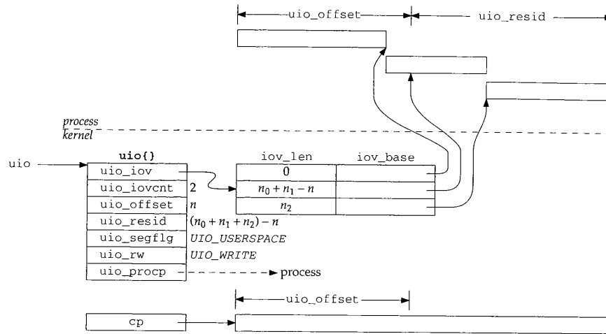
Figure 16.20 uiomove: after.
