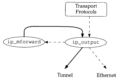
Figure 14.7 Multicast output processing with no loopback.
