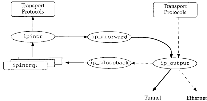
Figure 14.6 Multicast output processing with loopback.
