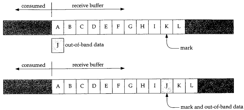
Figure 16.34 Receiving out-of-band data.
