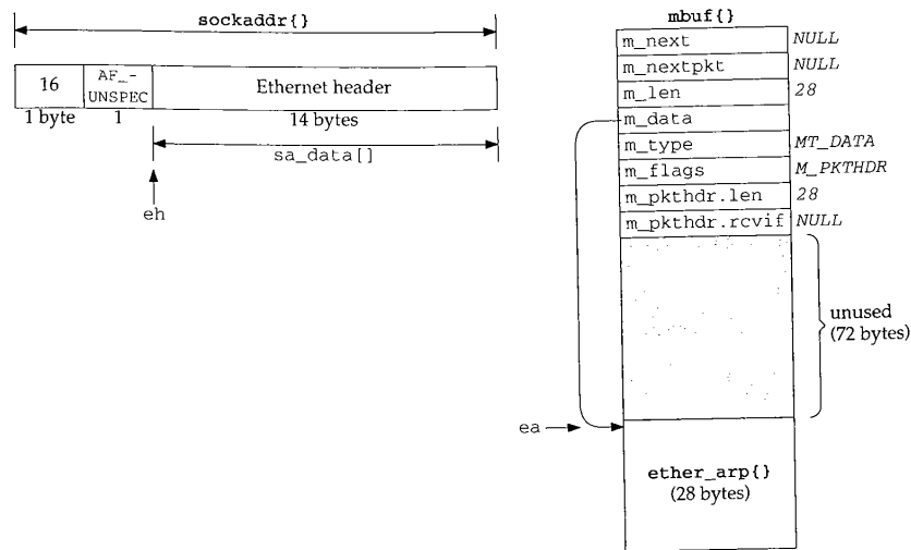
Figure 21.12 sockaddr and mbuf built by arprequest .
