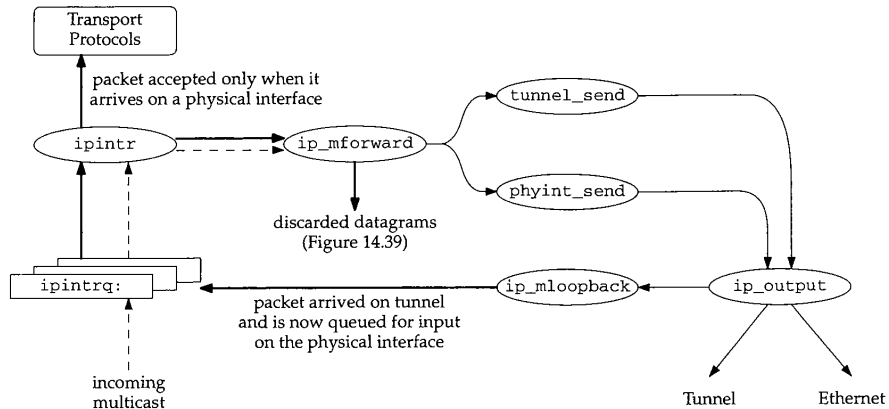
Figure 14.36 Multicast datagram arriving on a multicast tunnel.
