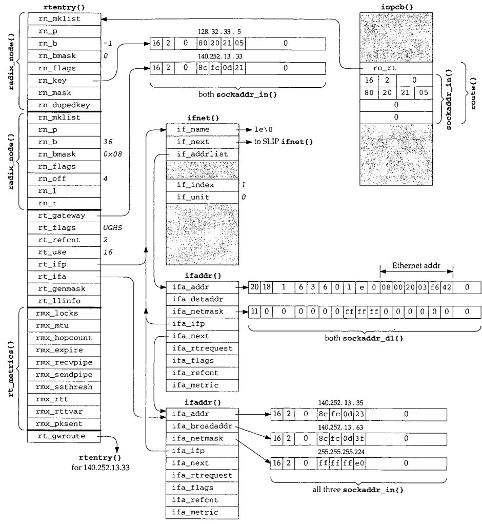
Figure 18.28 Summary of routing structures.
