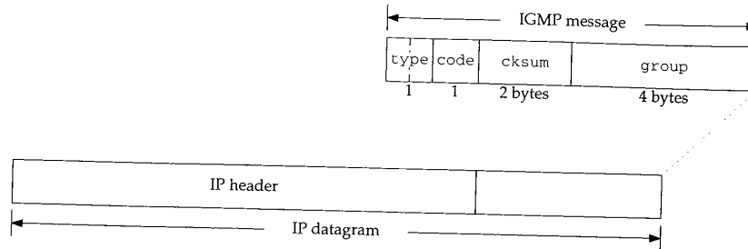
Figure 13.8 An IGMP message (igmp_omitted).
