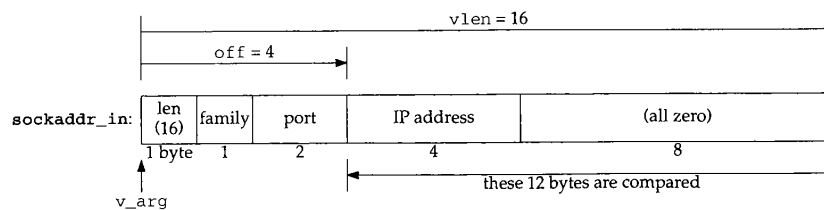
Figure 18.39 Variables during comparison of sockadr_in structures.
