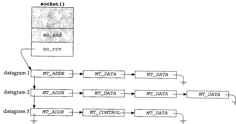
Figure 16.35 UDP receive buffer consisting of three datagrams.
