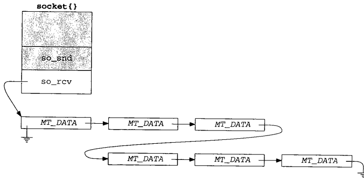
Figure 16.36 so_rcv buffer for TCP.
