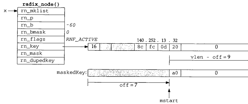
Figure 18.46 Comparison of maskedKey and new leaf.
