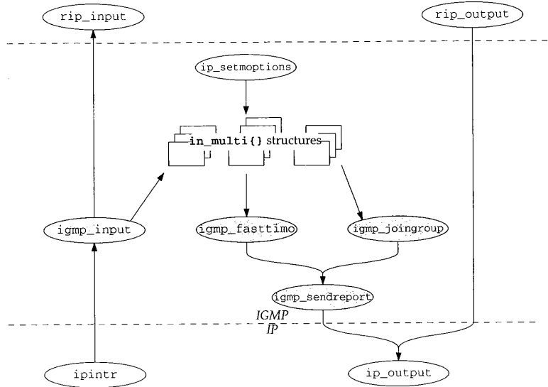
Figure 13.1 Summary of IGMP processing.
