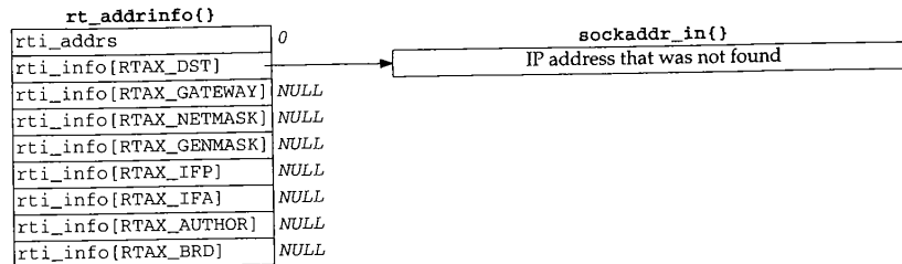
Figure 19.21 rt_addrinfo structure passed by rtalloc1 to rt_missmsg .
