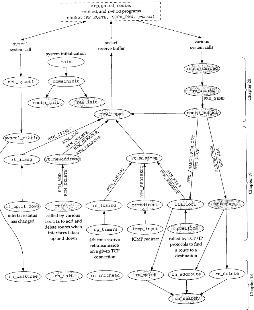
Figure 18.11 Relationships between the various routing functions.
