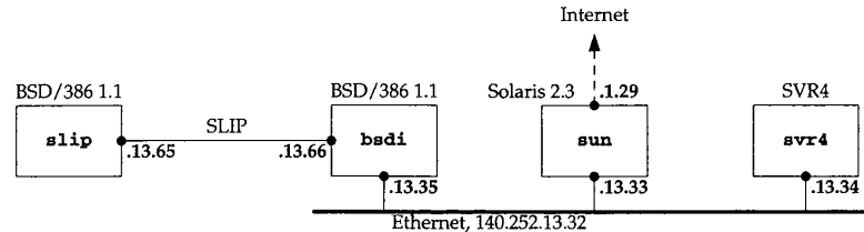
Figure 18.1 Subnet used for routing table example.
