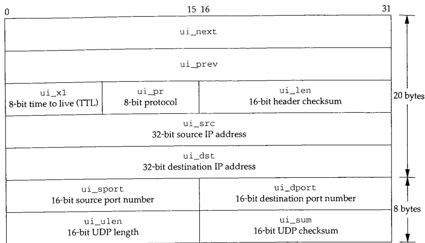
Figure 23.18 udphdr structure used by udp_output.
