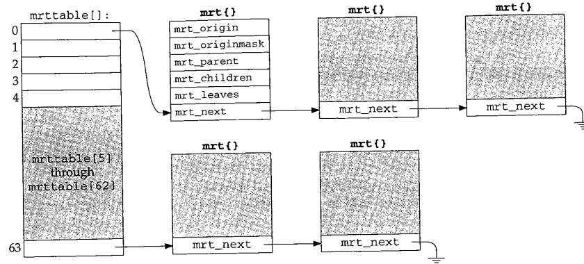
Figure 14.29 Multicast routing table.
