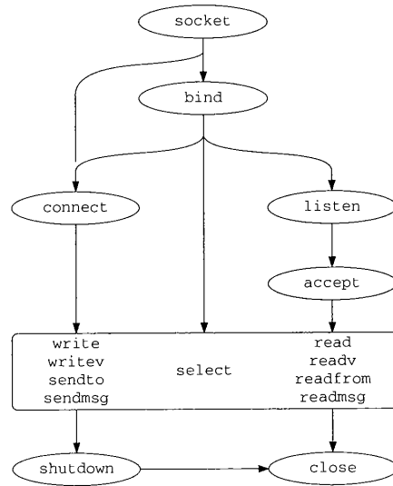
Figure 15.12 Network system call flowchart.
