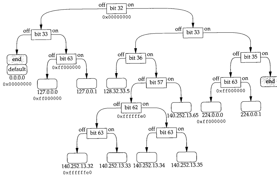
Figure 18.4 Net/3 routing table corresponding to Figure 18.2.
