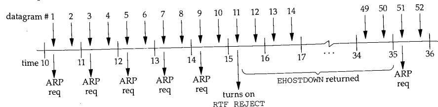
Figure 21.25 Algorithm used to avoid ARP flooding.
