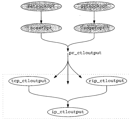
Figure 17.1 setsockopt and getsockopt system calls.
