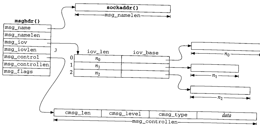
Figure 16.15 msghdr structure for sendmsg system call.
