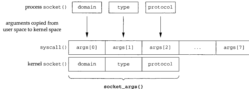
Figure 15.10 socket argument processing.
