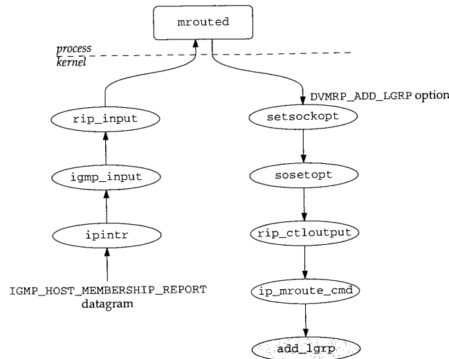
Figure 14.20 IGMP report processing.
