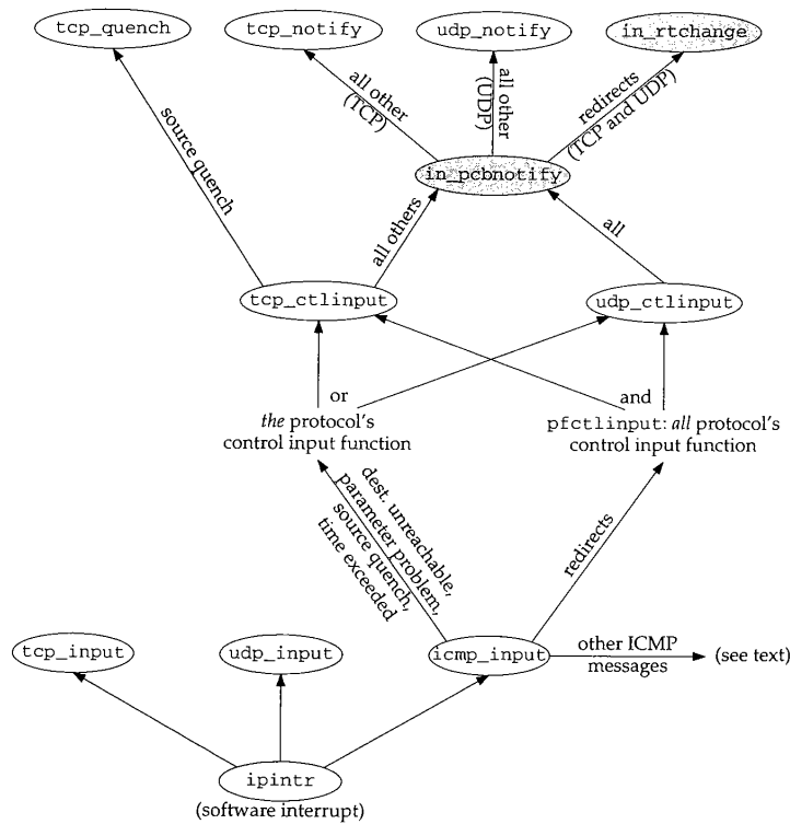
Figure 22.32 Summary of processing of ICMP errors.
