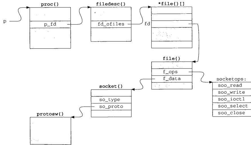
Figure 15.13 Process, file, and socket structures.
