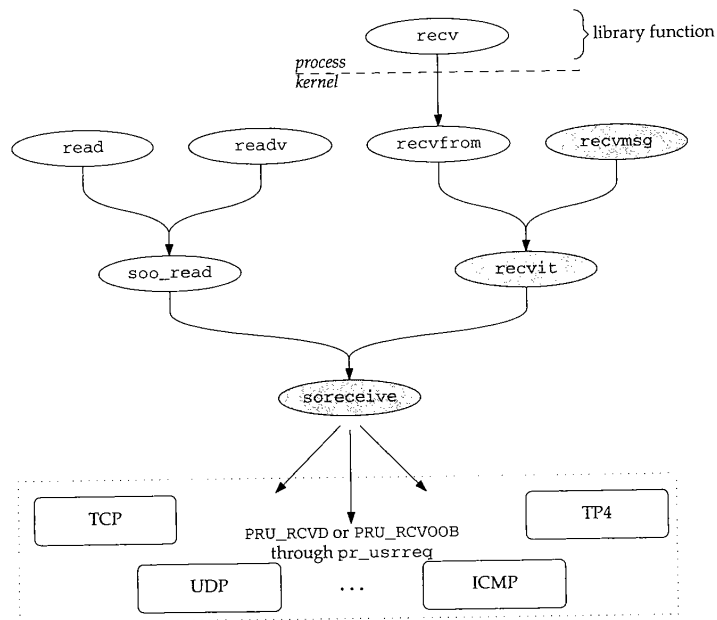
Figure 16.28 All socket input is processed by soreceive .
