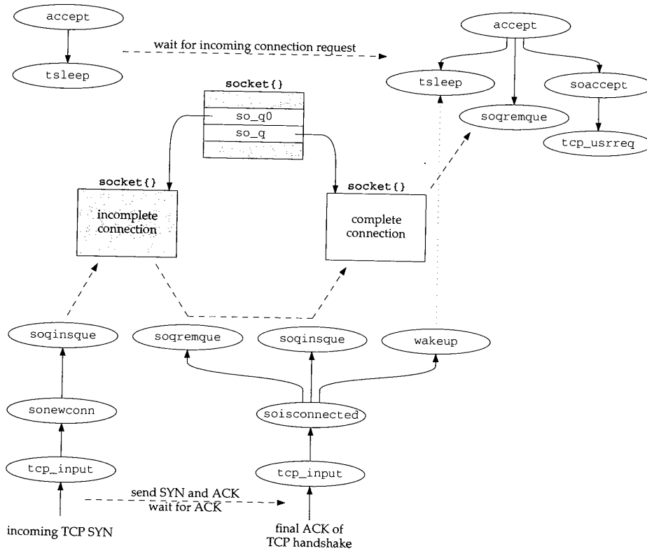
Figure 15.28 Incoming TCP connection processing.
