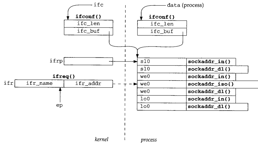
Figure 4.25 ifconf data structures.
