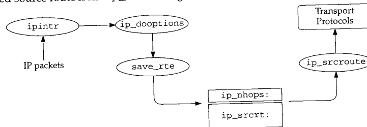
Figure 9.17 Processing of reversed source routes.
