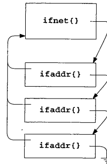
Figure 3.5 Each ifnet structure has a list of associated ifaddr structures.
