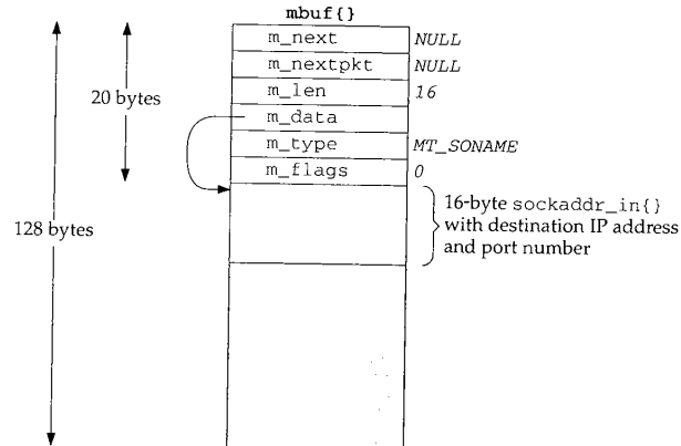
Figure 1.6 Mbuf containing destination address for sendto .
