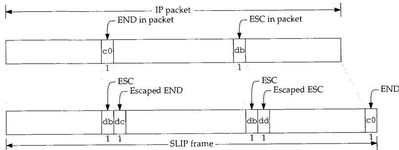
Figure 5.5 SLIP encapsulation of an IP packet.
