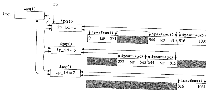
Figure 10.17 Reassembly of three IP datagrams.
