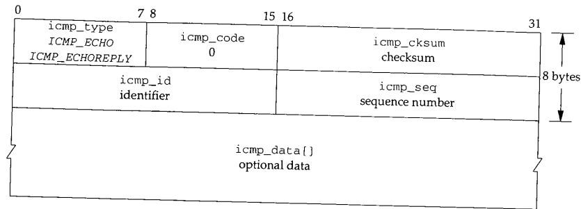
Figure 11.20 ICMP echo request and reply.
