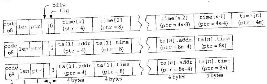
Figure 9.23 The three timestamp options (ipt_omitted).
