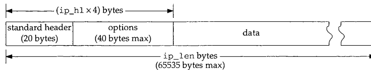
Figure 8.10 Organization of an IP packet with options.
