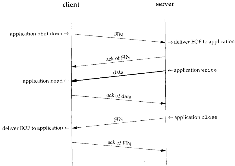
Figure 18.10 Example of TCP's half-close.
