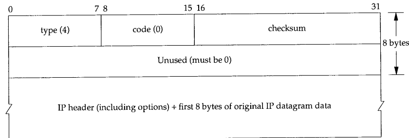
Figure 11.18 ICMP source quench error.
