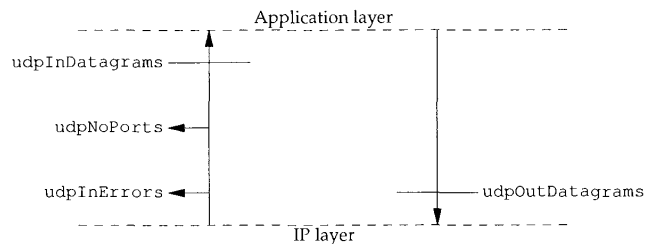
Figure 25.10 Case Diagram for UDP group.
