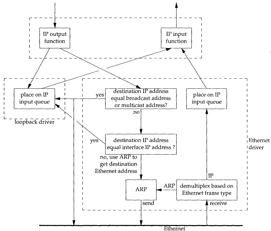
Figure 2.4 Processing of IP datagrams by loopback interface.
