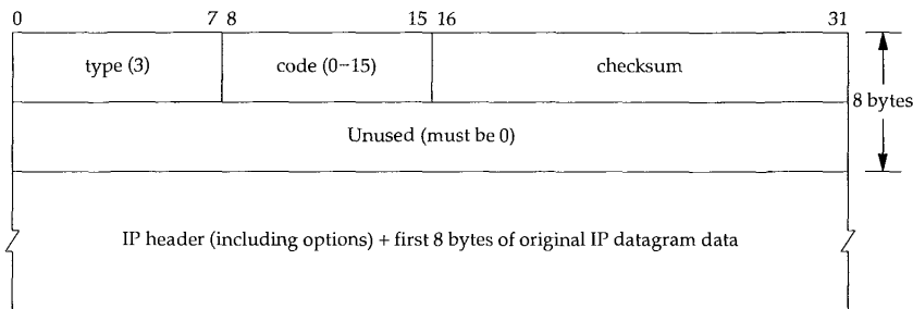
Figure 6.10 ICMP unreachable message.
