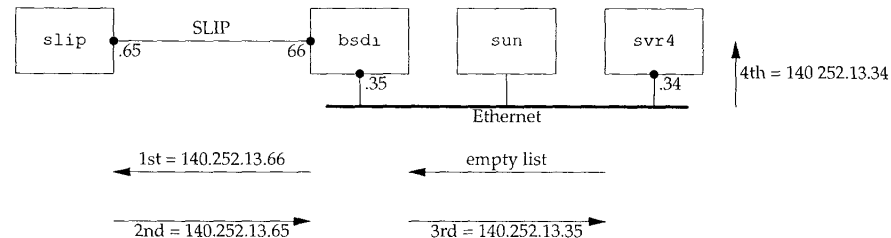
Figure 7.4 ping with record route option.
