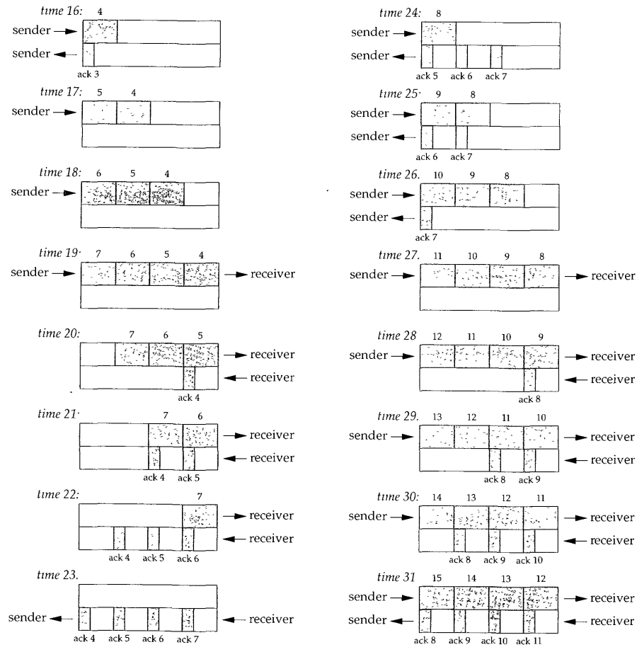
Figure 20.10 Times 16-31 for bulk data throughput example.
