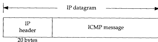
Figure 6.1 ICMP messages encapsulated within an IP datagram.
