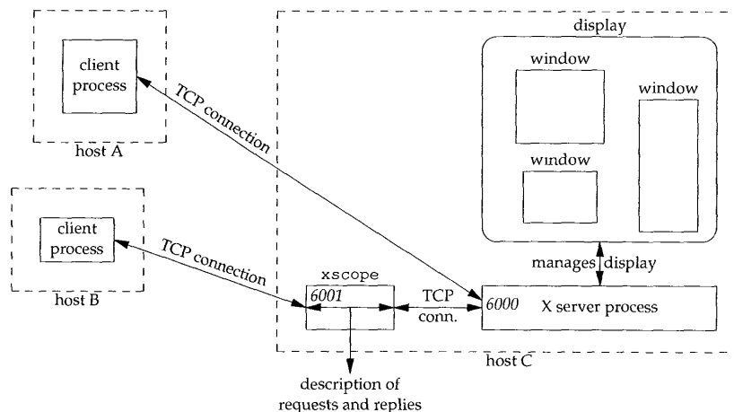
Figure 30.3 Using xscope to monitor an X connection.
