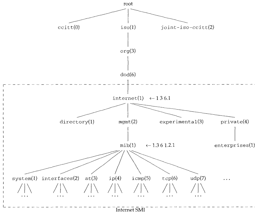
Figure 25.6 Object identifiers in the Management Information Base.
