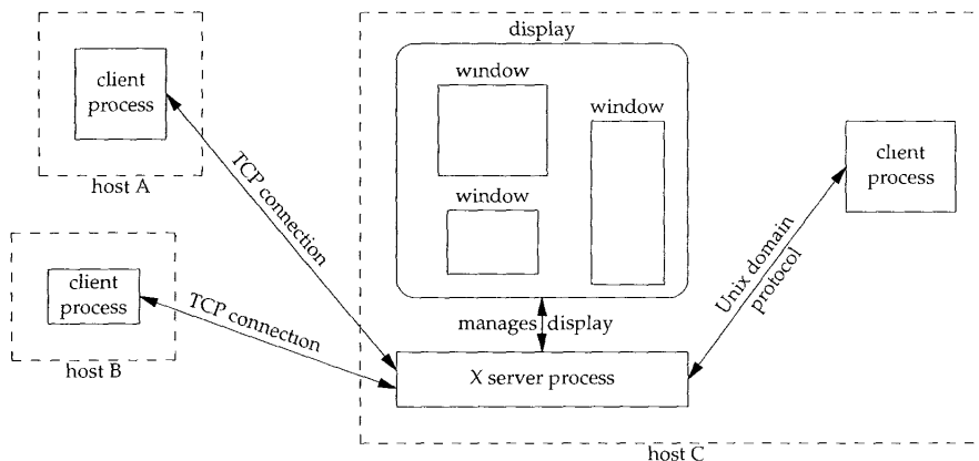
Figure 30.2 Three clients using one display.
