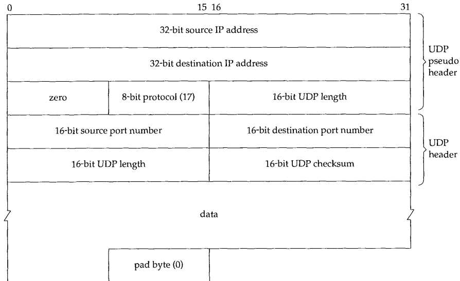
Figure 11.3 Fields used for computation of UDP checksum.
