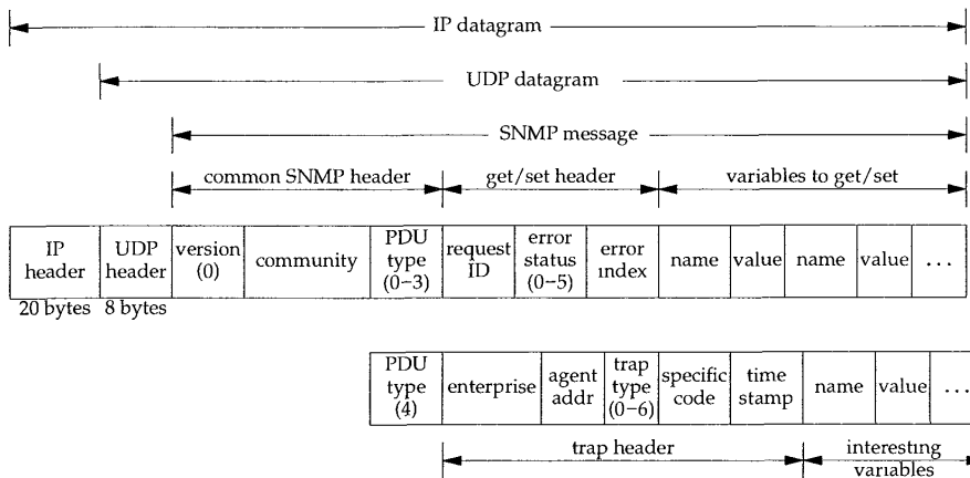
Figure 25.2 Format of the five SNMP messages.
