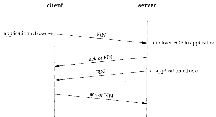
Figure 18.4 Normal exchange of segments during connection termination.
