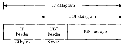
Figure 10.2 RIP message encapsulated within a UDP datagram.
