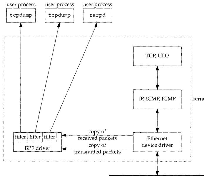
Figure A.1 BSD Packet Filter.
