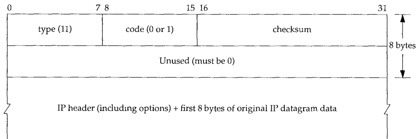
Figure 8.2 ICMP time exceeded message.
