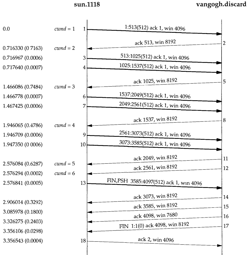
Figure 20.8 Example of slow start.
