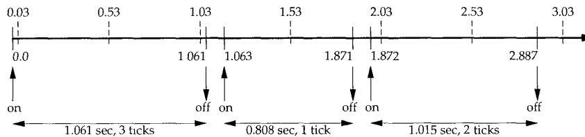
Figure 21.3 RTT measurements and clock ticks.
