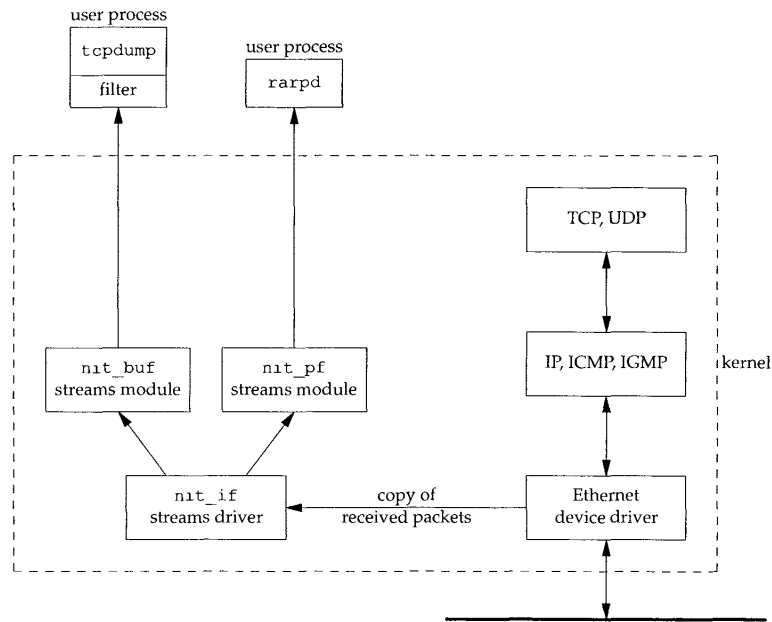
Figure A.2 SunOS Network Interface Tap.
