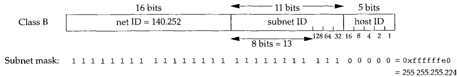
Figure 3.11 Using variable-length subnets.
