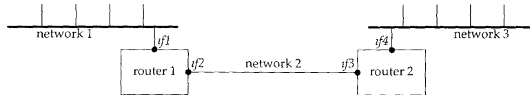
Figure 8.3 Identification of interfaces printed by traceroute.
