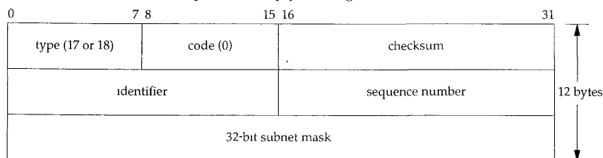
Figure 6.4 ICMP address mask request and reply messages.
