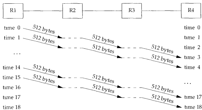
Figure 24.4 Sending sixteen 512-byte packets through four routers
