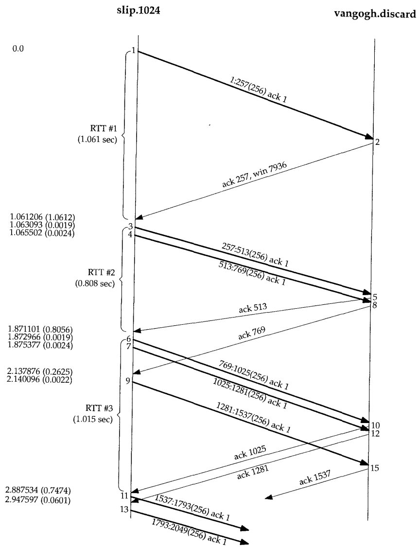
Figure 21.2 Packet exchange and RTT measurement.
