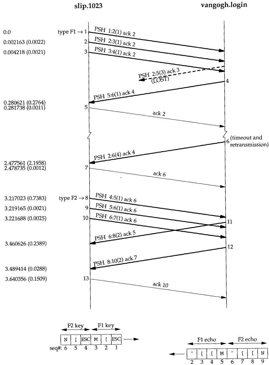
Figure 19.8 Time line for Figure 19.7 (Nagle algorithm disabled).
