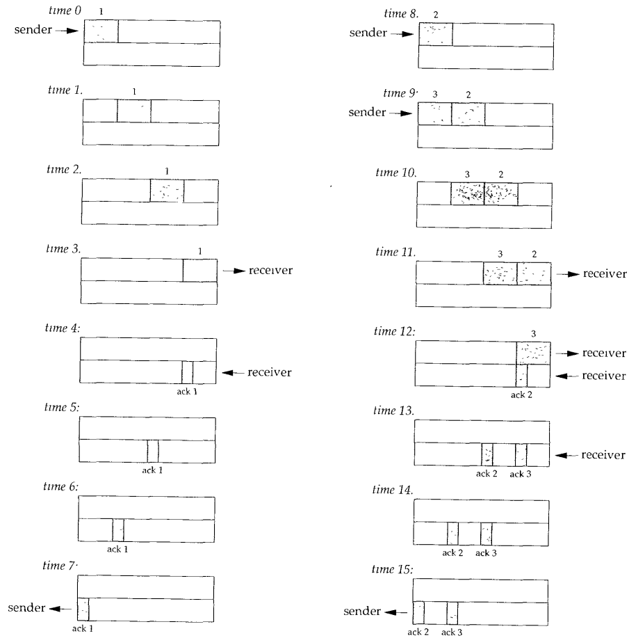
Figure 20.9 Times 0-15 for bulk data throughput example.
