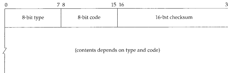
Figure 6.2 ICMP message.
