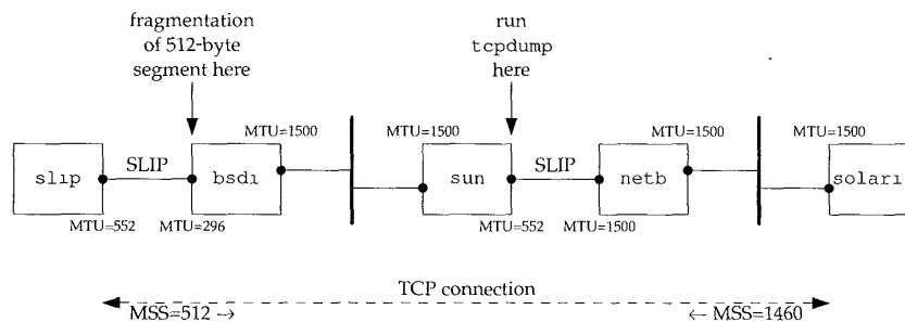
Figure 24.1 Topology for path MTU example.
