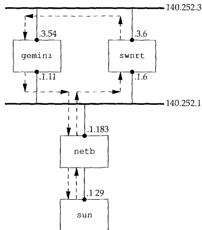
Figure 25.29 Topology of systems being used for example.
