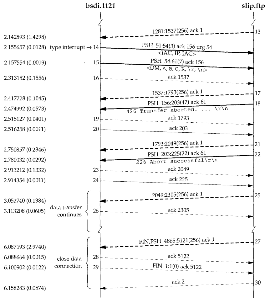
Figure 27.10 Aborting a file transfer (second half).
