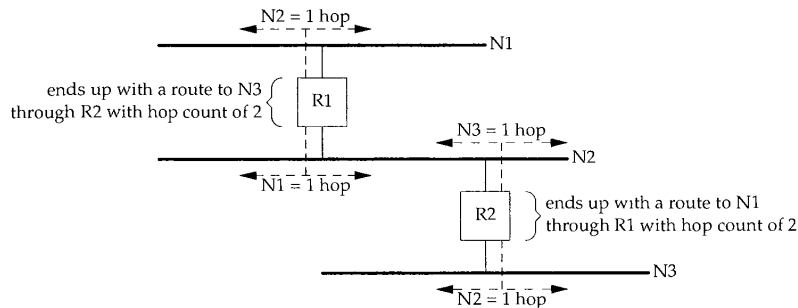
Figure 10.4 Example routers and networks
