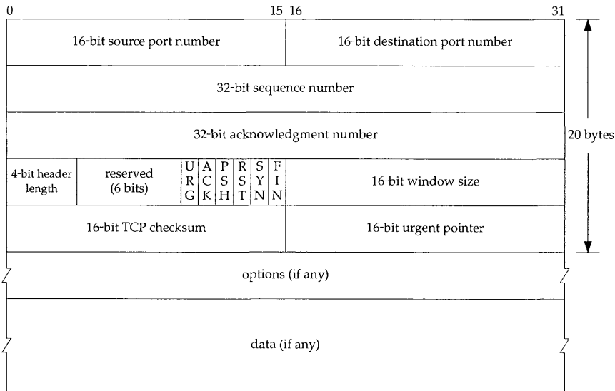
Figure 17.2 TCP header.
