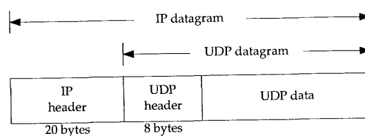
Figure 11.1 UDP encapsulation.
