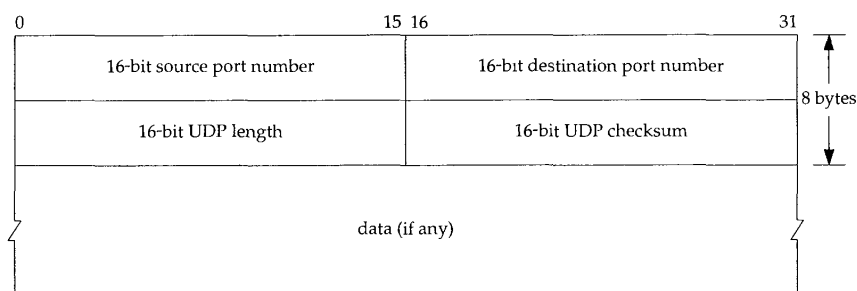
Figure 11.2 UDP header.
