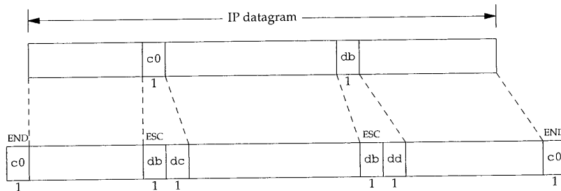
Figure 2.2 SLIP encapsulation.
