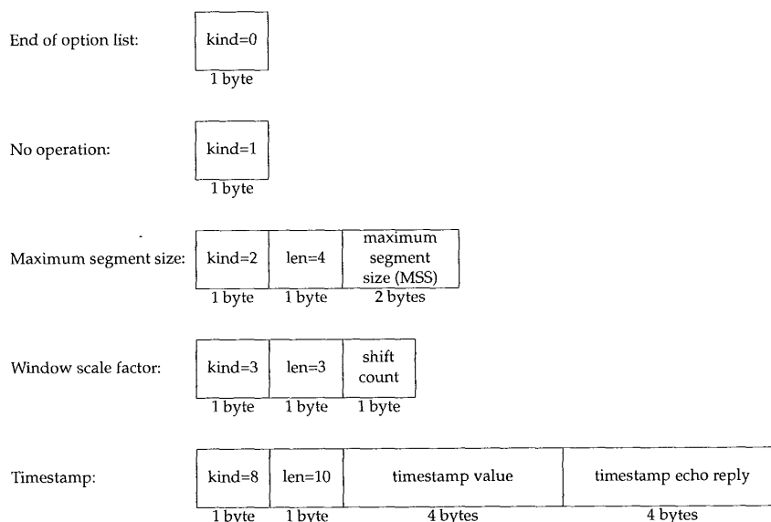
Figure 18.20 TCP options.
