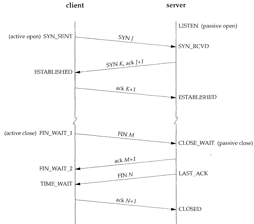
Figure 18.13 TCP states corresponding to normal connection establishment and termination.
