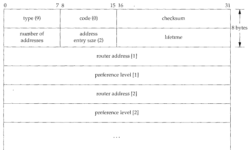
Figure 9.7 Format of ICMP router advertisement message.
