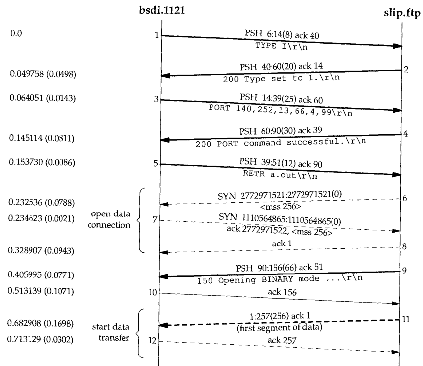
Figure 27.9 Aborting a file transfer (first half).
