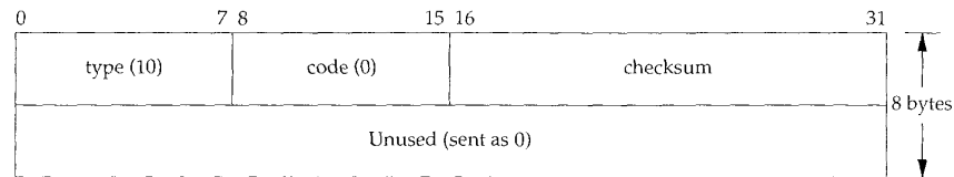
Figure 9.6 Format of ICMP router solicitation message.
