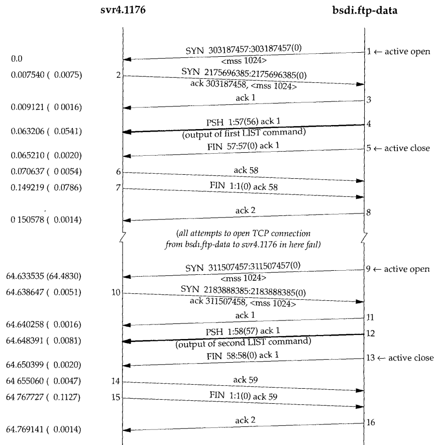
Figure 27.8 Data connection for two consecutive LIST commands.
