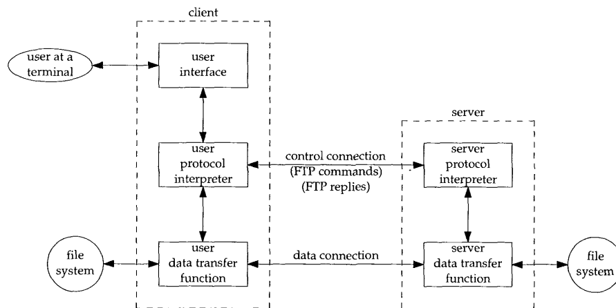
Figure 27.1 Processes involved in file transfer.
