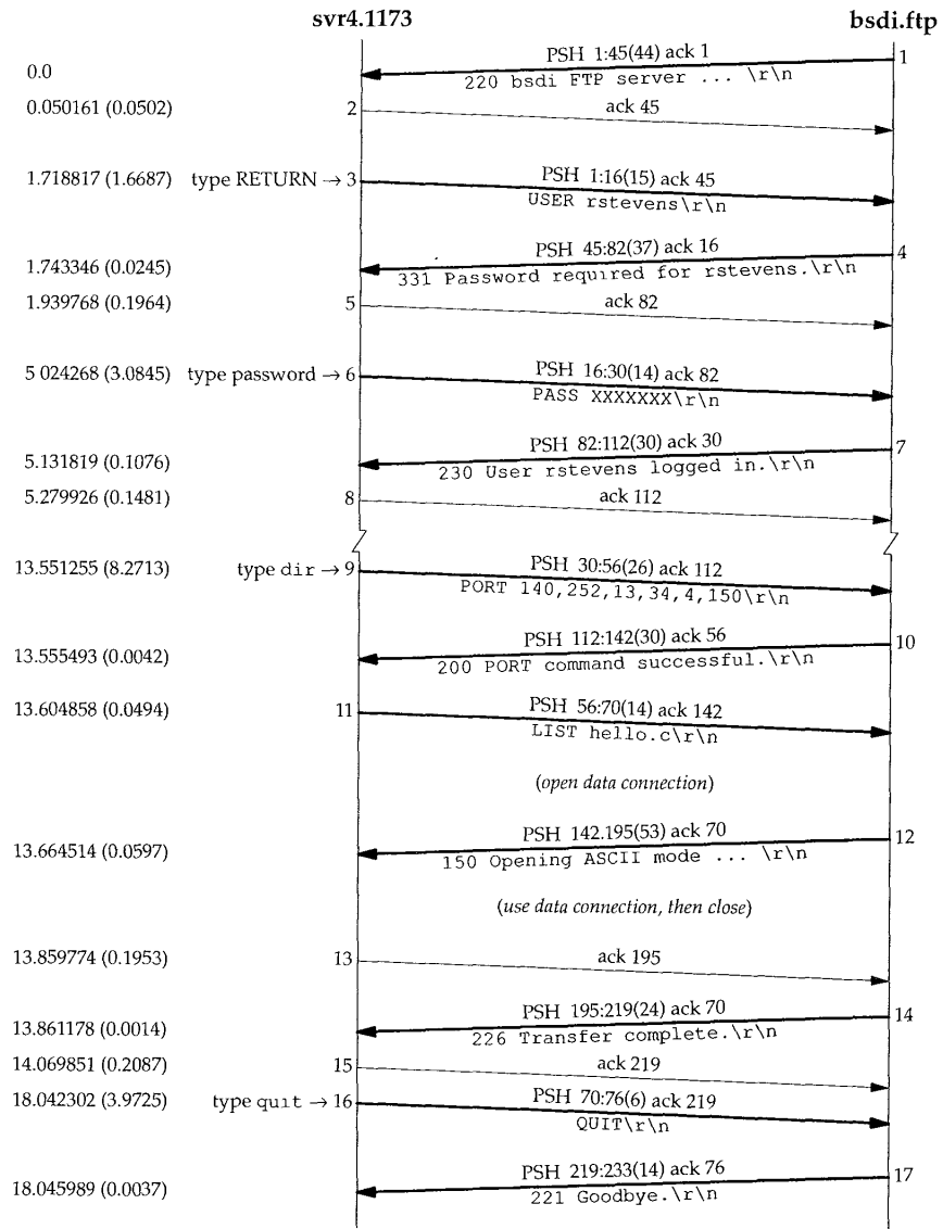
Figure 27.6 Control connection for FTP example.
