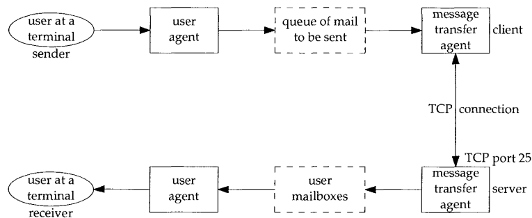
Figure 28.1 Outline of Internet electronic mail.
