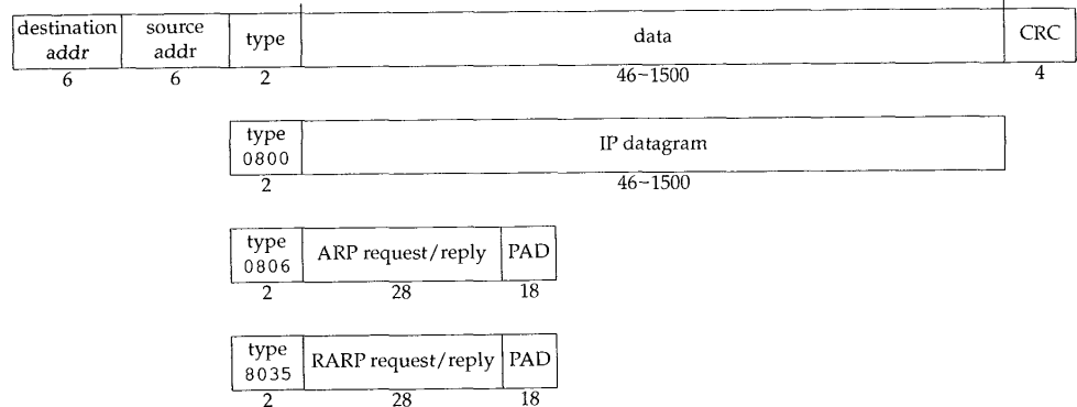
Figure 2.1 IEEE 802.2/802.3 encapsulation (RFC 1042) and Ethernet encapsulation (RFC 894).
