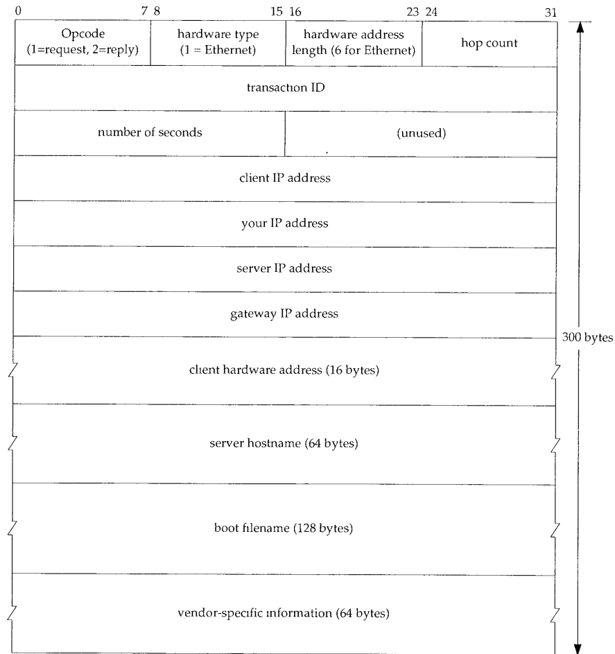
Figure 16.2 Format of BOOTP request and reply.
