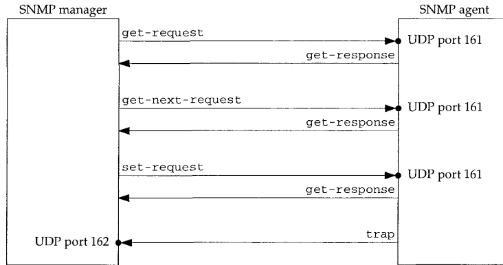
Figure 25.1 Summary of the five SNMP operators.
