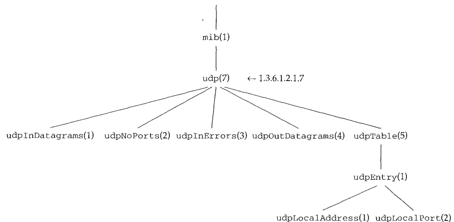
Figure 25.7 Tree structure of UDP group.
