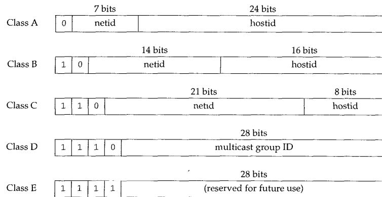
Figure 1.5 The five different classes of Internet addresses.
