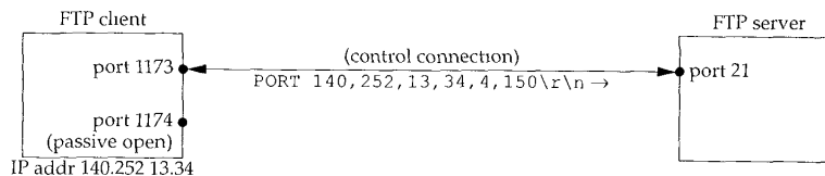
Figure 27.4 PORT command going across FTP control connection.
