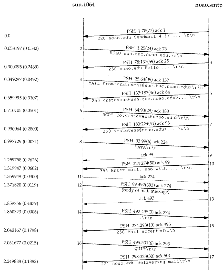
Figure 28.2 Basic SMTP mail delivery
