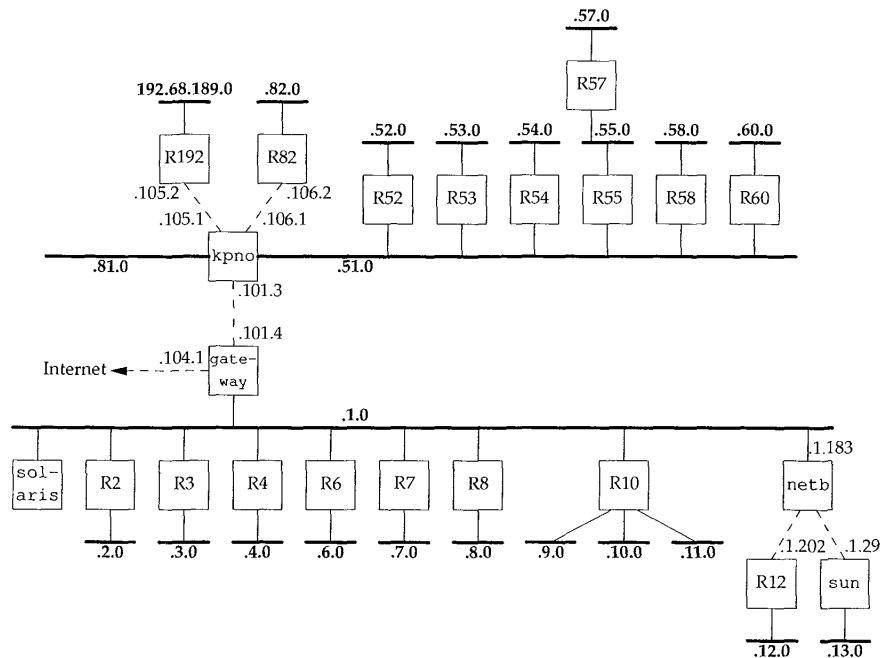
Figure 10.7 Many of the noao.edu 140.252 networks.
