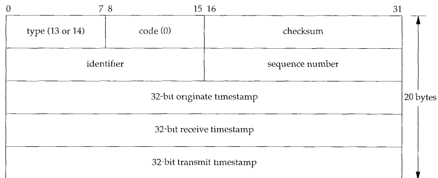
Figure 6.6 ICMP timestamp request and reply messages.
