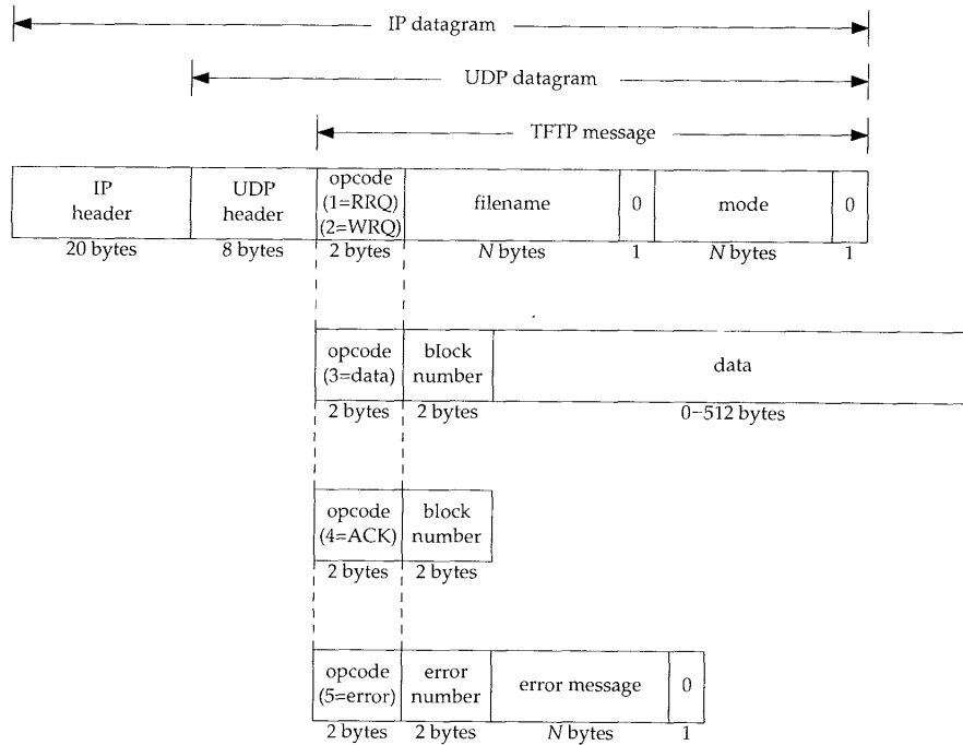
Figure 15.1 Format of the five TFTP messages.
