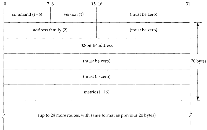
Figure 10.3 Format of a RIP message.
