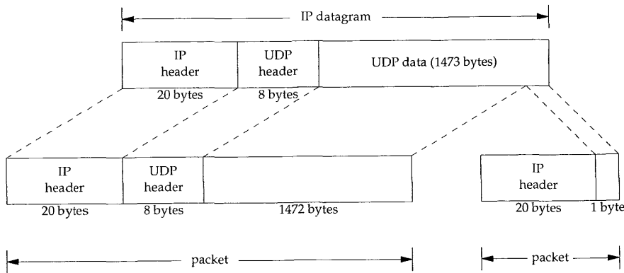
Figure 11.8 Example of UDP fragmentation.
