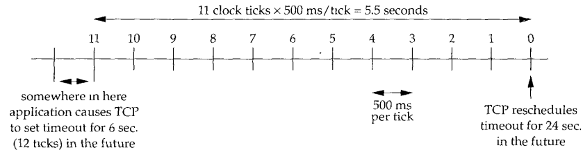
Figure 18.7 TCP 500-ms timer.
