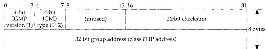
Figure 13.2 Format of fields in IGMP message.
