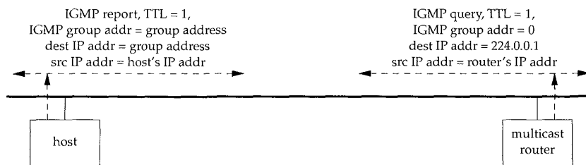
Figure 13.3 IGMP reports and queries.
