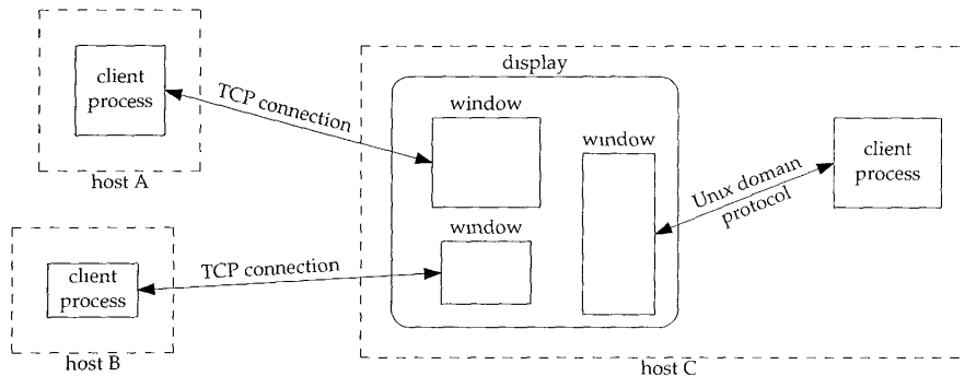
Figure 30.1 Three X clients using one display
