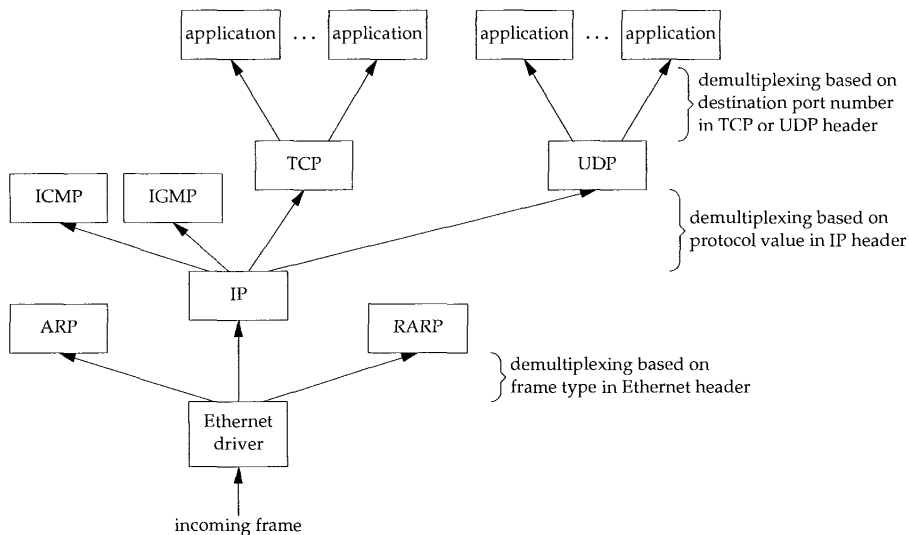
Figure 1.8 The demultiplexing of a received Ethernet frame.
