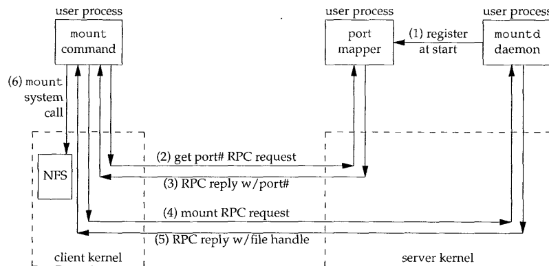
Figure 29.5 Mount protocol used by Unix mount command.
