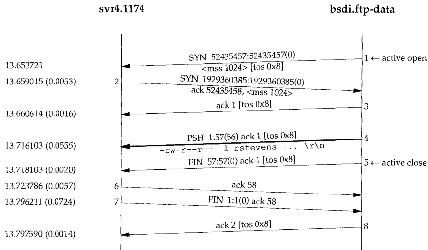
Figure 27.7 Data connection for FTP example.
