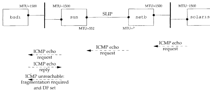
Figure 11.12 Packets exchanged in example.
