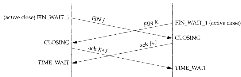
Figure 18.19 Segments exchanged during simultaneous close.
