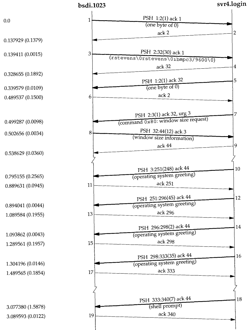
Figure 26.5 Time line for an Rlogin connection.
