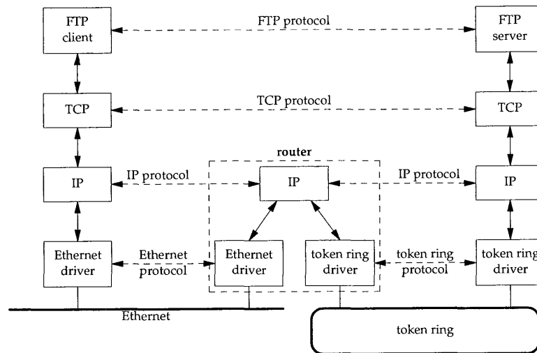
Figure 1.3 Two networks connected with a router.
