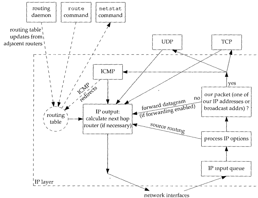
Figure 9.1 Processing done at the IP layer.
