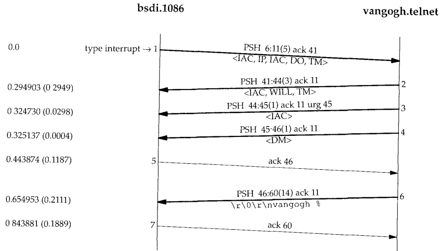
Figure 26.17 Typing interrupt key during linemode operation.
