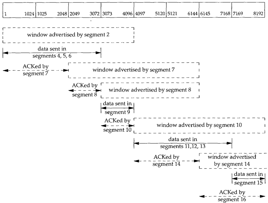
Figure 20.6 Sliding window protocol for Figure 20.1.
