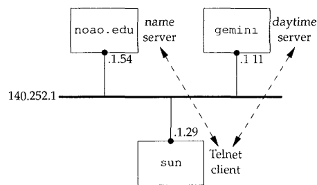
Figure 14.9 Systems being used for simple DNS example.
