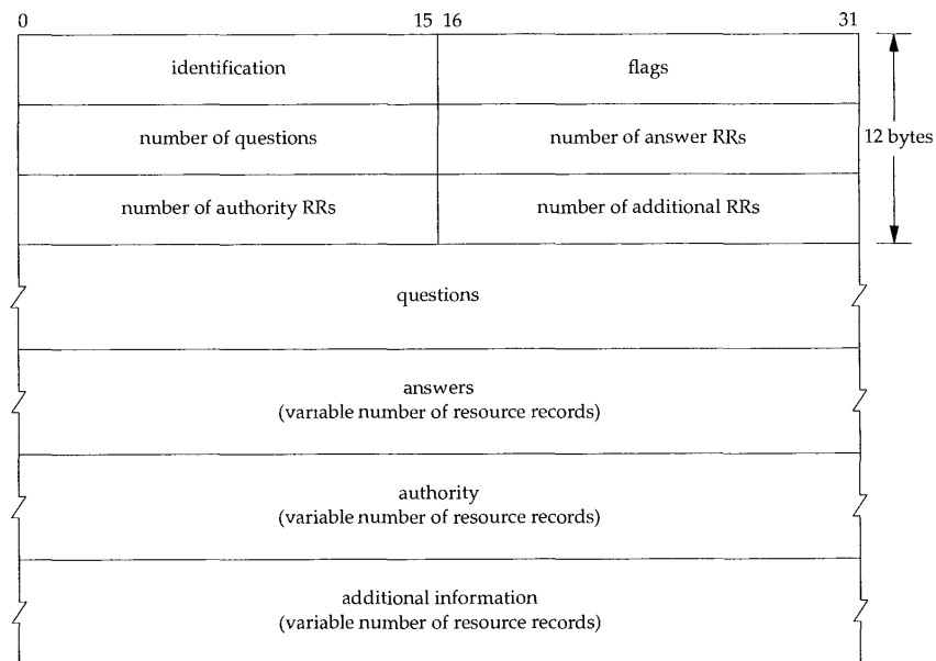
Figure 14.3 General format of DNS queries and responses.
