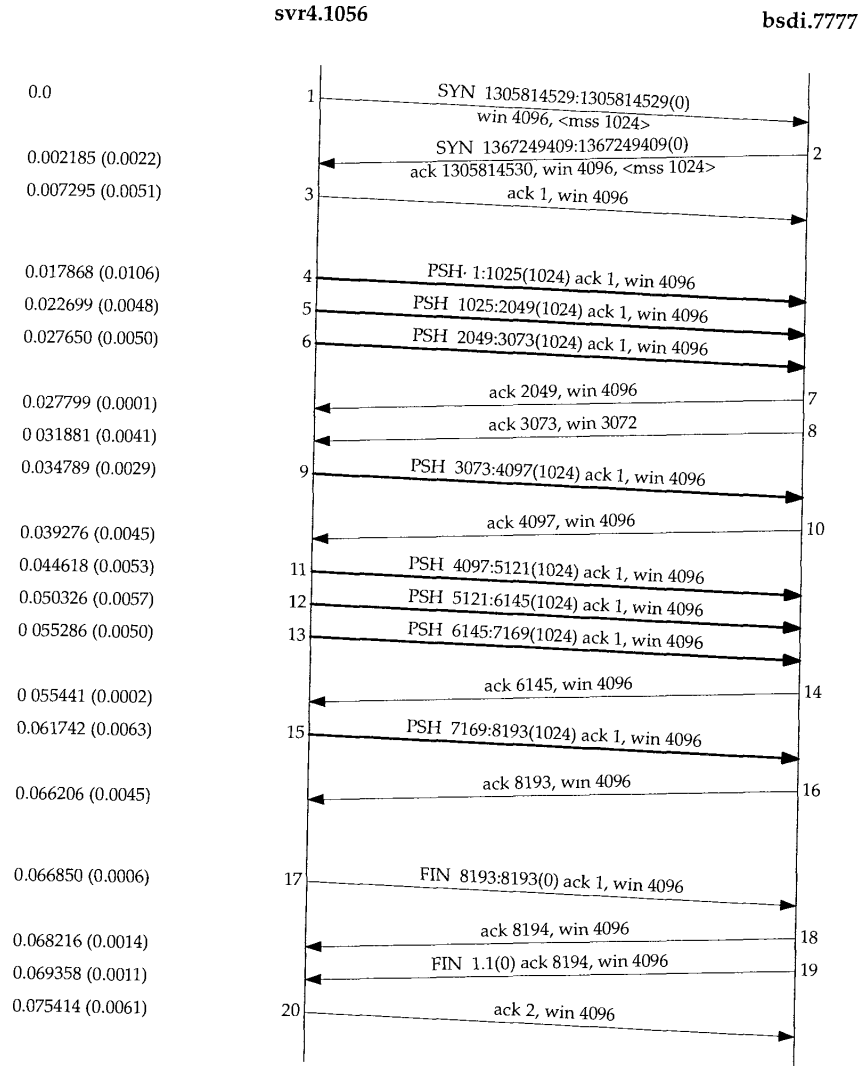
Figure 20.1 Transfer of 8192 bytes from svr4 to bsd1 .
