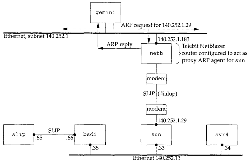
Figure 4.6 Example of proxy ARP.
