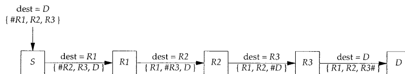
Figure 8.7 Example of IP source routing.
