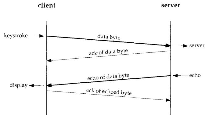
Figure 19.1 One possible way to do remote echo of interactive keystroke.
