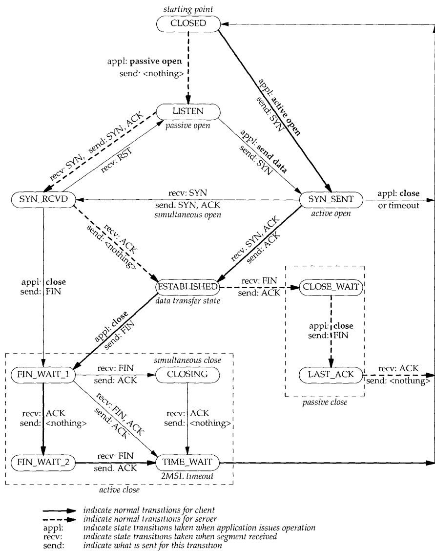
Figure 18.12 TCP state transition diagram.
