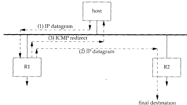
Figure 9.3 Example of an ICMP redirect.
