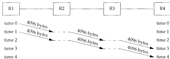
Figure 24.3 Sending two 4096-byte packets through four routers.
