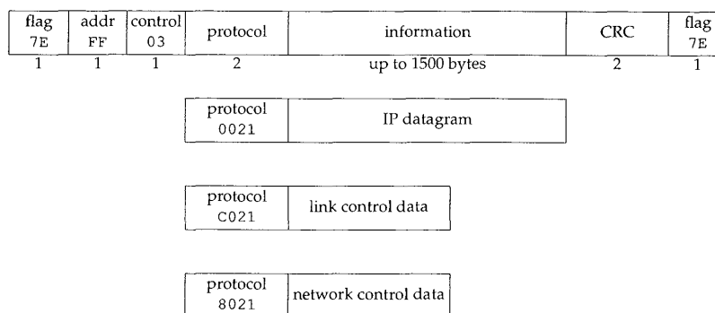
Figure 2.3 Format of PPP frames.
