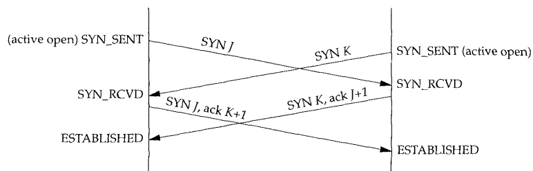
Figure 18.17 Segments exchanged during simultaneous open.
