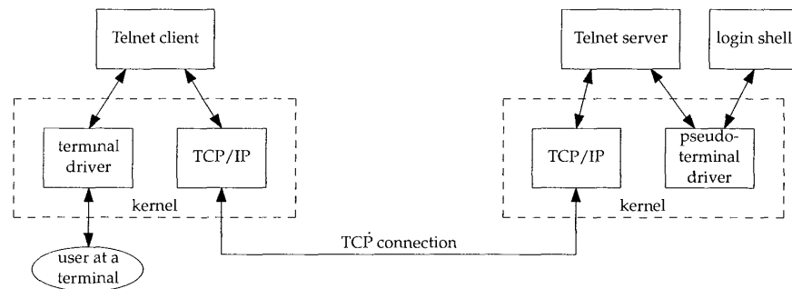
Figure 26.1 Overview of Telnet client-server.
