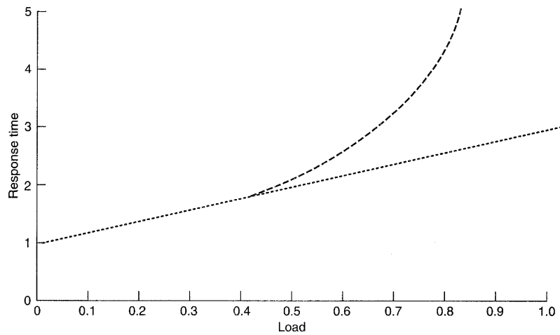
Fig. 6-47. Response as a function of load.
