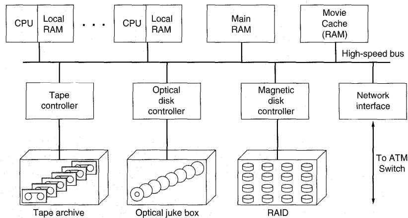
Fig. 7-90. The hardware architecture of a typical video server.
