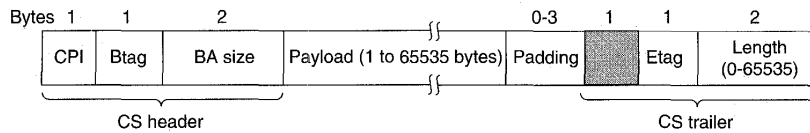
Fig. 6-42. AAL 3/4 convergence sublayer message format.
