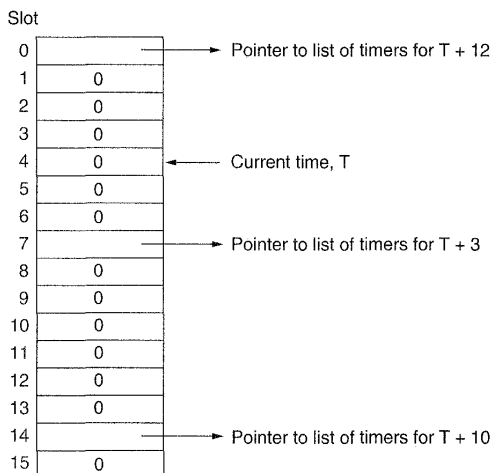
Fig. 6-51. A timing wheel.
