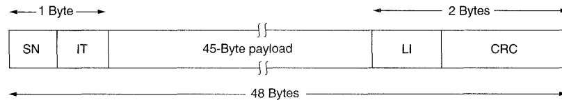
Fig. 6-40. The AAL 2 cell format.
