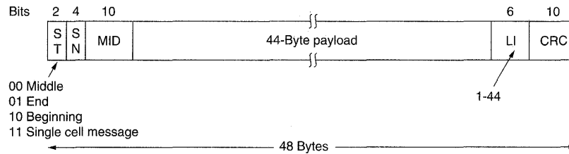
Fig. 6-43. The AAL 3/4 cell format.
