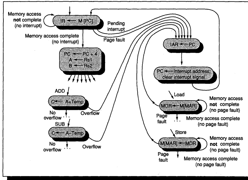
FIGURE 5.12 The top-level view of the DLX finite-state diagram (Figure 5.4 on page 207) modified to check for interrupts. Either a between interrupt or an instruction page fault invokes the control that saves the PC and then loads it with the address of the appropriate interrupt routine. The lower portion of the figure shows interrupts resulting in page faults of data accesses or arithmetic overflow.
