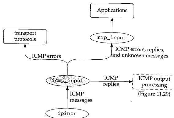
Figure 11.14 ICMP input processing.
