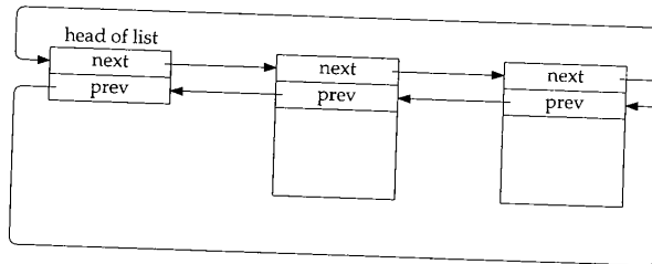
Figure 2.23 Doubly linked, circular list.
