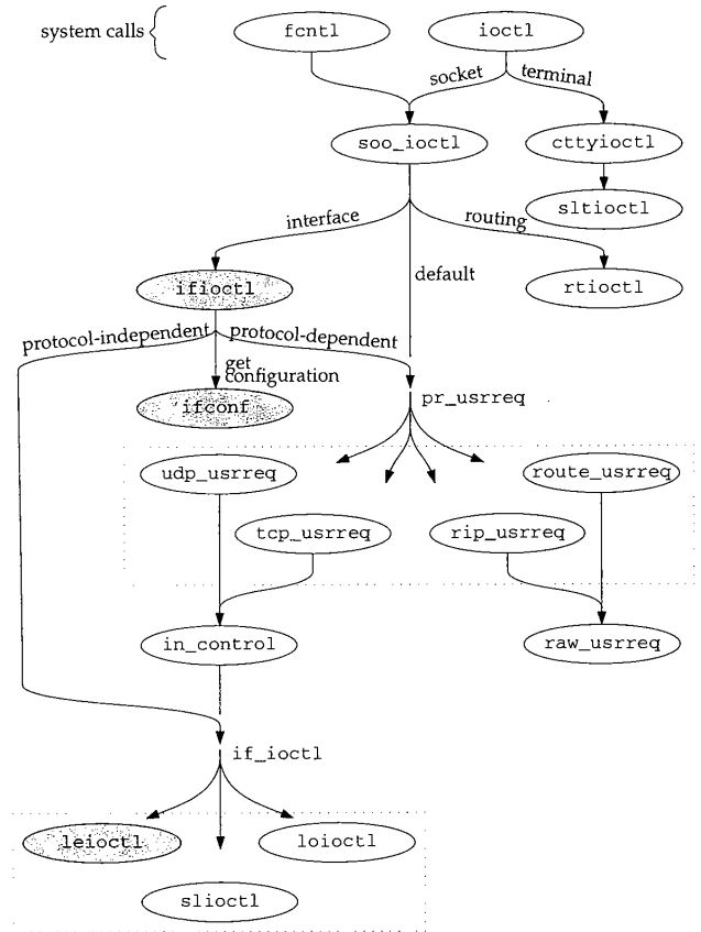
Figure 4.21 ioctl functions described in this chapter.
