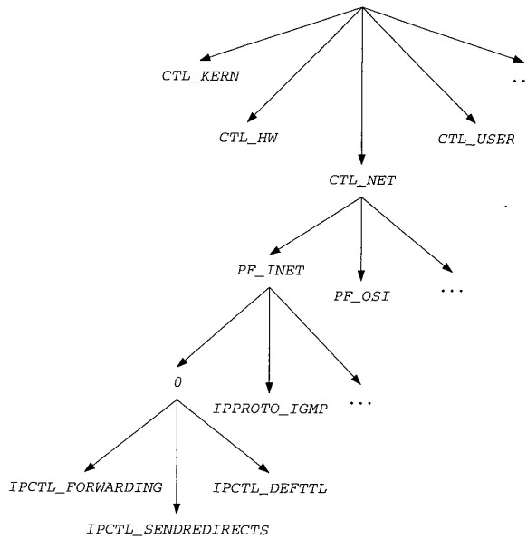
Figure 7.24 sysctl names.
