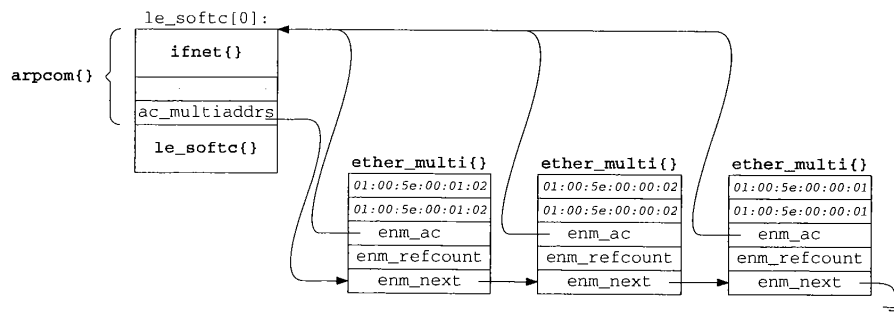
Figure 12.8 The LANCE interface with three ether_multi structures.
