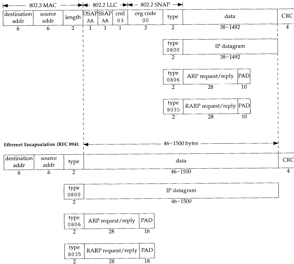
Figure 2.1 IEEE 802.2/802.3 encapsulation (RFC 1042) and Ethernet encapsulation (RFC 894).
