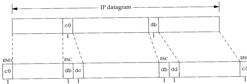
Figure 2.2 SLIP encapsulation.
