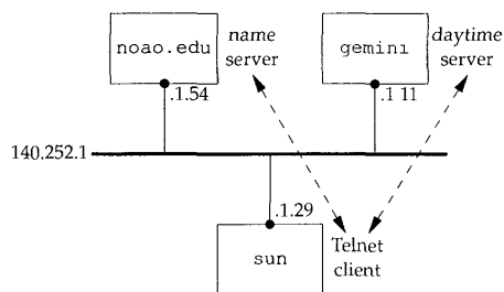
Figure 14.9 Systems being used for simple DNS example.
