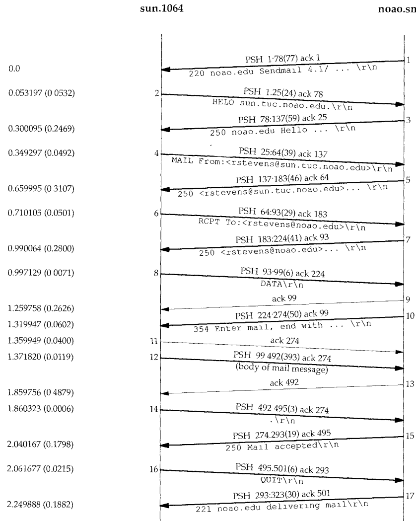
Figure 28.2 Basic SMTP mail delivery
