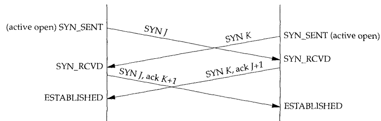
Figure 18.17 Segments exchanged during simultaneous open.
