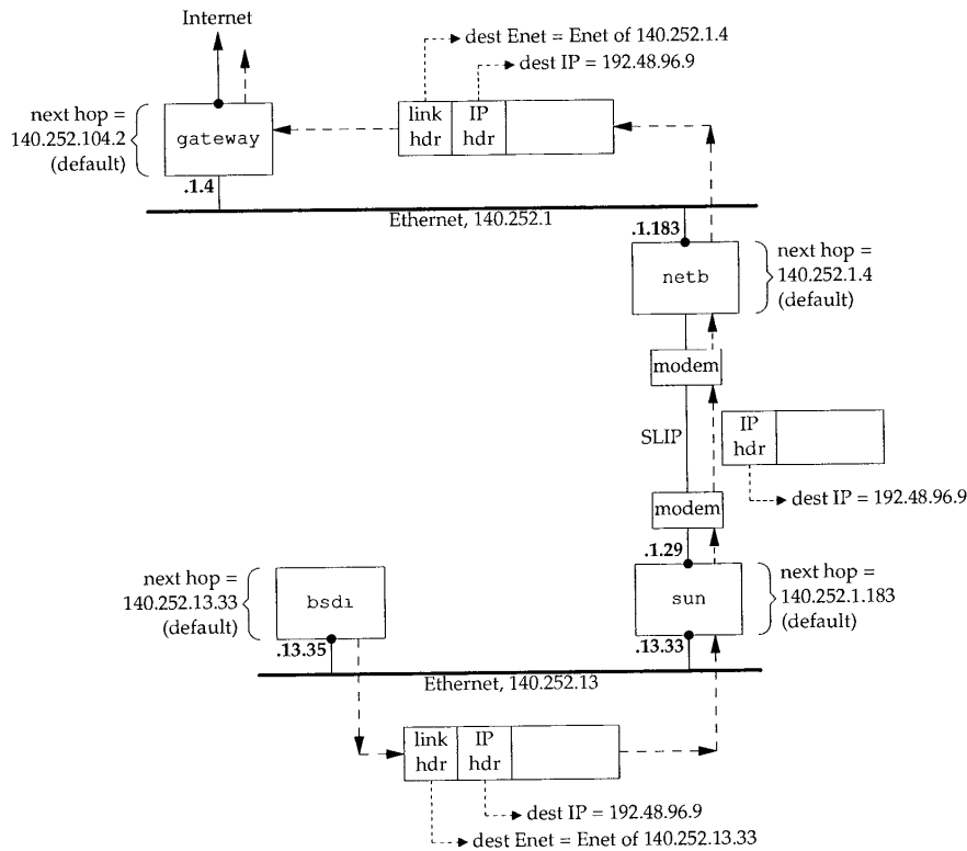
Figure 3.4 Initial path of datagram from bsdi to ftp.uu.net (192.48.96.9).
