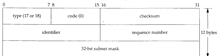
Figure 6.4 ICMP address mask request and reply messages.
