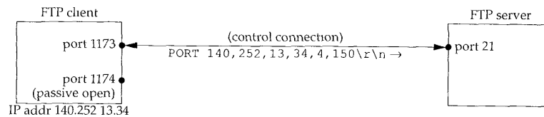
Figure 27.4 PORT command going across FTP control connection.
