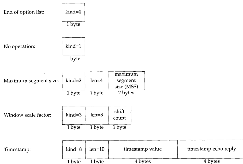
Figure 18.20 TCP options.
