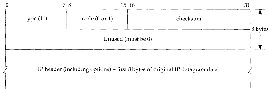
Figure 8.2 ICMP time exceeded message.
