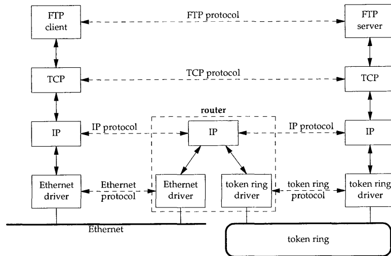
Figure 1.3 Two networks connected with a router.
