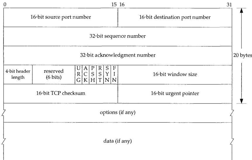
Figure 17.2 TCP header.
