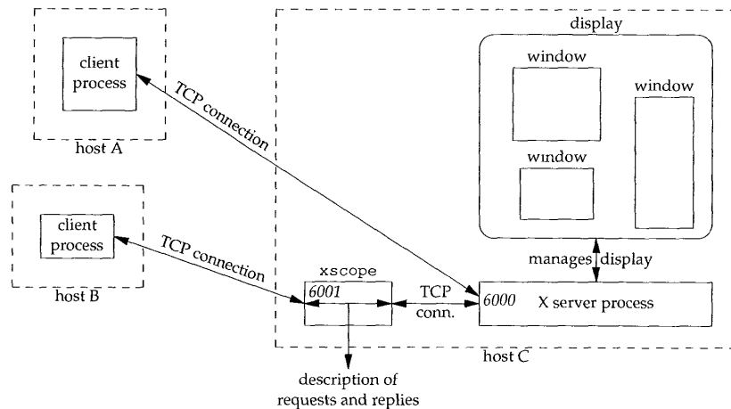
Figure 30.3 Using xscope to monitor an X connection.
