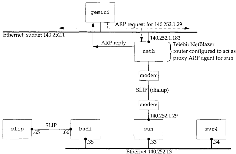
Figure 4.6 Example of proxy ARP.
