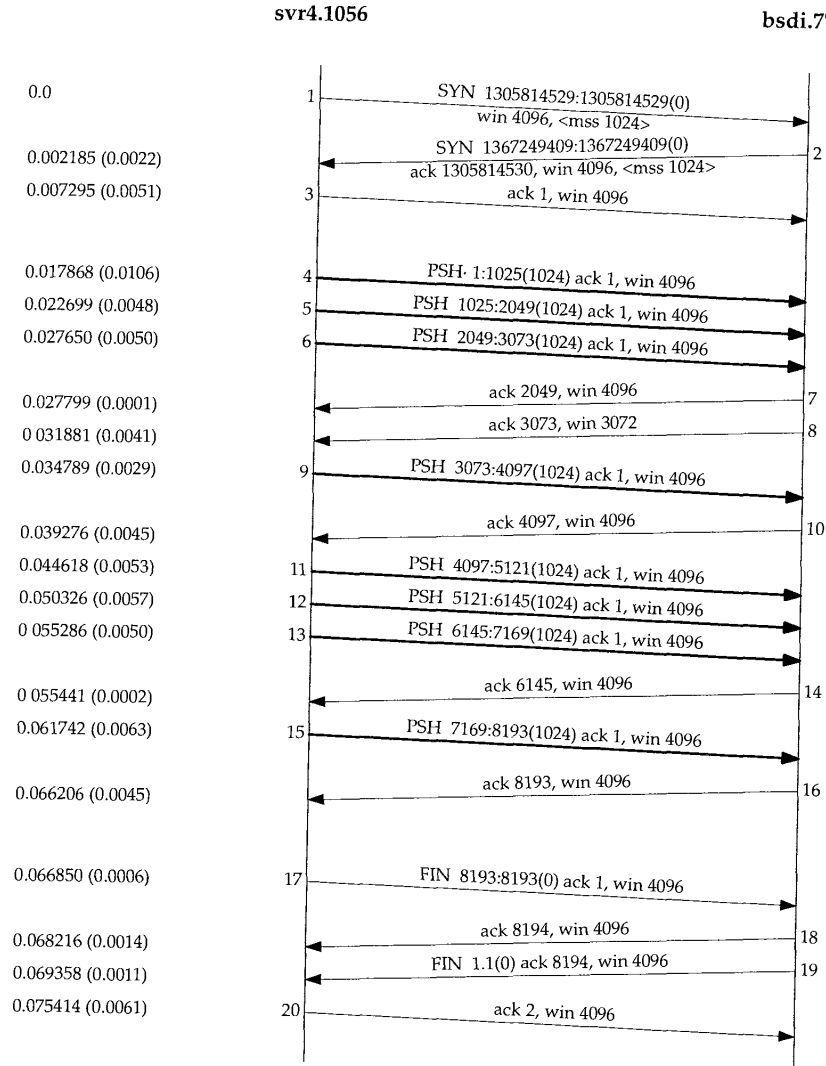
Figure 20.1 Transfer of 8192 bytes from svr4 to bsd1 .
