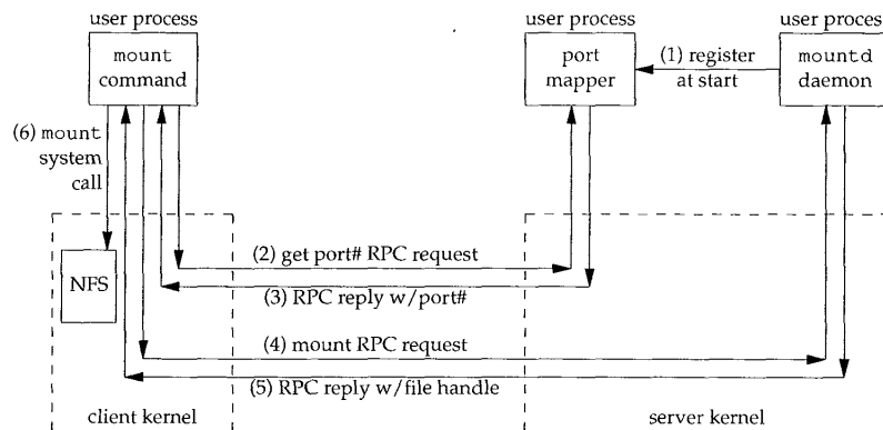
Figure 29.5 Mount protocol used by Unix mount command.
