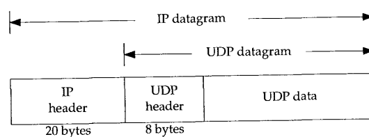
Figure 11.1 UDP encapsulation.
