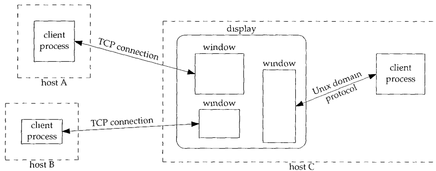
Figure 30.1 Three X clients using one display
