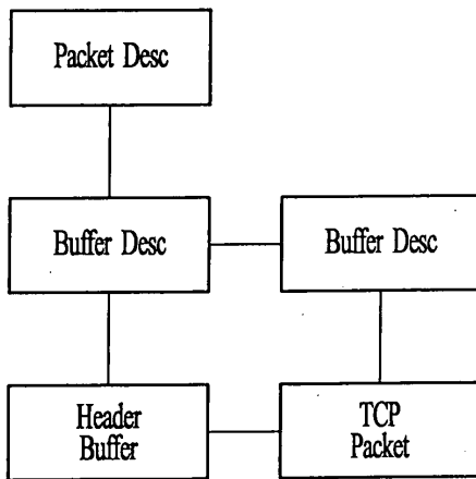
Example of incoming TCP pkt
