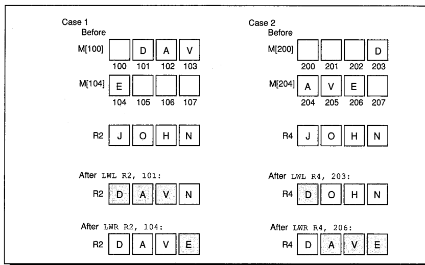
FIGURE E.9 MIPS instructions for unaligned word reads. This figure assumes operating in Big Endian mode. Case (1) first loads the 3 bytes 101, 102, and 103 into the left of R2 leaving the least significant byte undisturbed. The following LWR simply loads byte 104 into the least significant byte of R2 leaving the other bytes of the register unchanged using LWL . Case (2) first loads byte 203 into the most significant byte of R4 and the following LWR loads the other 3 bytes of R4 from memory bytes 204, 205, and 206. LWL reads the word with the first byte from memory, shifts to the left to discard the unneeded byte(s), and changes only those bytes in Rd. The byte(s) transferred are from the first byte until the lowest-order byte of the word. The following LWR addresses the last byte, right shifts to discard the unneeded byte(s), and finally changes only those bytes of Rd. The byte(s) transferred are from the last byte up to the highest-order byte of the word. Store word left ( SWL ) is simply the inverse of LWL , and store word right ( SWR ) is the inverse of LWR . Changing to Little Endian mode flips which bytes are selected and discarded. (If big/little–left/right–load/store seems confusing, don't worry, it works!)
