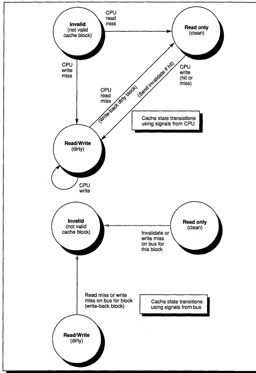
FIGURE 8.44 A write-invalidate, cache-coherency protocol. The upper part of the diagram shows state transitions based on actions of the CPU associated with this cache; the lower part shows state transitions based on operations on the bus. There is only one state machine in a cache, although there are two represented here to clarify when a transition occurs. The black arrows and states would be in a normal cache, with the gray arrows added to get cache coherency. In contrast to what is shown here, some protocols call writes to clean data a “write miss,” so that there is no separate signal for invalidation.
