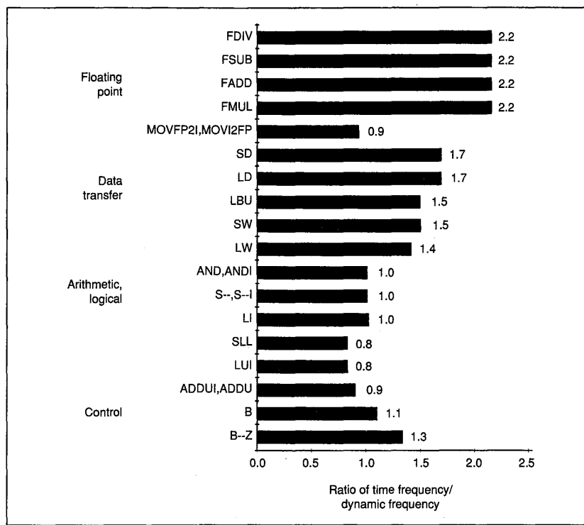
FIGURE D.7 Time frequency divided by execution frequency for DLX as measured using the time data from Figure D.6 and the frequency data from Figure 4.34 (page 181). The integer register–floating-point register moves are inexpensive, since they are really register–register operations. Surprisingly, the double-precision memory references are not twice as expensive as the 32-bit loads and stores. Can you hypothesize why based on the discussions of pipelining and cache design?
