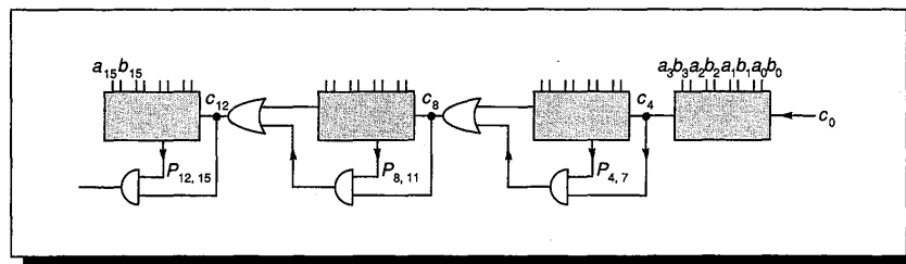
FIGURE A.15 Carry-skip adder.
