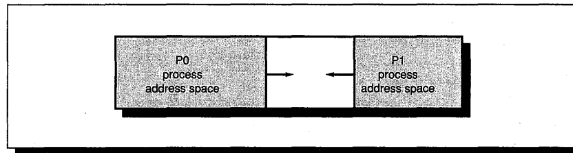
FIGURE 8.26 The organization of P0 and P1 in the VAX. This is the process half of the address space, selected with a 0 in bit 31 of a virtual address. Bit 30 of the address divides P0 and P1. Operating systems put the text and heap areas into P0 and a downward growing stack into P1.
