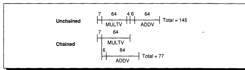
FIGURE 7.14 Timings for a sequence of dependent vector operations ADDV and MULTV, both unchained and chained. The 4-clock-cycle delay comes from a stall for dependence, described earlier; the 6- and 7-clock-cycle delays are the latency of the adder and multiplier.
