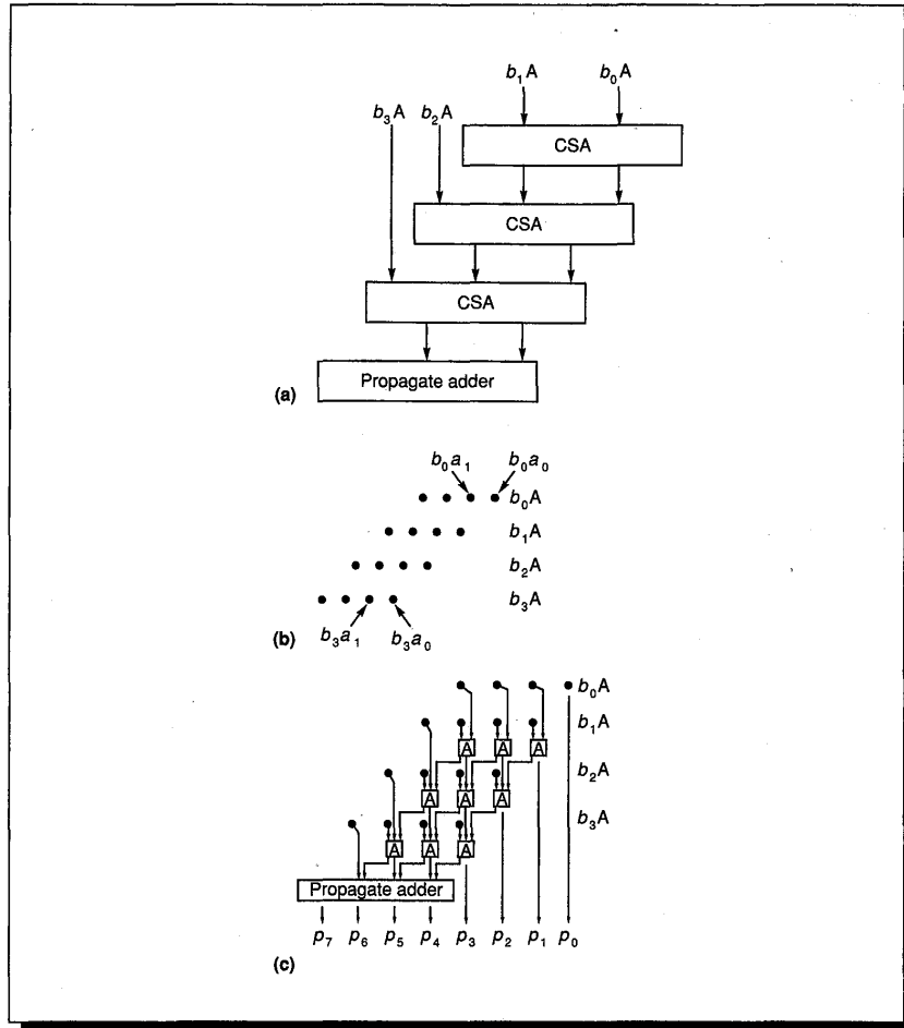
FIGURE A.26 Block diagram of an array multiplier (a); the inputs to the array (b); the array expanded to show all the adders (c).
