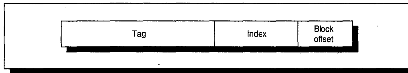
FIGURE 8.8 The 3 portions of an address in a set-associative or direct-mapped cache. The tag is used to check all the blocks in the set and the index is used to select the set. The block offset is the address of the desired data within the block.
