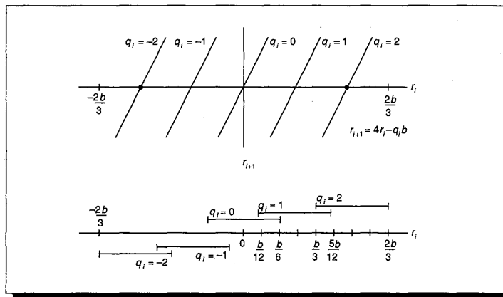
FIGURE A.29 Quotient selection for radix-4 division.
