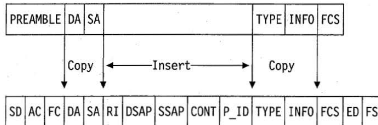
Figure 5-15. 8229 TCP/IP Support. Conversion process.
