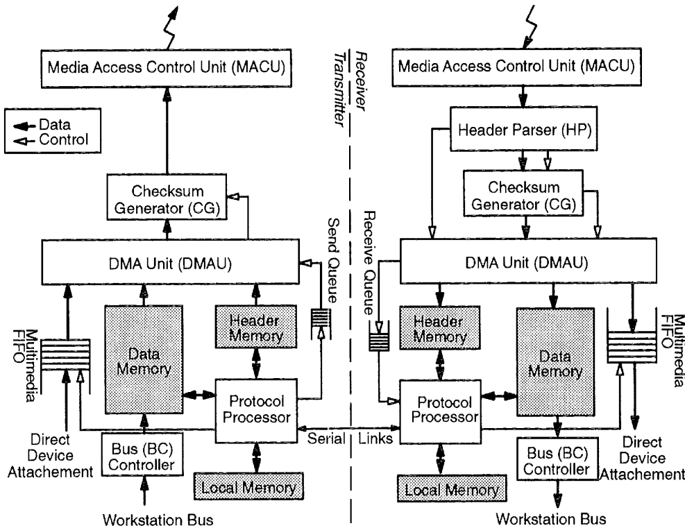
Figure 1. MPA Architecture
