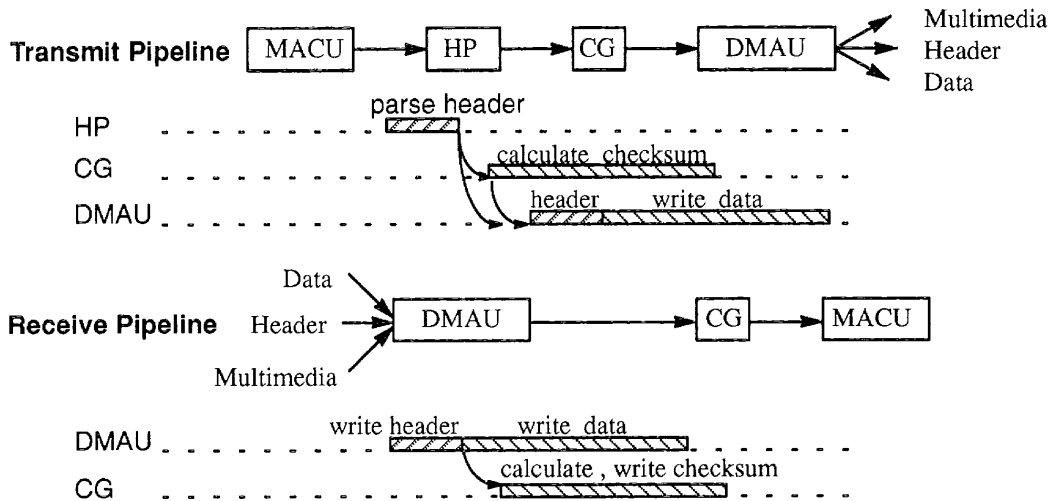
Figure 2. Pipelined Packet Processing
