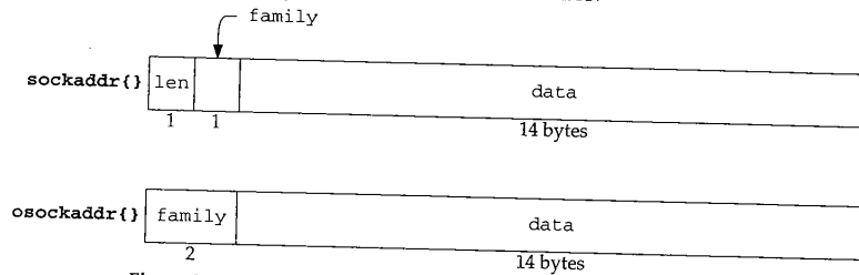
Figure 3.18 sockaddr and osockaddr structures (sa_ prefix dropped).
