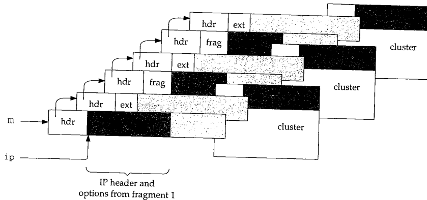
Figure 10.28 The reassembled datagram.
