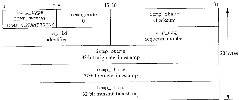
Figure 11.22 ICMP timestamp request and reply.
