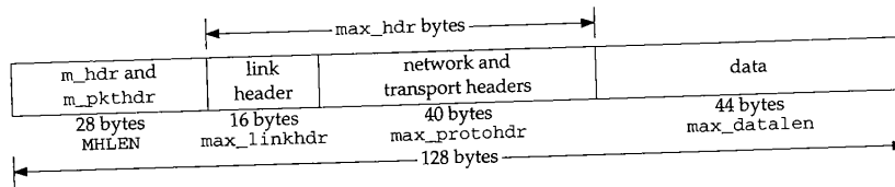
Figure 7.18 Mbuf and associated maximum header lengths.
