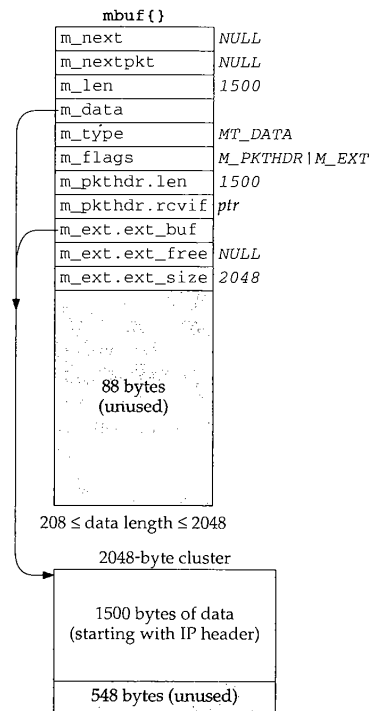
Figure 2.16 Fourth type of mbuf created by m_devget .
