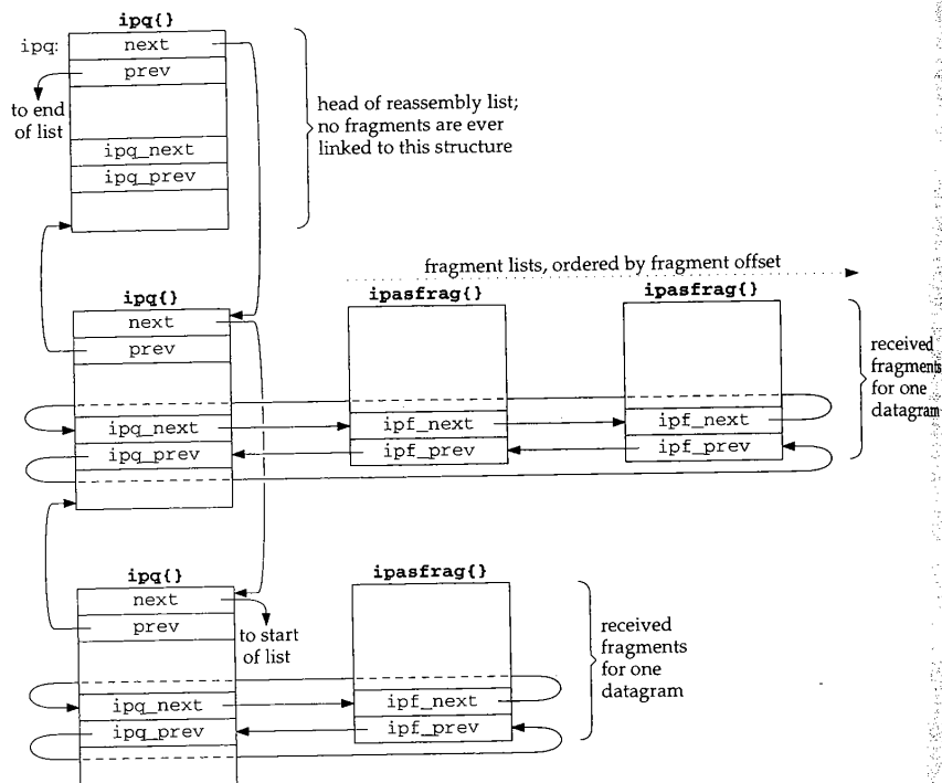
Figure 10.15 The fragment header list, ipq , and fragments.
