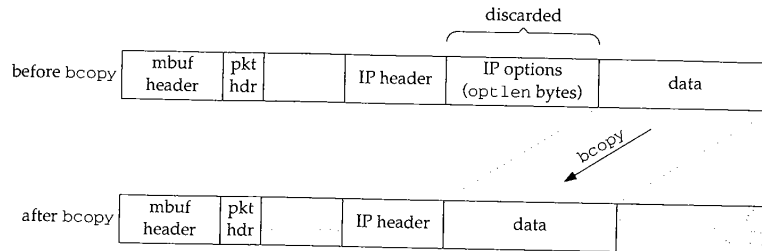
Figure 11.38 icmp_reflect: removal of options.
