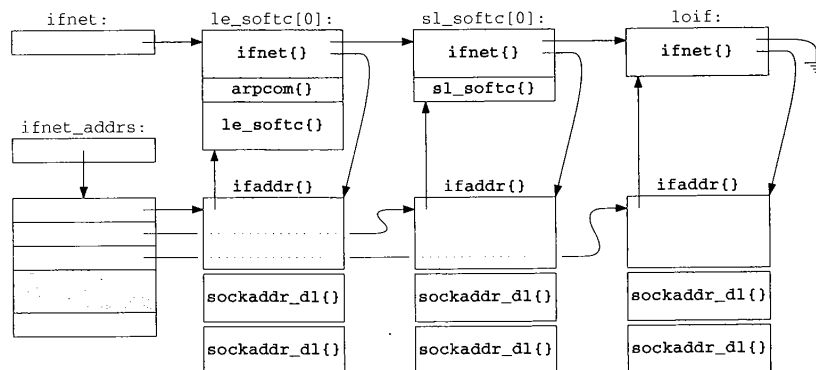
Figure 4.27 Interface and address data structures.
