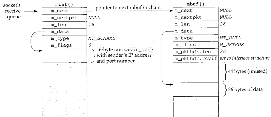
Figure 1.11 Sender's address and data.
