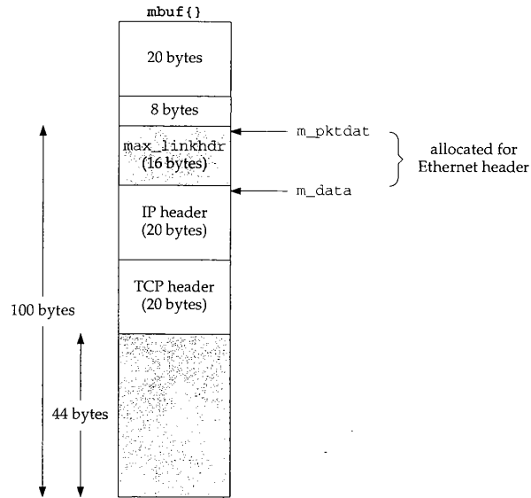
Figure 9.29 ip_insertoptions function: TCP segment.
