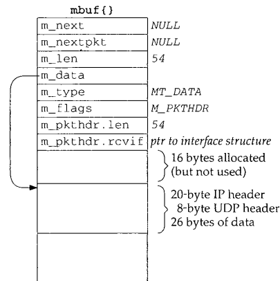
Figure 1.10 Single mbuf to hold input Ethernet data.
