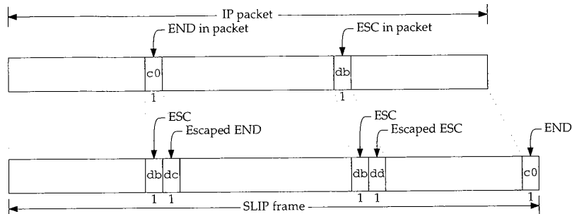
Figure 5.5 SLIP encapsulation of an IP packet.
