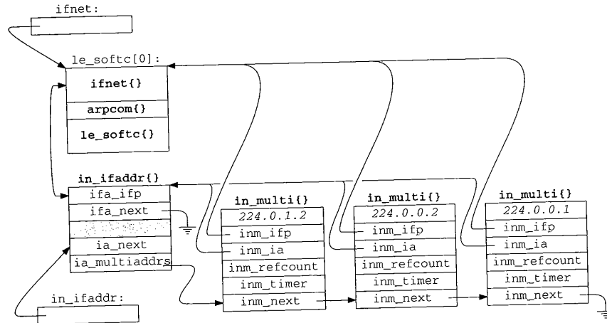
Figure 12.13 An IP multicast group list for the le interface.
