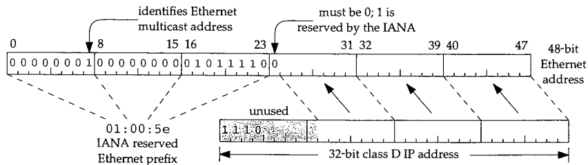
Figure 12.5 Mapping between IP and Ethernet addresses.
