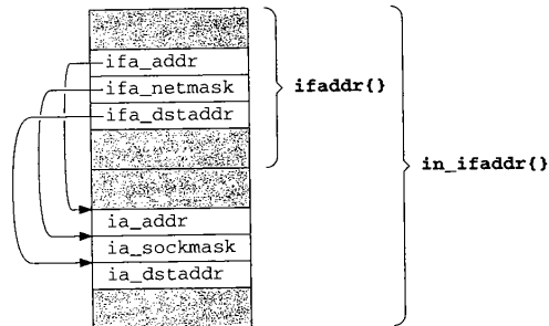
Figure 6.15 An in_ifaddr structure after initialization by in_control .
