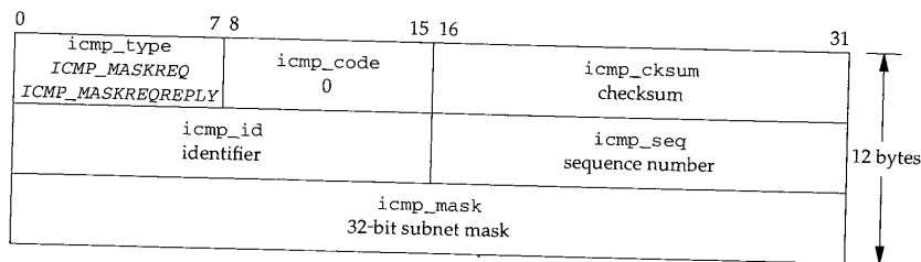
Figure 11.24 ICMP address mask request and reply.
