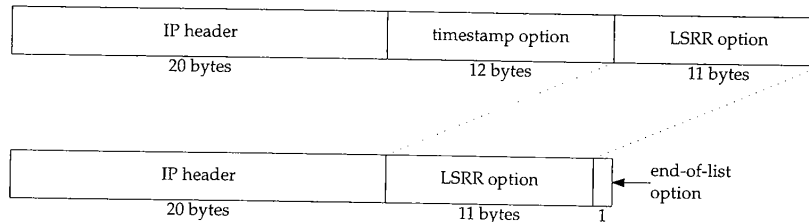
Figure 10.10 Not all options are copied during fragmentation.
