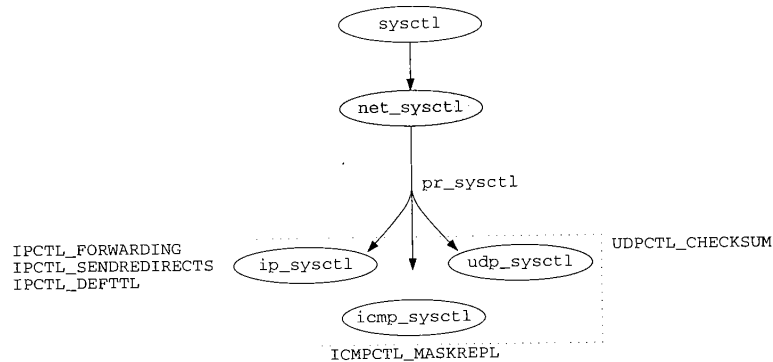
Figure 7.25 sysctl functions for Internet parameters.
