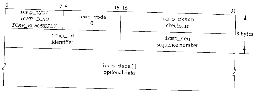
Figure 11.20 ICMP echo request and reply.
