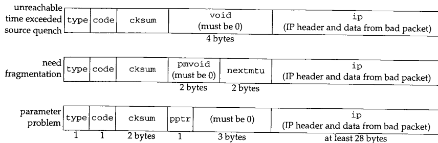
Figure 11.17 ICMP error messages (icmp_omitted).
