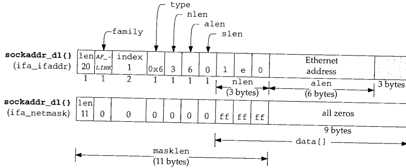
Figure 3.38 The initialized Ethernet sockaddr_dl structures ( sdl_prefix omitted).
