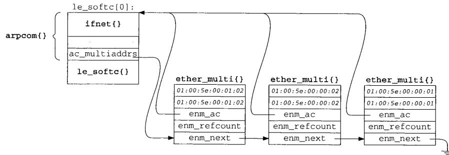
Figure 12.8 The LANCE interface with three ether_multi structures.
