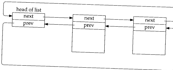
Figure 2.23 Doubly linked, circular list.
