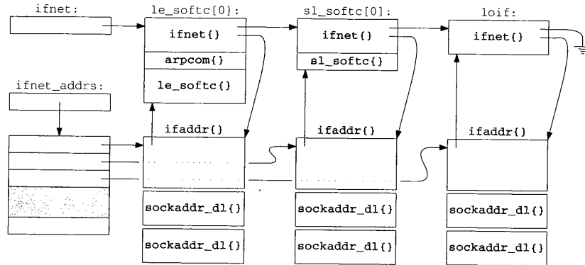
Figure 3.32 ifnet list.
