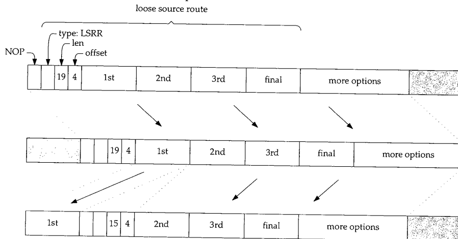
Figure 9.33 ip_pcbopts option list processing.
