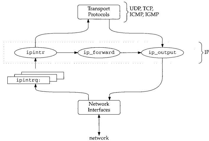
Figure 8.1 IP layer processing.
