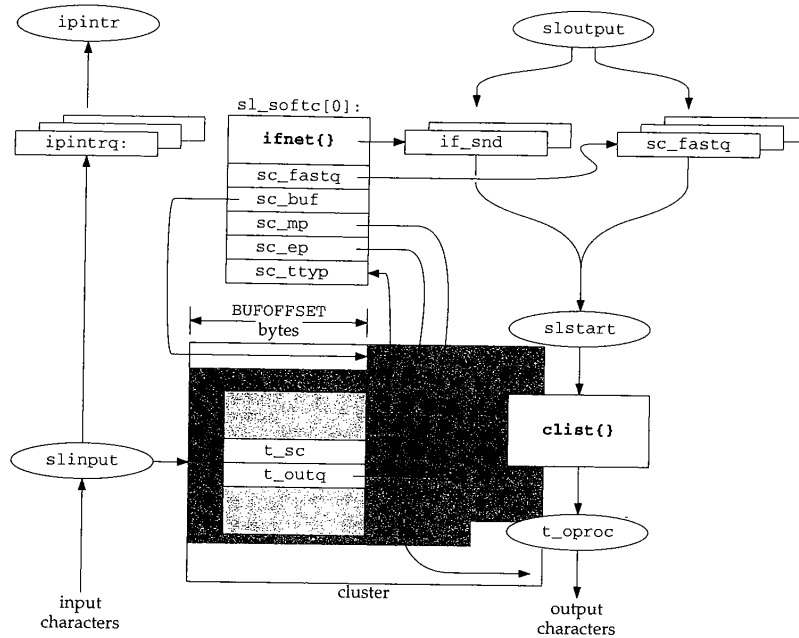
Figure 5.8 SLIP device driver.
