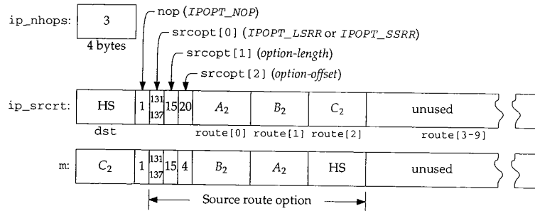
Figure 9.20 ip_srcroute reverses the route in ip_srcrt.
