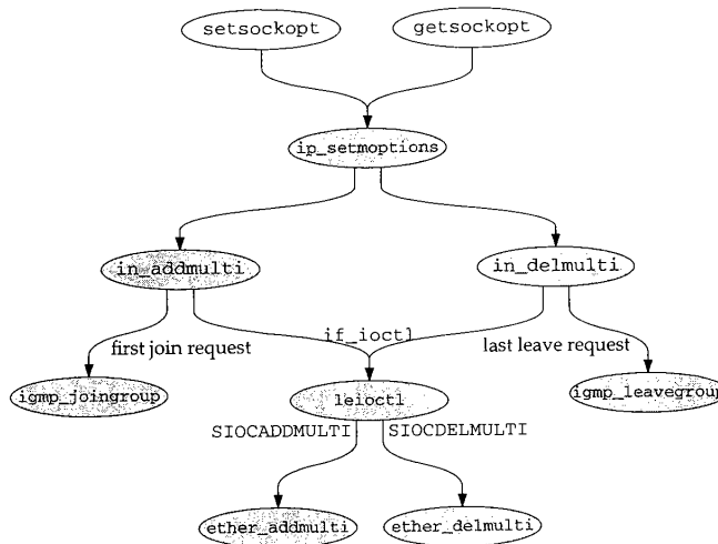
Figure 12.25 Joining and leaving a multicast group.
