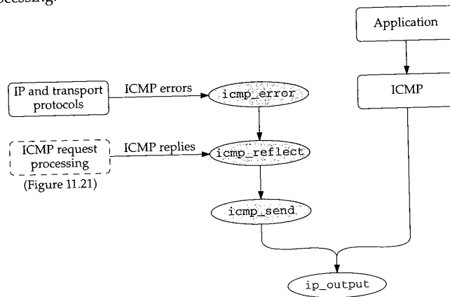
Figure 11.29 ICMP output processing.
