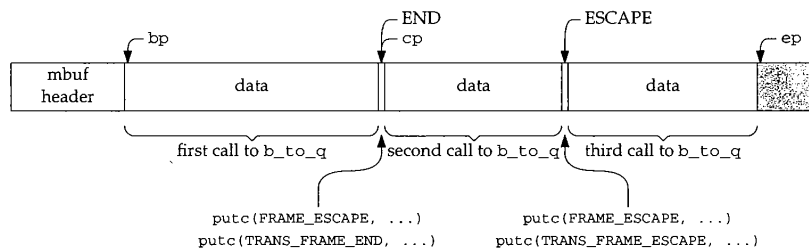
Figure 5.21 SLIP transmission of a single mbuf.
