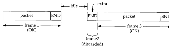
Figure 5.19 Karn's method with no noise.
