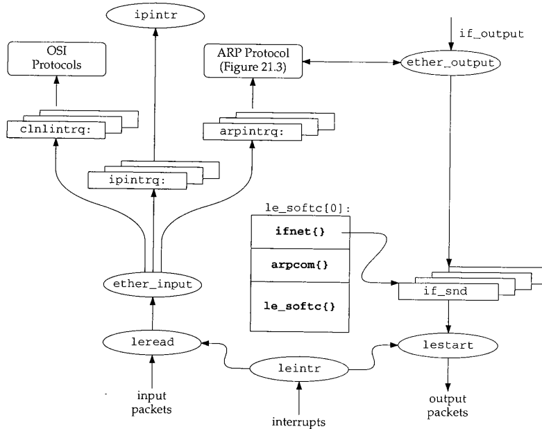
Figure 4.9 Ethernet device driver.
