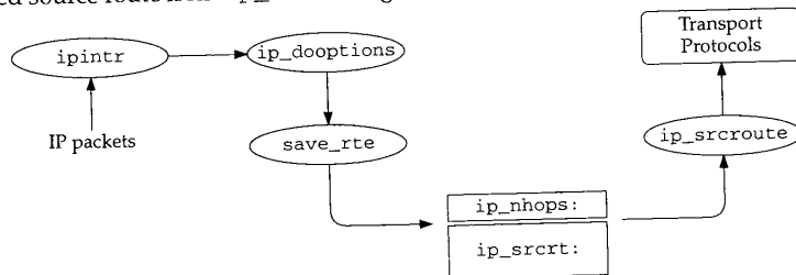
Figure 9.17 Processing of reversed source routes.
