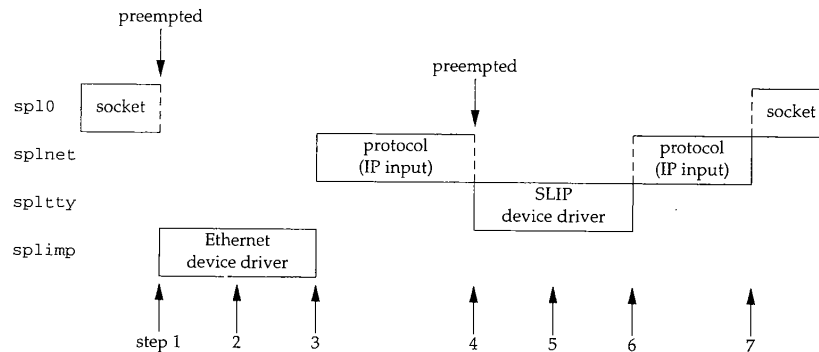
Figure 1.14 Example of priority levels and kernel processing.
