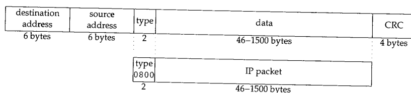
Figure 4.8 Ethernet encapsulation of an IP packet.
