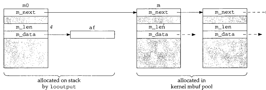
Figure 5.29 BPF loopback packet: mbuf format.
