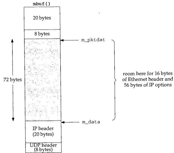
Figure 9.31 ip_insertoptions function: UDP datagram.
