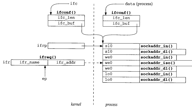
Figure 4.25 ifconf data structures.
