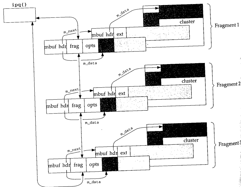
Figure 10.27 m_cat reassembles the fragments within mbufs.
