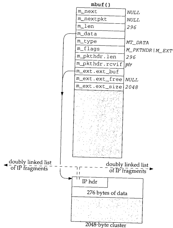
Figure 2.17 An IP fragment of length 296.
