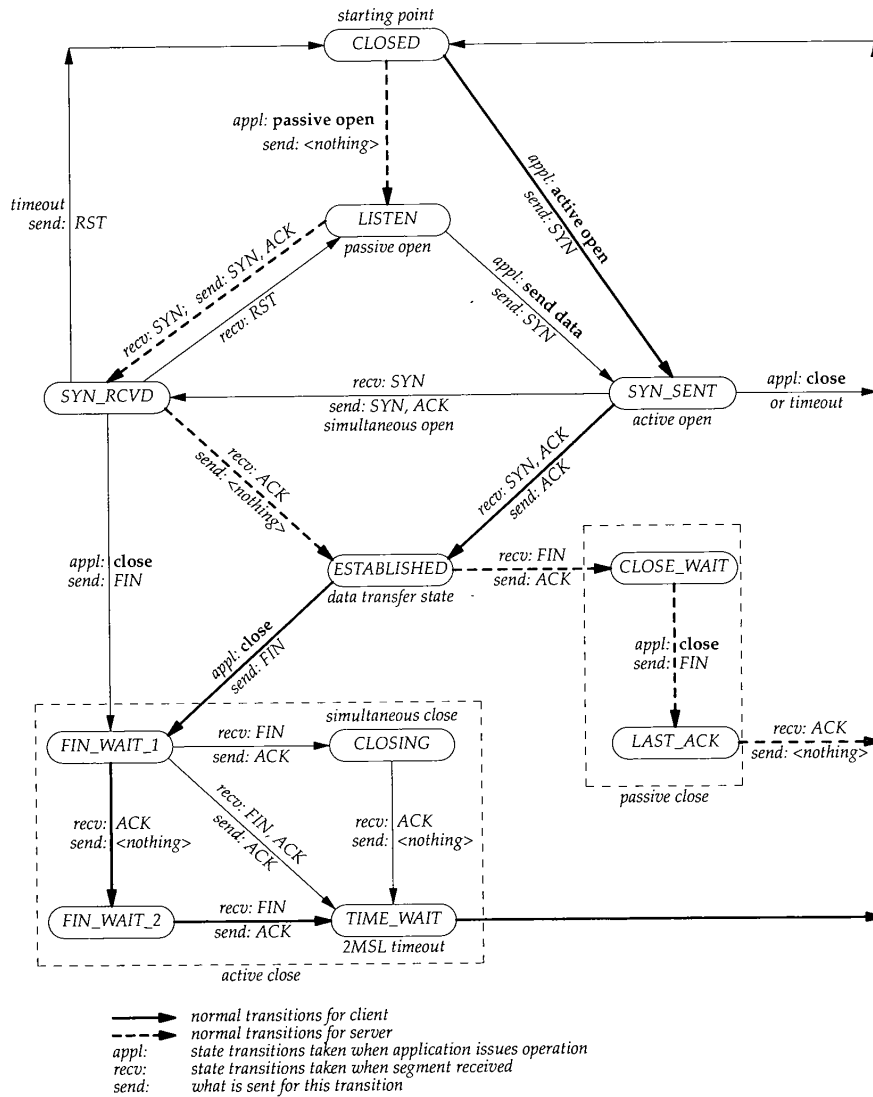
TCP state transition diagram.
