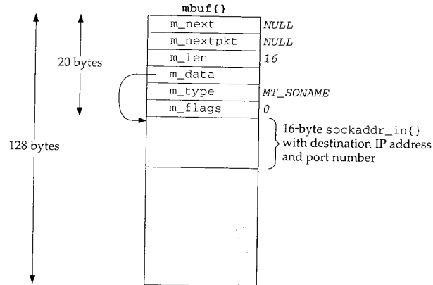
Figure 1.6 Mbuf containing destination address for sendto .
