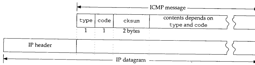
Figure 11.11 An ICMP message ( icmp_omitted ).
