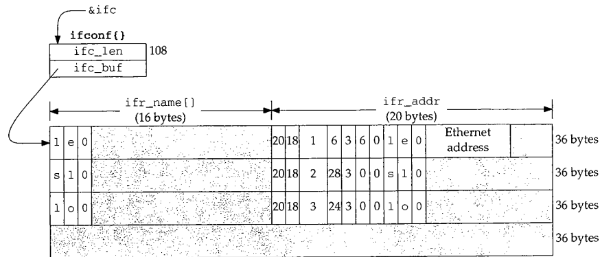
Figure 4.28 Data returned by the SIOCGIFCONF command.
