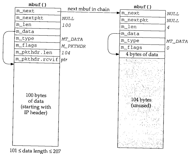
Figure 2.15 Third type of mbuf created by m_devget .
