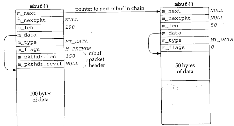
Figure 1.7 Two mbufs holding 150 bytes of data.
