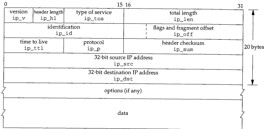
Figure 8.8 IP datagram, including the ip structure names.
