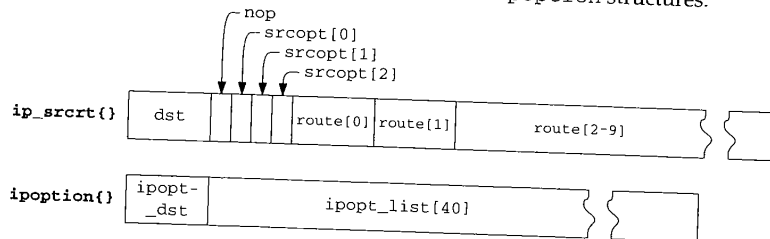
Figure 9.27 The ip_srcrt and ipoption structures.
