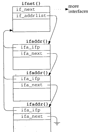
Figure 3.16 ifnet and ifaddr structures.
