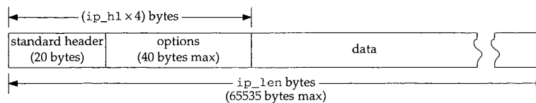
Figure 8.10 Organization of an IP packet with options.
