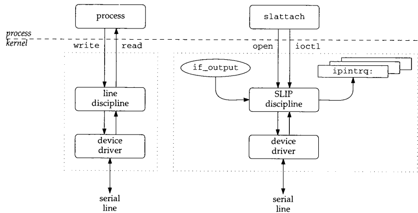
Figure 5.6 The SLIP interface as a line discipline.
