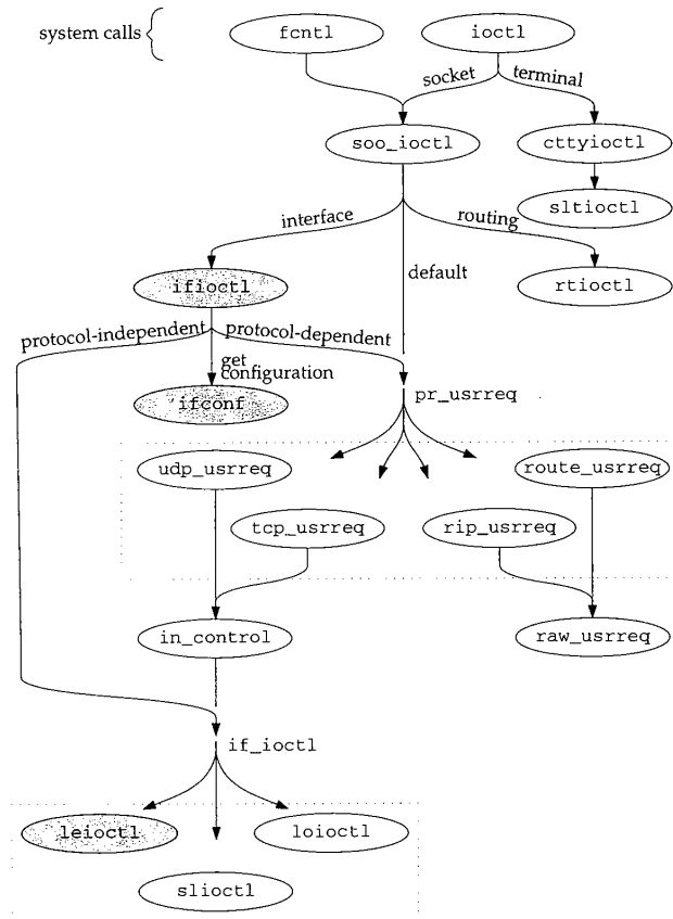
Figure 4.21 ioctl functions described in this chapter.
