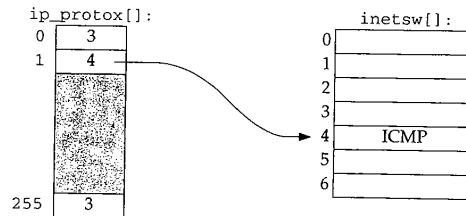
Figure 11.13 An ip_p value of 1 selects inetsw[4] .
