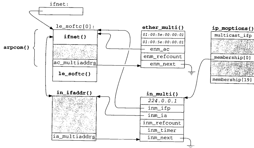
Figure 12.34 Overview of multicast data structures.
