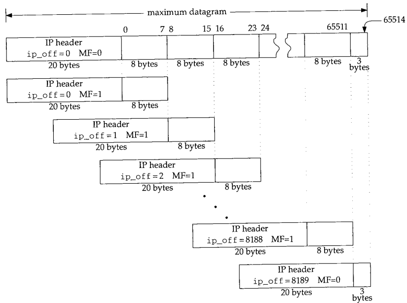
Figure 10.2 Fragmentation of a 65535-byte datagram.
