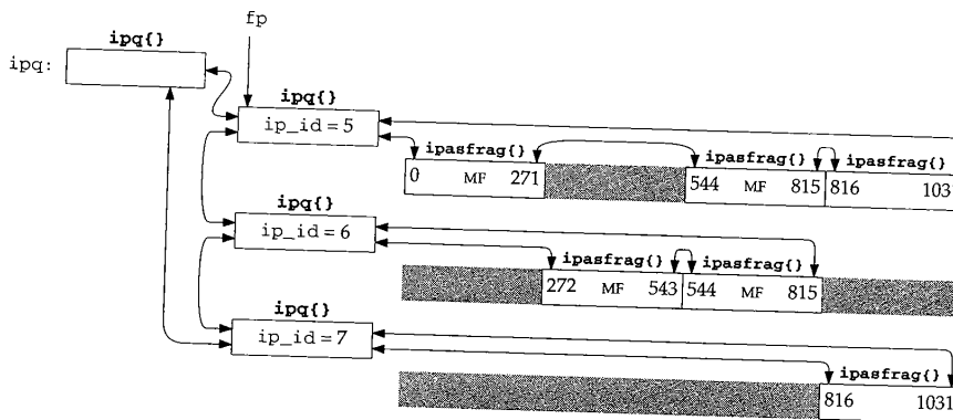
Figure 10.17 Reassembly of three IP datagrams.
