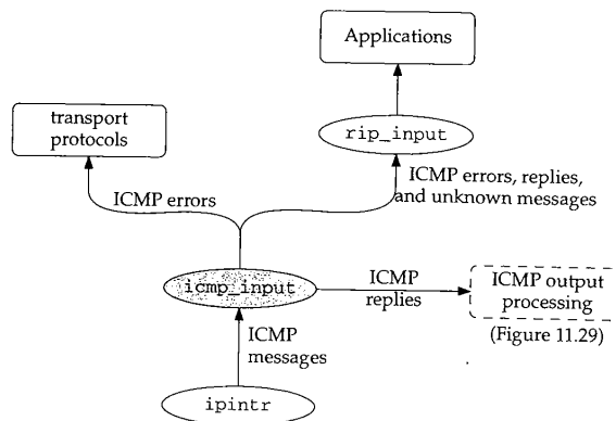
Figure 11.14 ICMP input processing.
