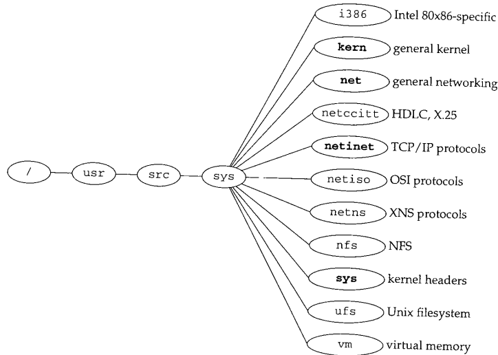
Figure 1.15 Net/3 source code organization.
