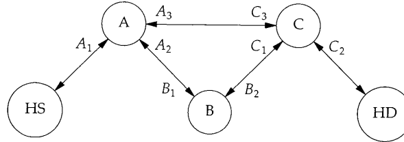
Figure 9.12 Source route example.
