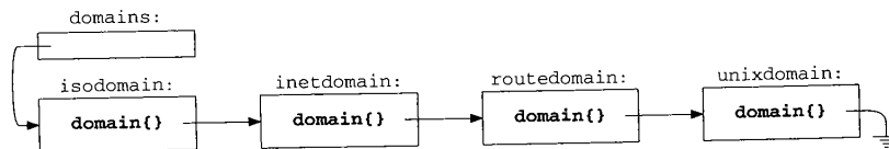
Figure 7.6 domains list.
