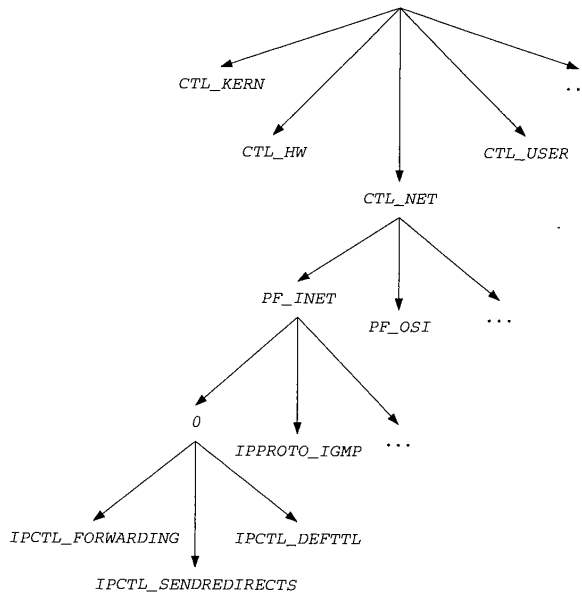
Figure 7.24 sysctl names.
