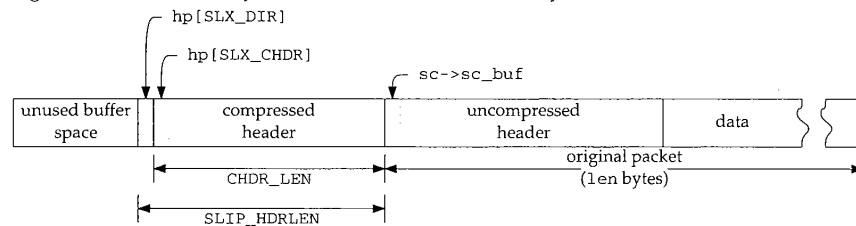
Figure 5.14 SLIP packet in BPF format.
