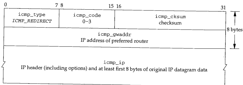
Figure 11.26 ICMP redirect message.
