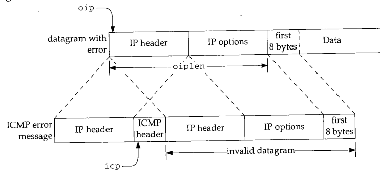
Figure 11.31 The construction of an ICMP error message.
