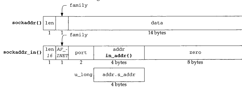
Figure 6.7 The organization of a sockaddr_in structure ( sin_omitted ).
