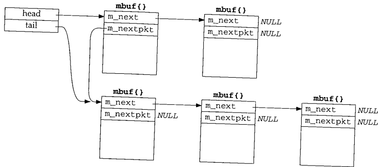
Figure 2.22 Linked list with head and tail pointers.
