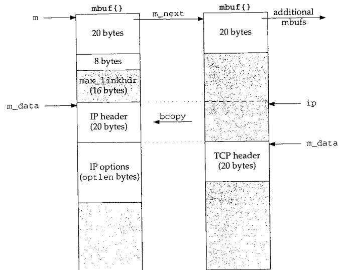
Figure 9.30 ip_insertoptions function: TCP segment, after options have been copied.
