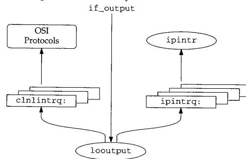
Figure 5.26 Loopback device driver.
