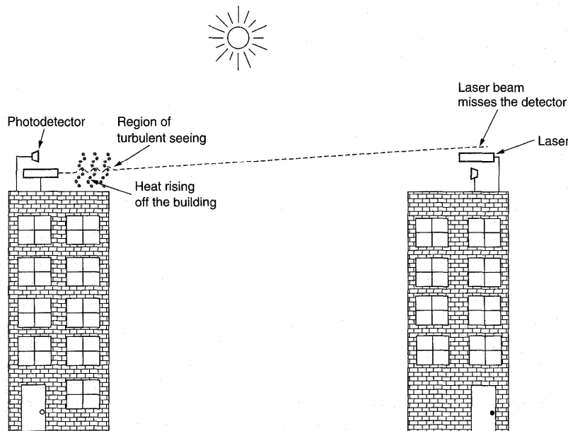
Fig. 2-13. Convection currents can interfere with laser communication systems. A bidirectional system, with two lasers, is pictured here.
