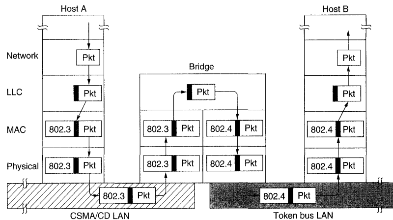
Fig. 4-35. Operation of a LAN bridge from 802.3 to 802.4.
