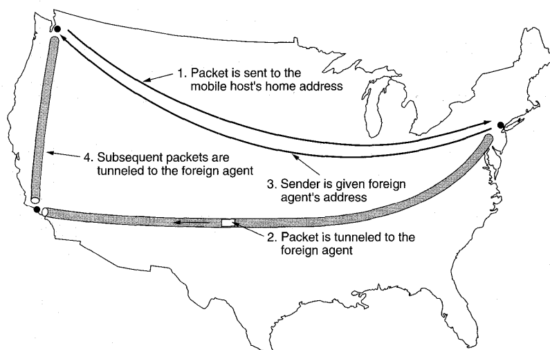
Fig. 5-19. Packet routing for mobile users.
