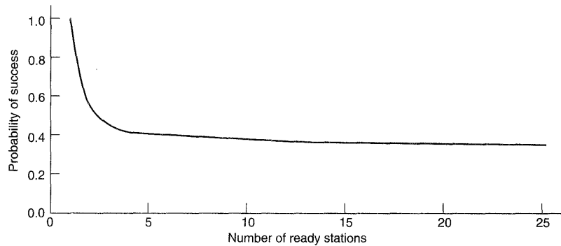
Fig. 4-8. Acquisition probability for a symmetric contention channel.
