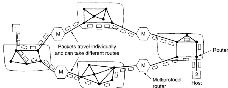
Fig. 5-37. A connectionless internet.
