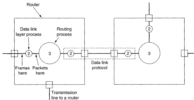
Fig. 3-2. Placement of the data link protocol.
