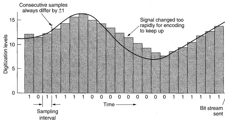
Fig. 2-27. Delta modulation.
