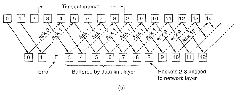
Fig. 3-15. (a) Effect of an error when the receiver window size is 1. (b) Effect of an error when the receiver window size is large.
