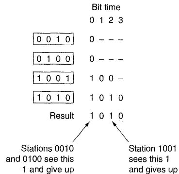
Fig. 4-7. The binary countdown protocol. A dash indicates silence.
