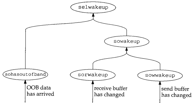
Figure 16.59 selwakeup processing.
