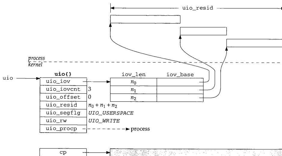
Figure 16.19 uiomove: before.
