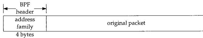
Figure 5.28 BPF loopback packet: logical format.
