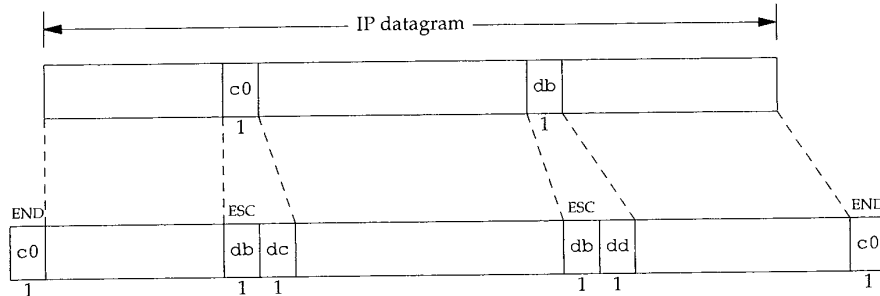
Figure 2.2 SLIP encapsulation.
