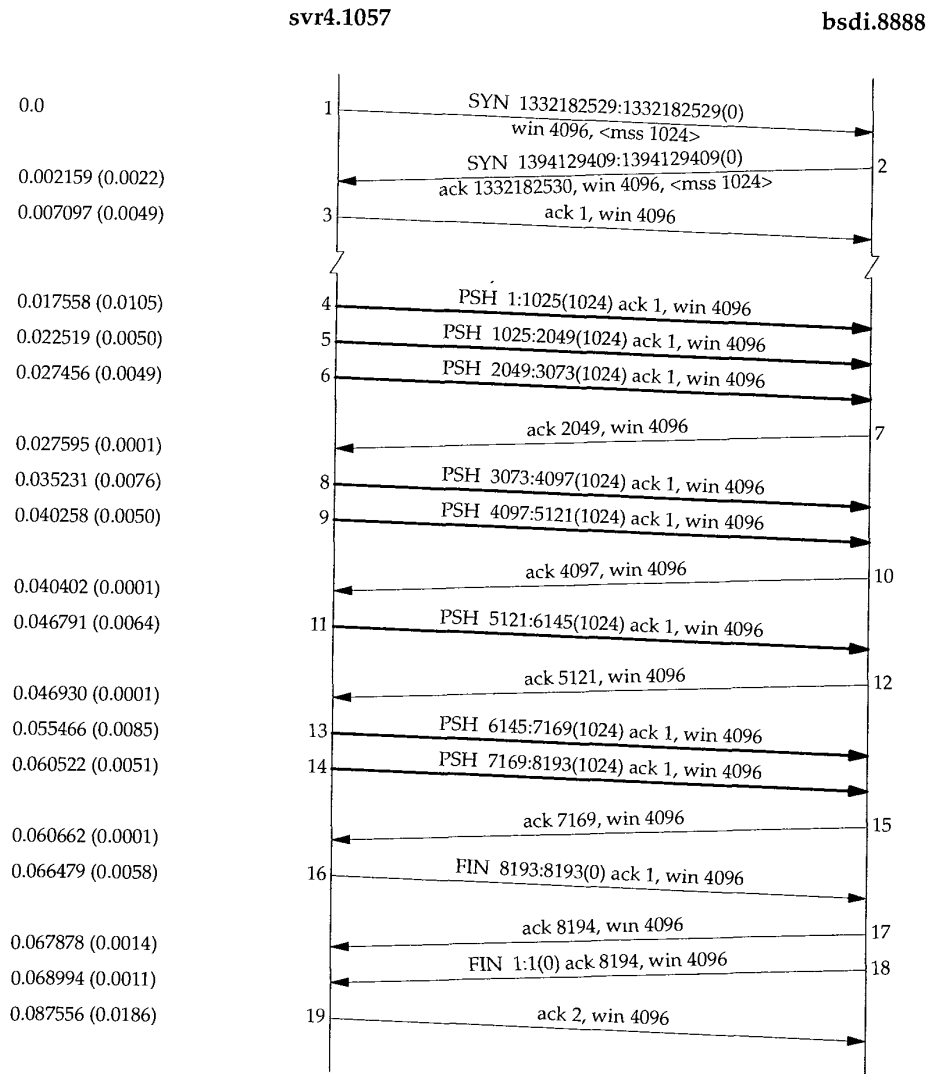
Figure 20.2 Another transfer of 8192 bytes from svr4 to bsd.
