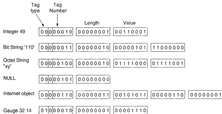
Fig. 7-34. ASN.1 encoding of some example values.
