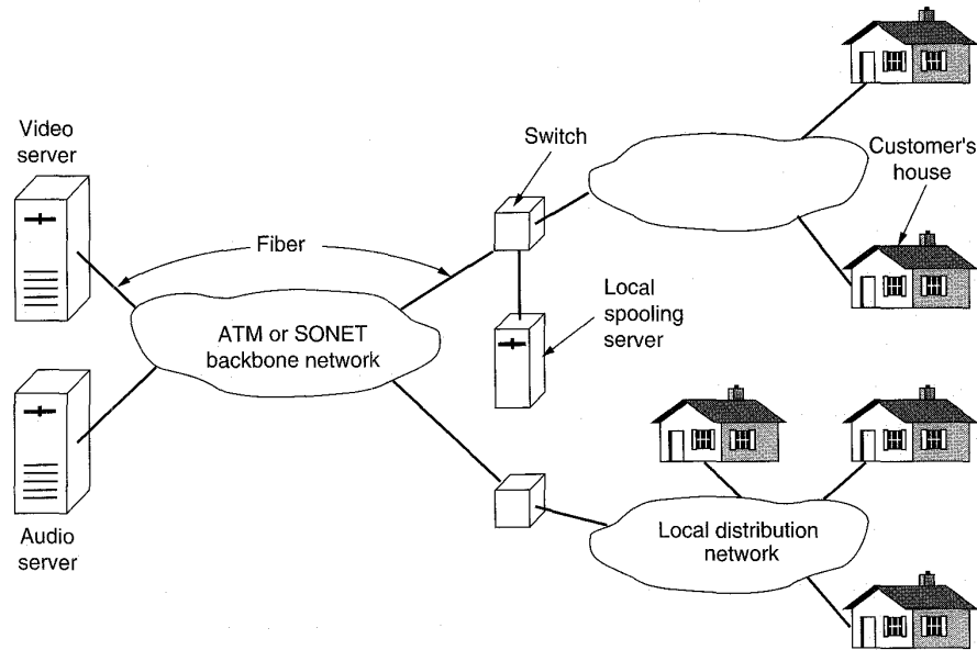
Fig. 7-88. Overview of a video-on-demand system.
