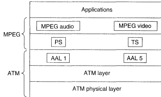
Fig. 7-93. A video-on-demand protocol stack.
