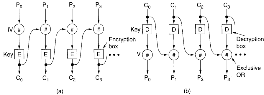
Fig. 7-7. Cipher block chaining
