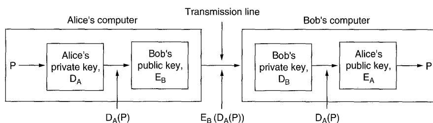
Fig. 7-23. Digital signatures using public-key cryptography.
