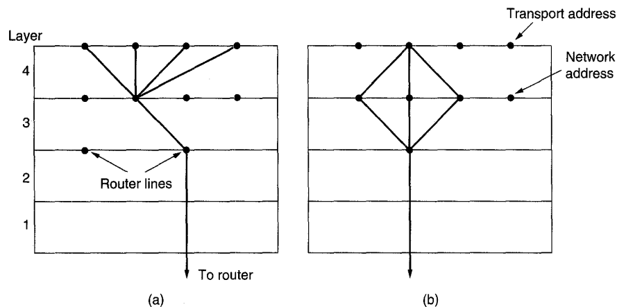
Fig. 6-17. (a) Upward multiplexing. (b) Downward multiplexing.
