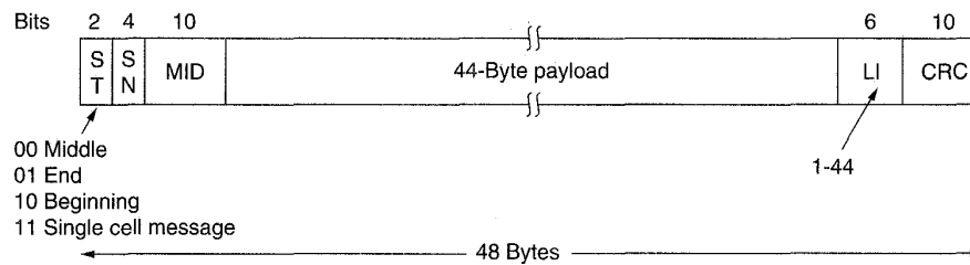
Fig. 6-43. The AAL 3/4 cell format.
