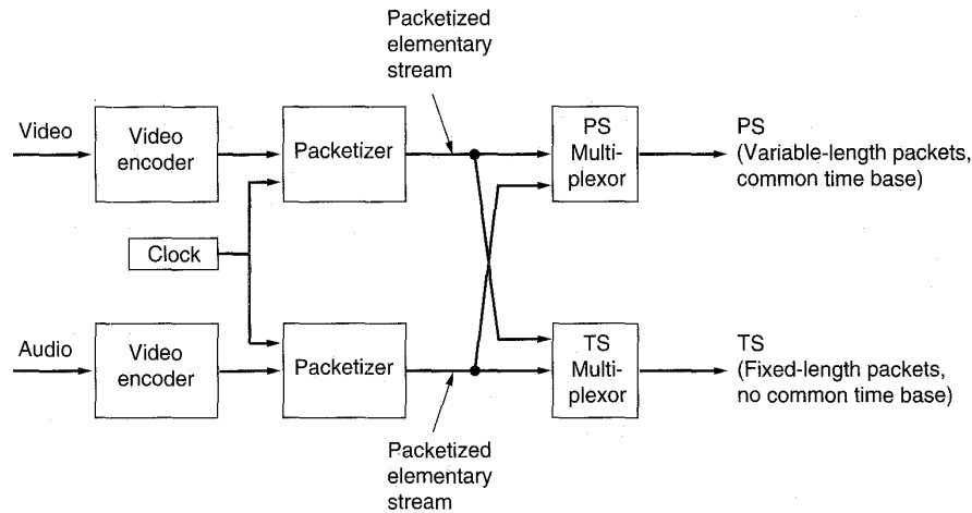
Fig. 7-87. Multiplexing of two streams in MPEG-2.
