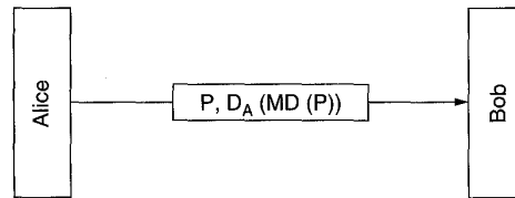
Fig. 7-24. Digital signatures using message digests.
