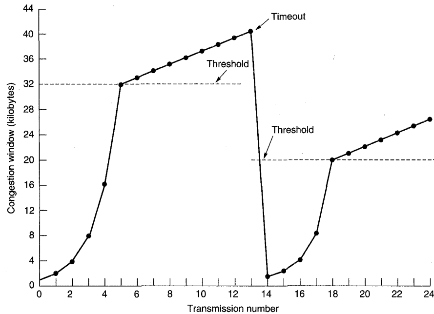
Fig. 6-32. An example of the Internet congestion algorithm.
