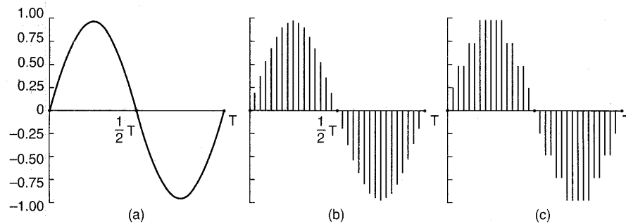
Fig. 7-76. (a) A sine wave. (b) Sampling the sine wave. (c) Quantizing the samples to 3 bits.
