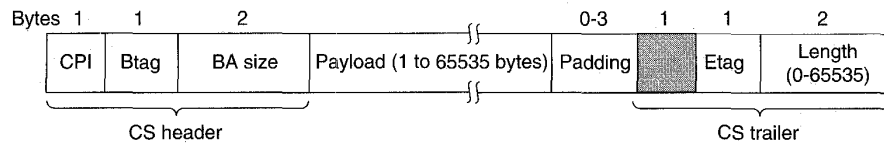
Fig. 6-42. AAL 3/4 convergence sublayer message format.
