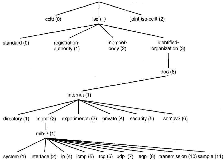
Fig. 7-32. Part of the ASN.1 object naming tree.
