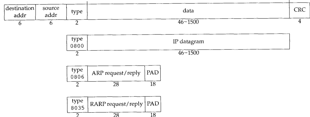
Figure 2.1 IEEE 802.2/802.3 encapsulation (RFC 1042) and Ethernet encapsulation (RFC 894).
