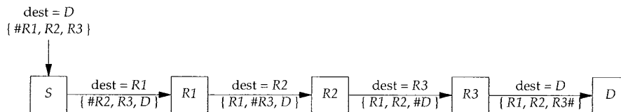
Figure 8.7 Example of IP source routing.
