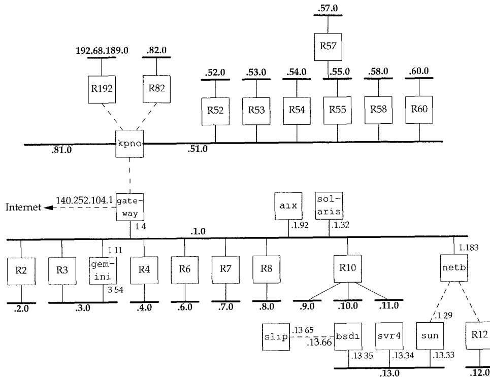
Figure 3.6 Arrangement of most of the noao.edu 140.252 subnets.
