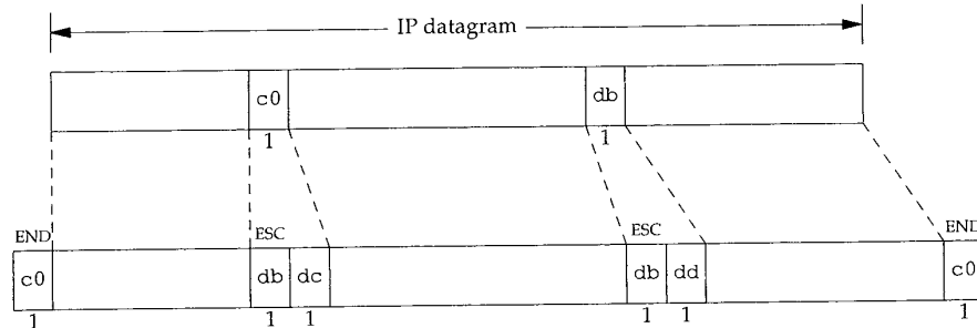
Figure 2.2 SLIP encapsulation.
