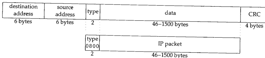
Figure 4.8 Ethernet encapsulation of an IP packet.
