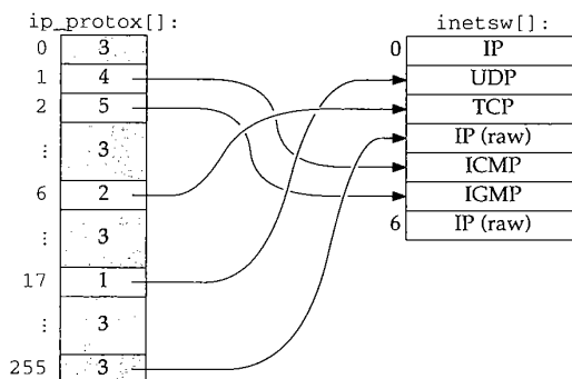
Figure 7.22 The ip_protosw array maps the protocol number to an entry in the inet_sw array.
