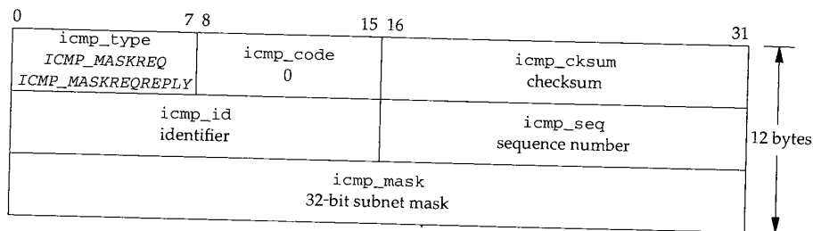
Figure 11.24 ICMP address mask request and reply.
