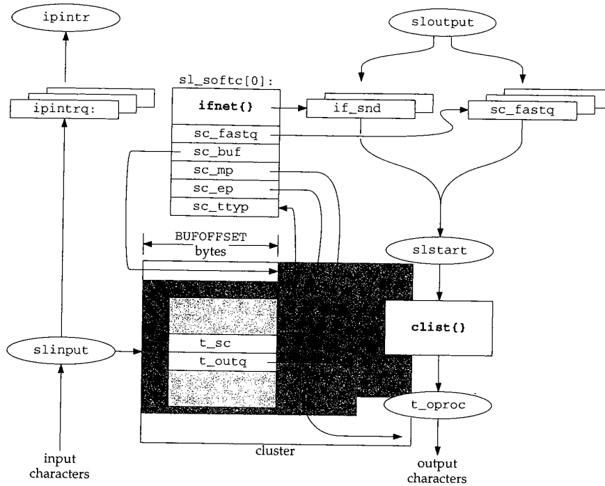
Figure 5.8 SLIP device driver.
