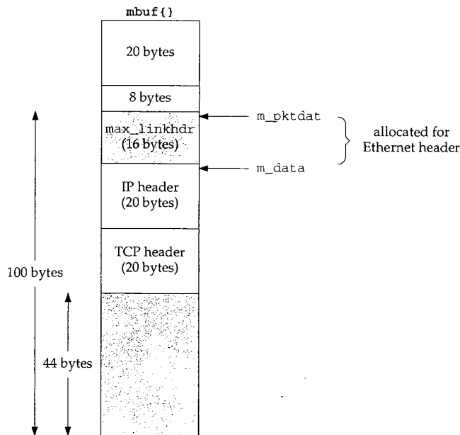
Figure 9.29 ip_insertoptions function: TCP segment.
