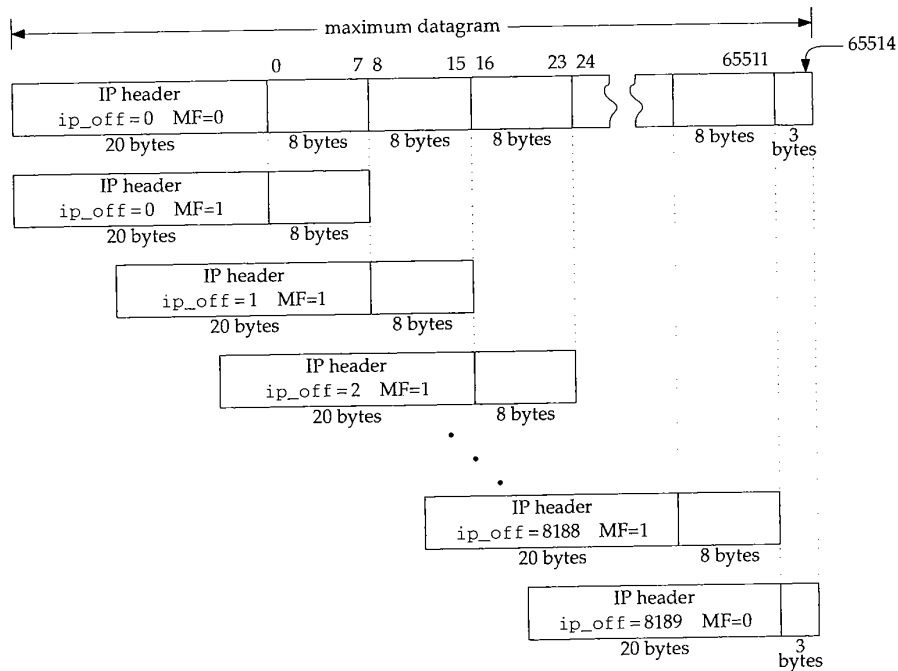
Figure 10.2 Fragmentation of a 65535-byte datagram.
