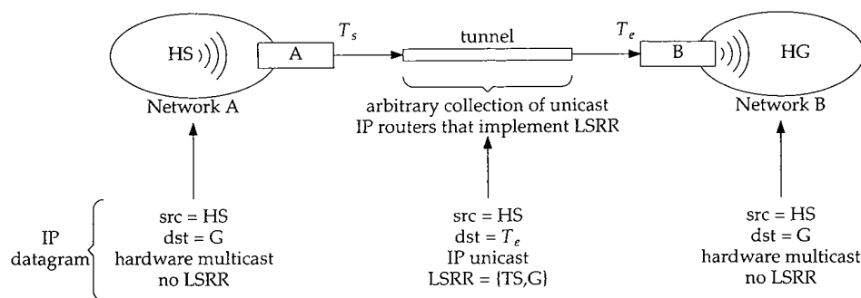
Figure 14.12 A multicast tunnel.
