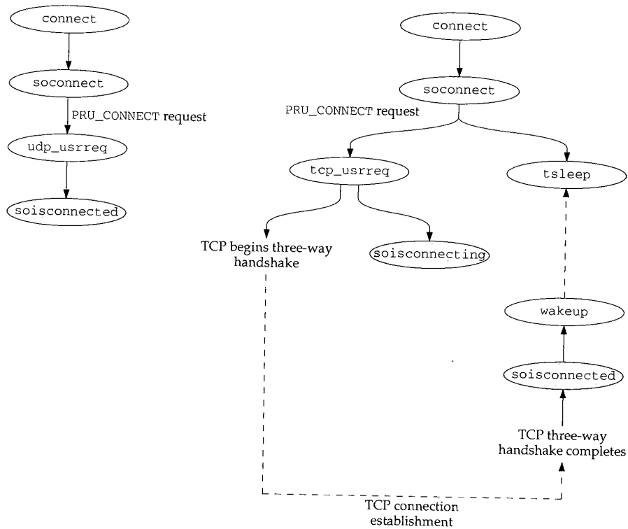
Figure 15.31 connect processing.
