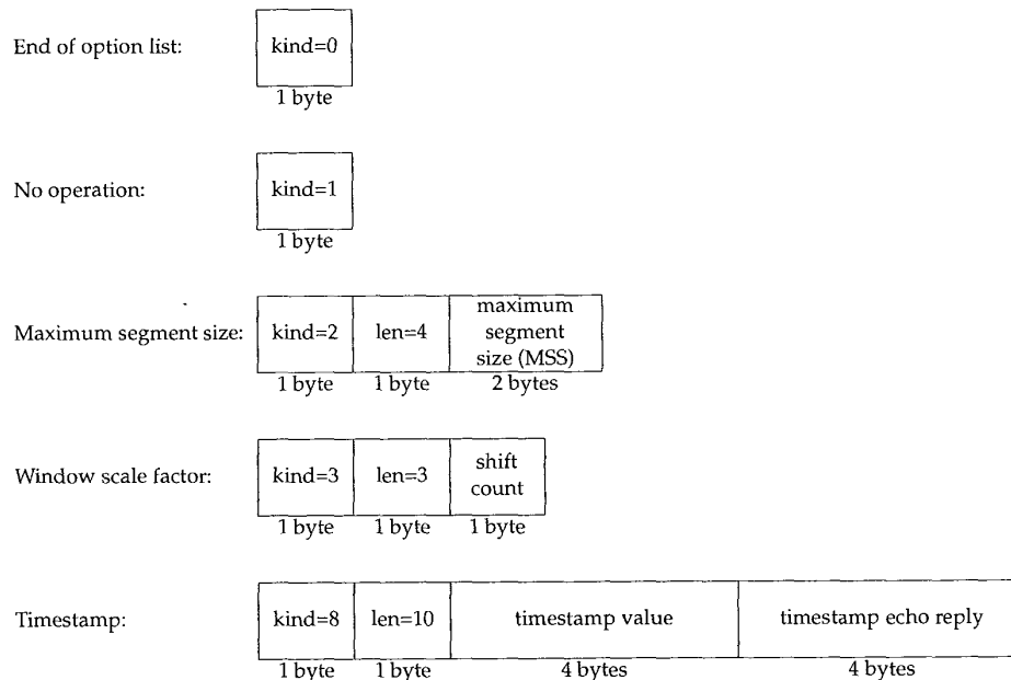
Figure 18.20 TCP options.
