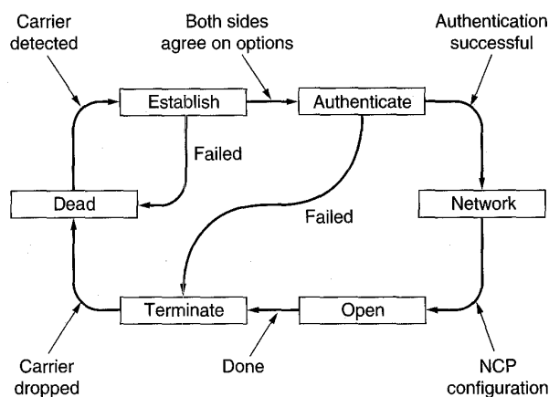
Fig. 3-28. A simplified phase diagram for bringing a line up and down.
