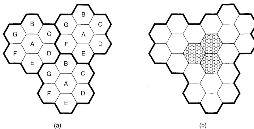
Fig. 2-54. (a) Frequencies are not reused in adjacent cells. (b) To add more users, smaller cells can be used.
