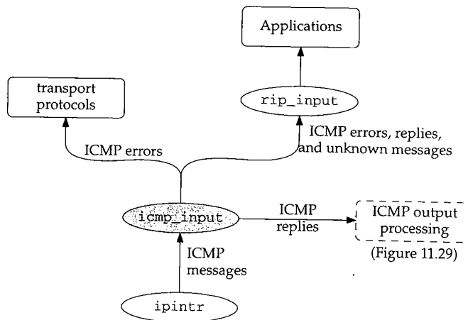
Figure 11.14 ICMP input processing.
