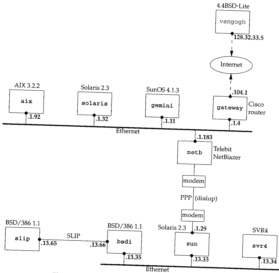
Figure 1.17 Test network used for all the examples in the text.
