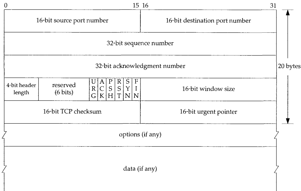
Figure 17.2 TCP header.
