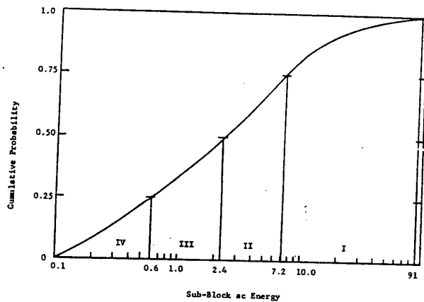
Figure 4. Probability distribution of sub-block ac energy.
