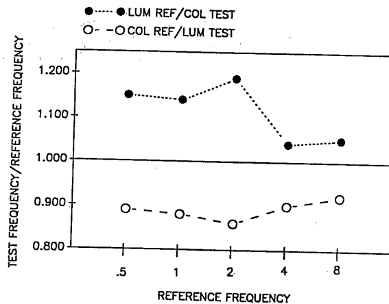
FIG. 4. Relationship of a reference spatial frequency which appears to match it perceptually, plotted as a function of the reference frequency. When the reference (standard) is a luminance grating and the test is an isoluminant chromatic grating (filled circles, dotted lines), the test must be set to a higher real frequency to produce a perceptual match. When the reference is a chromatic grating and the test is a luminance grating, the test must be set to a lower veridical frequency. Both reference and test gratings were set to equal multiples of their respective threshold contrasts.
