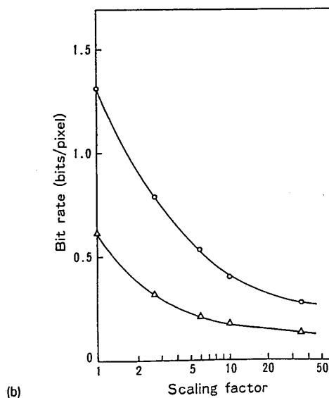
Fig. 4 (a) Relation of SNR versus scaling factor and (b) relation of bit rate versus scaling factor. Δ=continuous-tone image; ○=character image.
