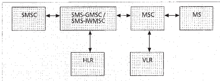
■ Figure 5. The SMS network architecture.
