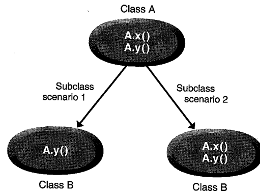
Figure 3.8 Method inheritance.
