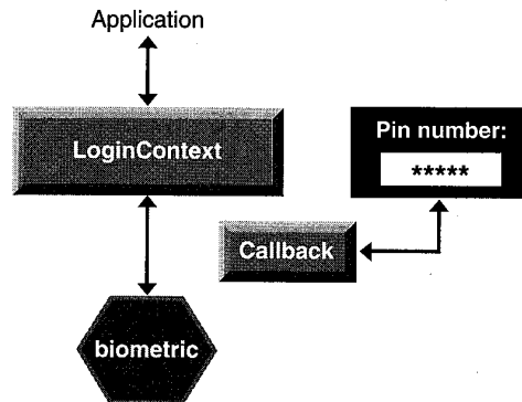
Figure 8.3 Callback design and usage.
