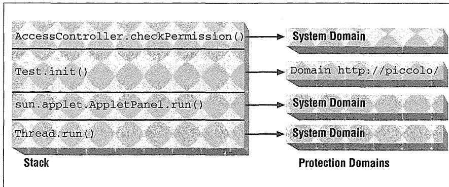
Figure 5-2. The stack and protection domains of a method
