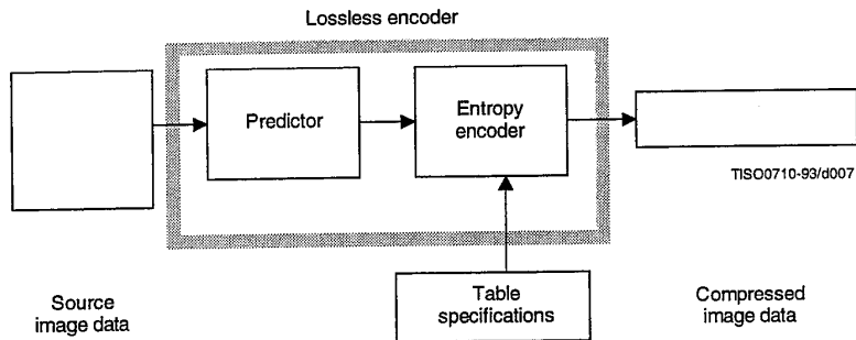
Figure 7 – Lossless encoder simplified diagram
