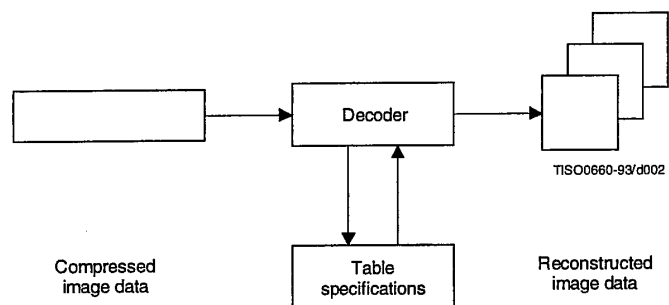
Figure 2 - Decoder
