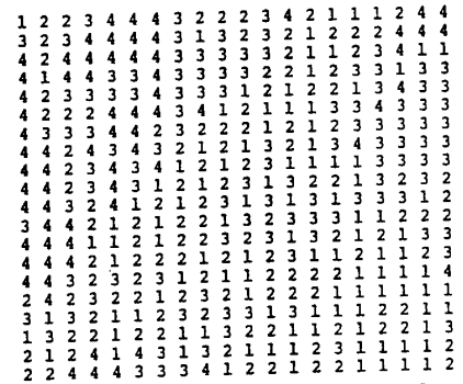
Figure 5. Classification of the central 20 x 20 transform sub-blocks for the monochrome image. 1 specifies the highest activity sub-blocks; 4 specifies the lowest activity sub-blocks.
