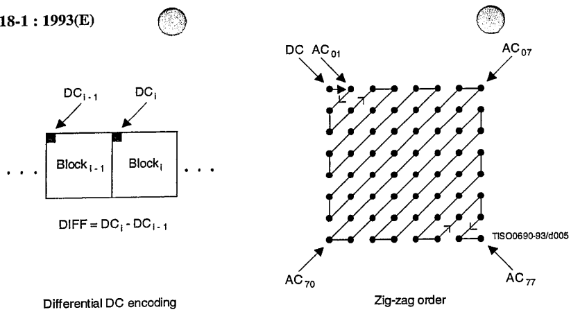
Figure 5 – Preparation of quantized coefficients for entropy encoding
