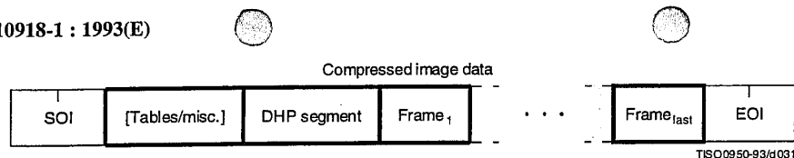
Figure B.13 – Syntax for the hierarchical mode of operation
