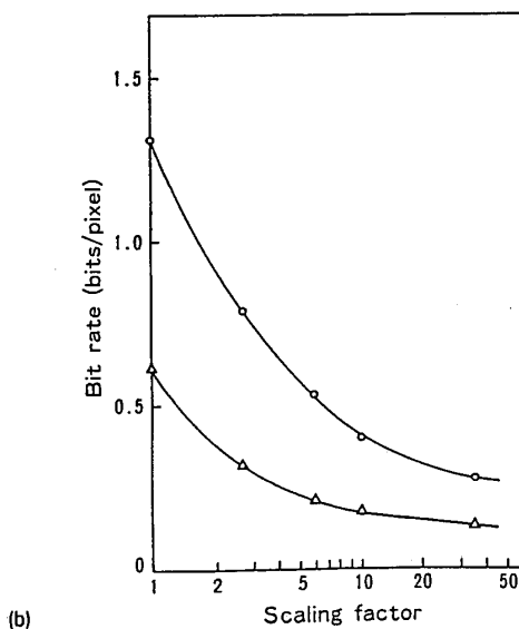
Fig. 4 (a) Relation of SNR versus scaling factor and (b) relation of bit rate versus scaling factor. \Delta =continuous-tone image; \circ =character image.
