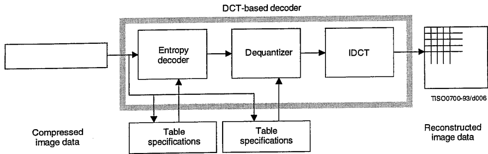
Figure 6 – DCT-based decoder simplified diagram
