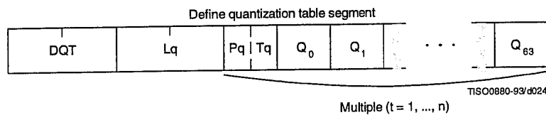
Figure B.6 – Quantization table syntax
