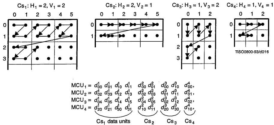
Figure A.3 – Interleaved data ordering example
