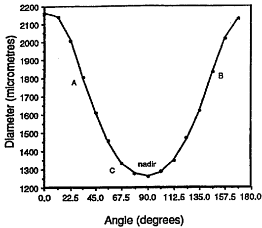
Figure 3a. Upper case O etched in chrome
