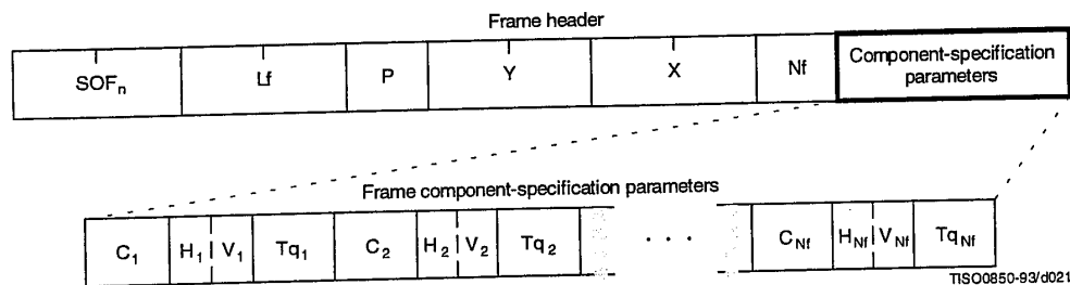
Figure B.3 – Frame header syntax
