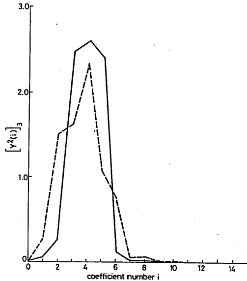
Fig. 7 Magnitude-squared spectral response over a window of length three corresponding to the results of Fig. 4
