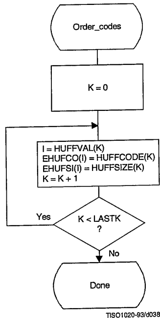
Figure C.3 – Ordering procedure for encoding procedure code tables
