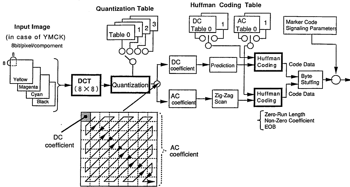
Fig. 1 Coding process by JPEG baseline system.
