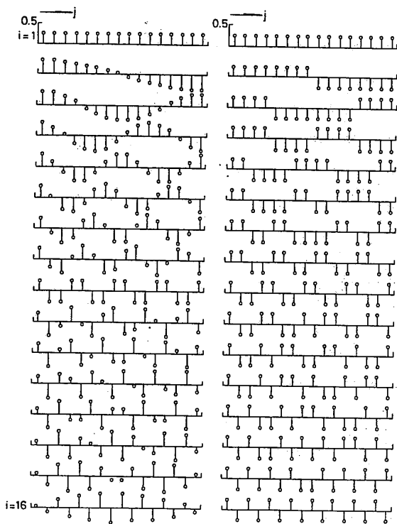
Fig. 2 Basis vectors of the 16-point DCT
