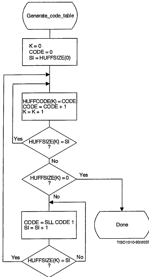
Figure C.2 – Generation of table of Huffman codes
