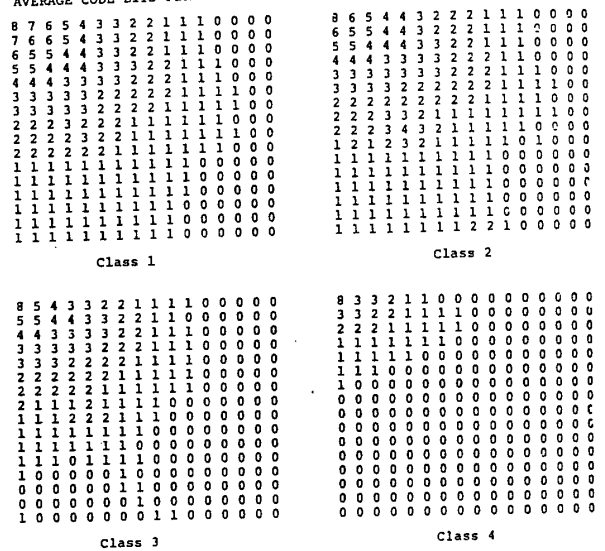
Figure 6. Bit allocation matrices for the monochrome image.
