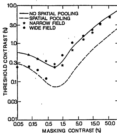
FIG. 6. Contrast discrimination: data and model. Contrast discrimination thresholds, for which both signal and masker are 2.0 cpd sine-wave gratings, have been replotted from Figs. 2 and 4 as a function of contrast. (●) wide field; (*) narrow field. The two curves are derived from the masking model. — prediction based on output of a single detector, no spatial pooling. --- model predictions include spatial pooling over 6°.
