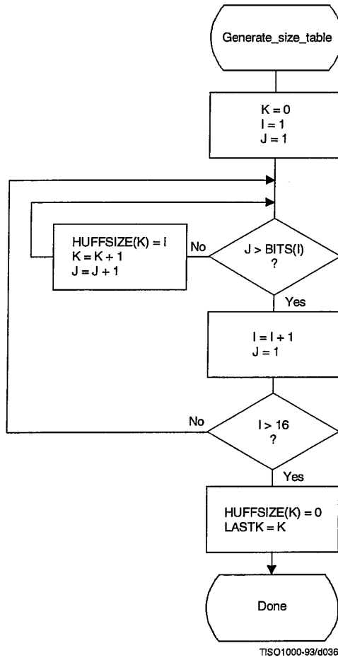
Figure C.1 – Generation of table of Huffman code sizes
