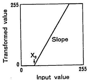
Fig. 7 Method of transformation characterized by x_0 (crossing point) and slope.
