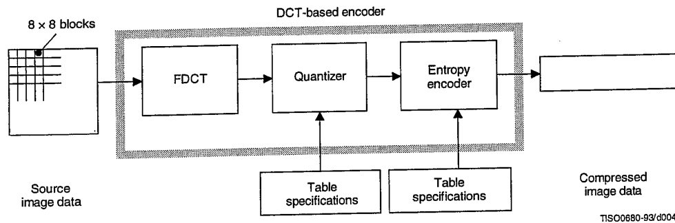
Figure 4 – DCT-based encoder simplified diagram
