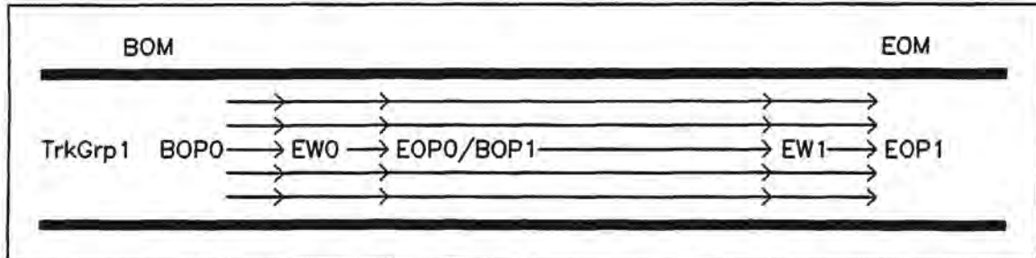
Figure 26 - Partitioning example - two partitions per track group
