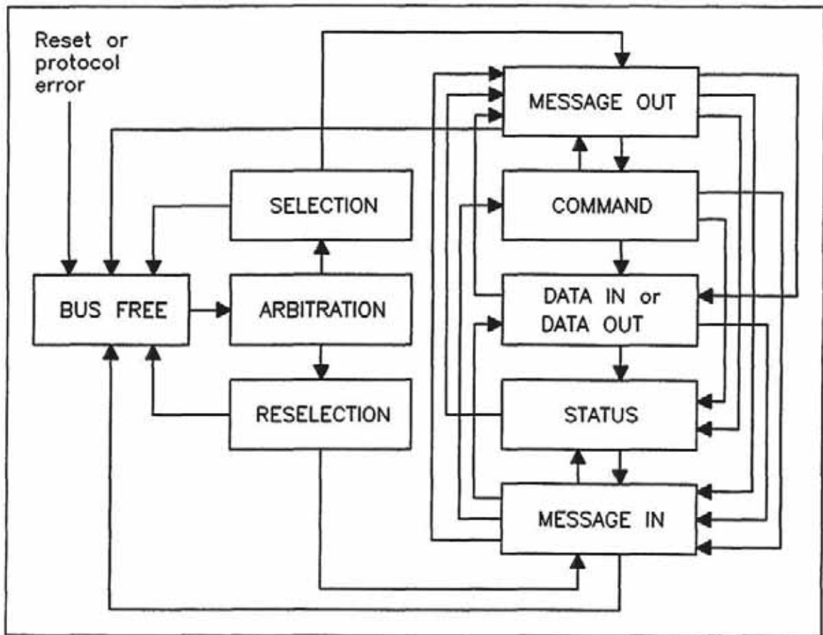
Figure 16 - Phase sequences
