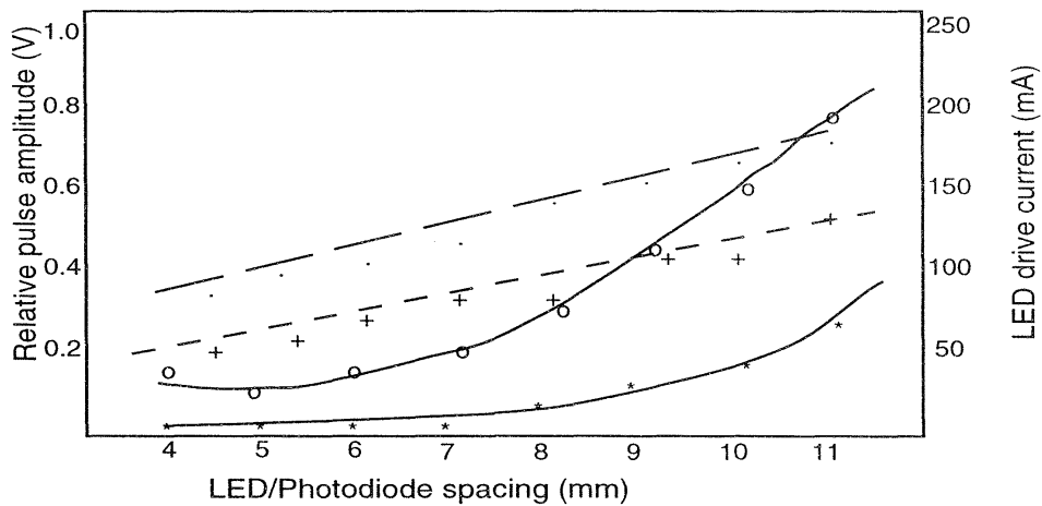
Figure 7.4 Effect of LED/photodiode separation on the relative pulse amplitude of the red (+) and infrared (·) plethysmograms. The driving currents of the red (o) and infrared (*) LEDs required to maintain a constant DC reflectance from the skin are shown for comparison (adapted from Mendelson and Ochs 1988).
