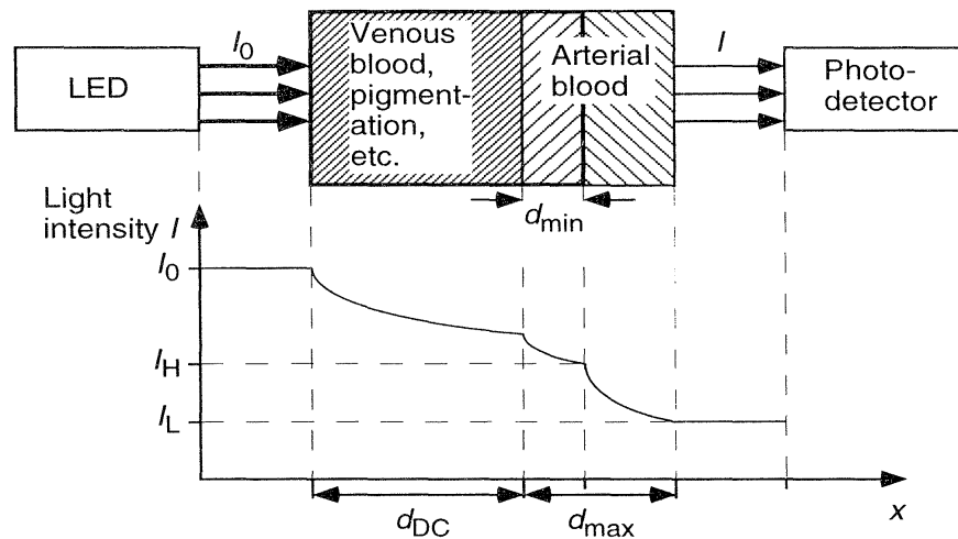
Figure 4.5 Beer's law in pulse oximetry. The DC components of the tissue (e.g. skin pigmentation, bone, venous blood and the nonpulsating part of the arterial blood) absorb a constant amount of the incident light I_0 . The effective optical path length in the DC components without the constant level of arterial blood is represented by d_{DC} . During diastole the optical path length through the arteries has a minimum length of d_{min} and the light intensity at the photodetector is maximal ( I_H ). The optical path length reaches a maximum d_{max} during systole and the hemoglobin in the arteries absorbs a maximum amount, causing I to decrease to a minimum level of I_L .
