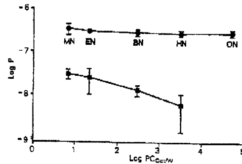
FIG. 1. Relationship between permeability coefficient P and partition coefficient octanol/water PC_{O/W} of the nicotinic acid esters across human nail plate (■) and bovine hoof membrane (●) at 32°C ( n = 3-8 , mean \pm s.d.). MN = methyl nicotinate, EN = ethyl nicotinate, BN = butyl nicotinate, HN = hexyl nicotinate, ON = octyl nicotinate. P in \text{cm}^2 \text{s}^{-1} .
